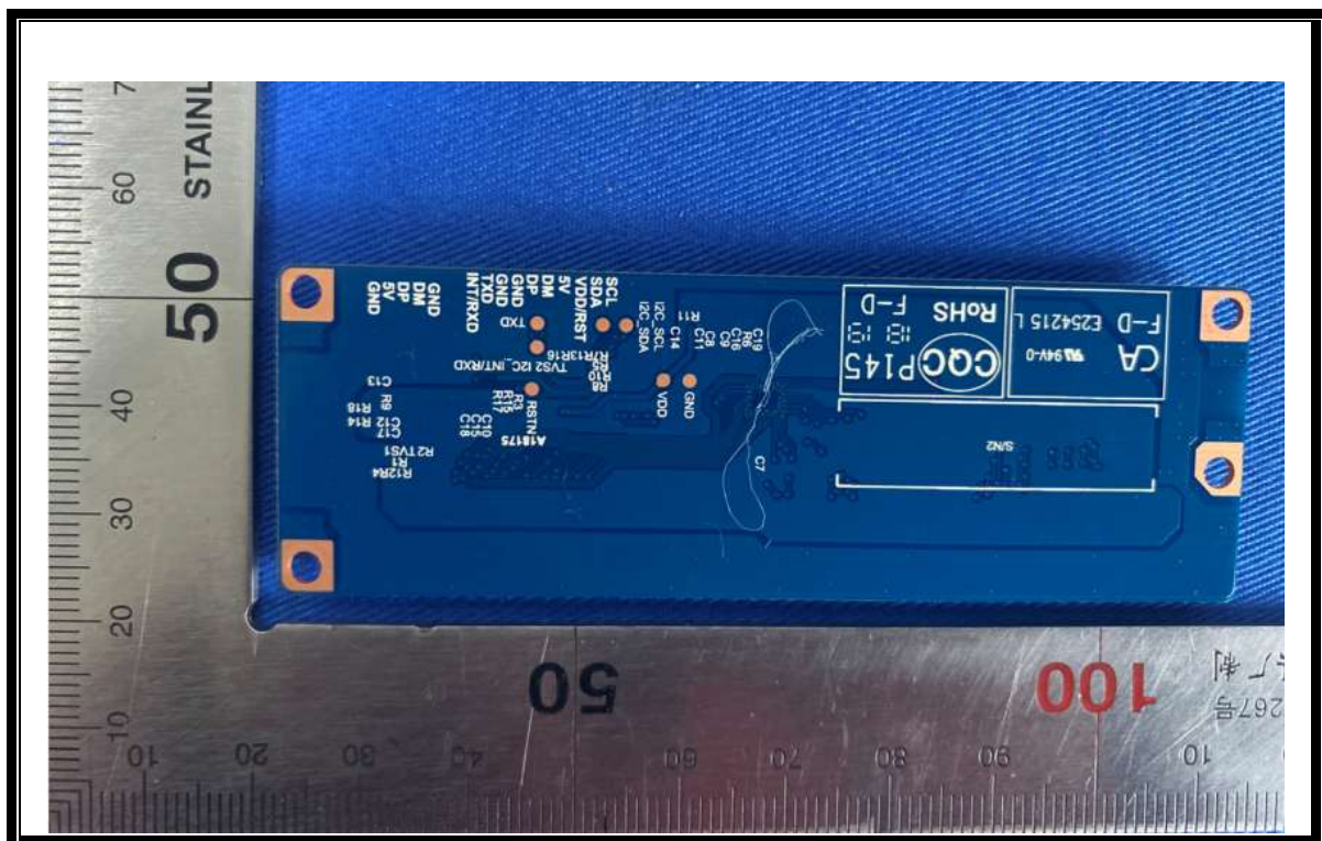
Internal view - Control board Bottom
