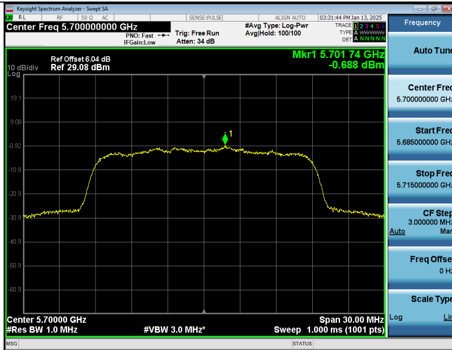
Power_Spectral_Density_NVNT_ANT2_802_11n(HT20)_5700
