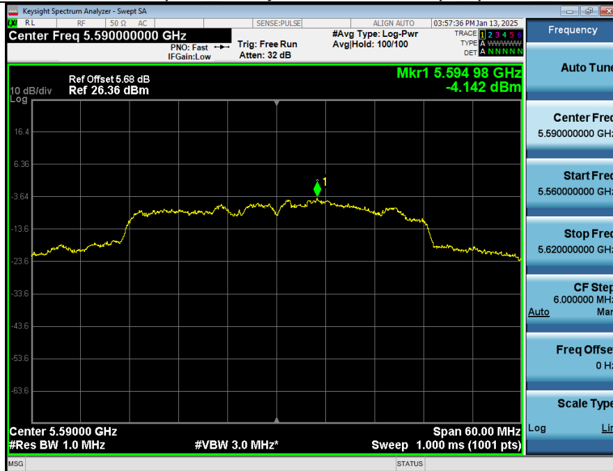
Power_Spectral_Density_NVNT_ANT2_802_11n(HT40)_5590
