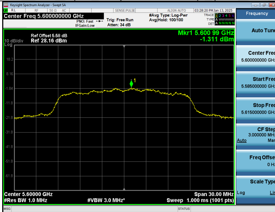
Power_Spectral_Density_NVNT_ANT2_802_11n(HT20)_5600
