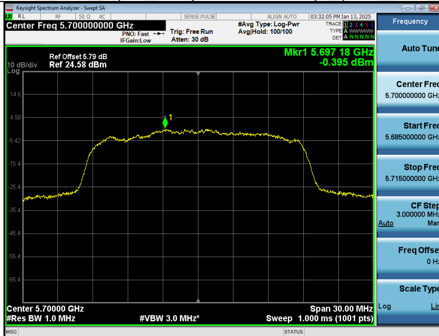
Power_Spectral_Density_NVNT_ANT2_802_11n(HT20)_5700
