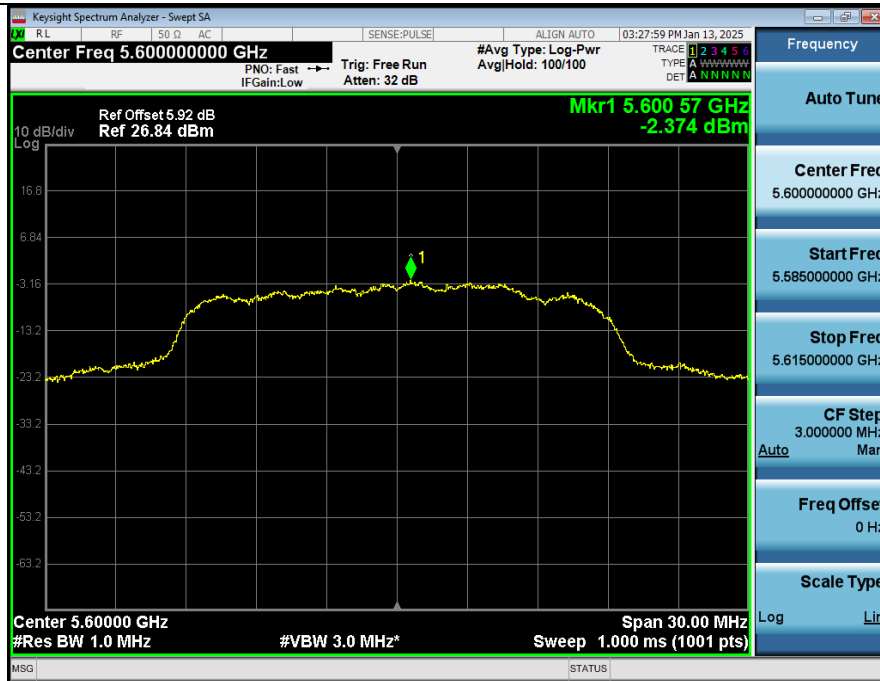
Power_Spectral_Density_NVNT_ANT2_802_11n(HT20)_5600
