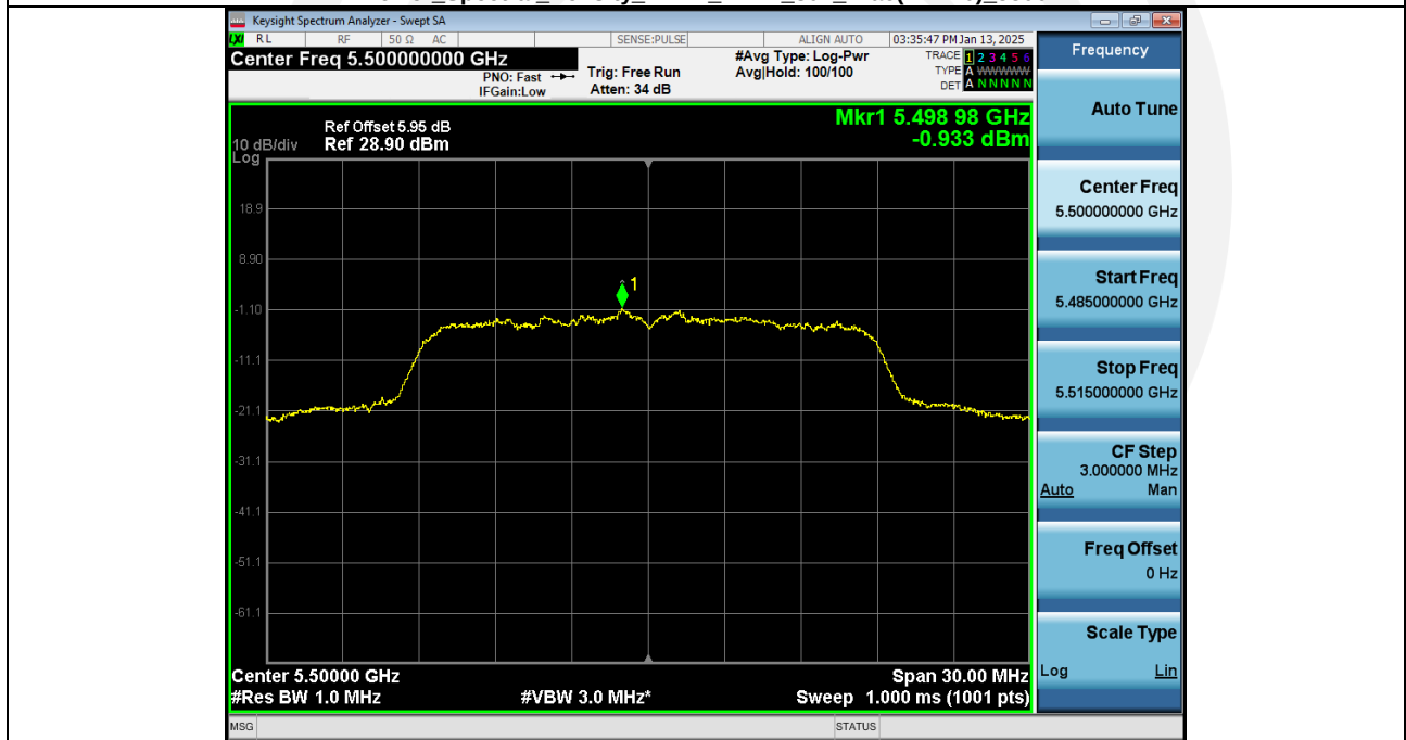
Power_Spectral_Density_NVNT_ANT2_802_11ac(VHT20)_5500
