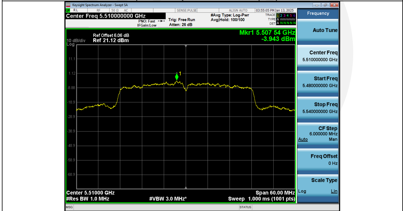
Power_Spectral_Density_NVNT_ANT2_802_11n(HT40)_5510
