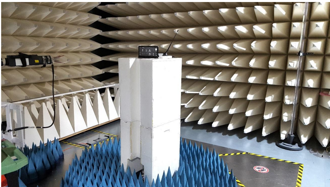
Figure B7. Radiated emission Setup 3
