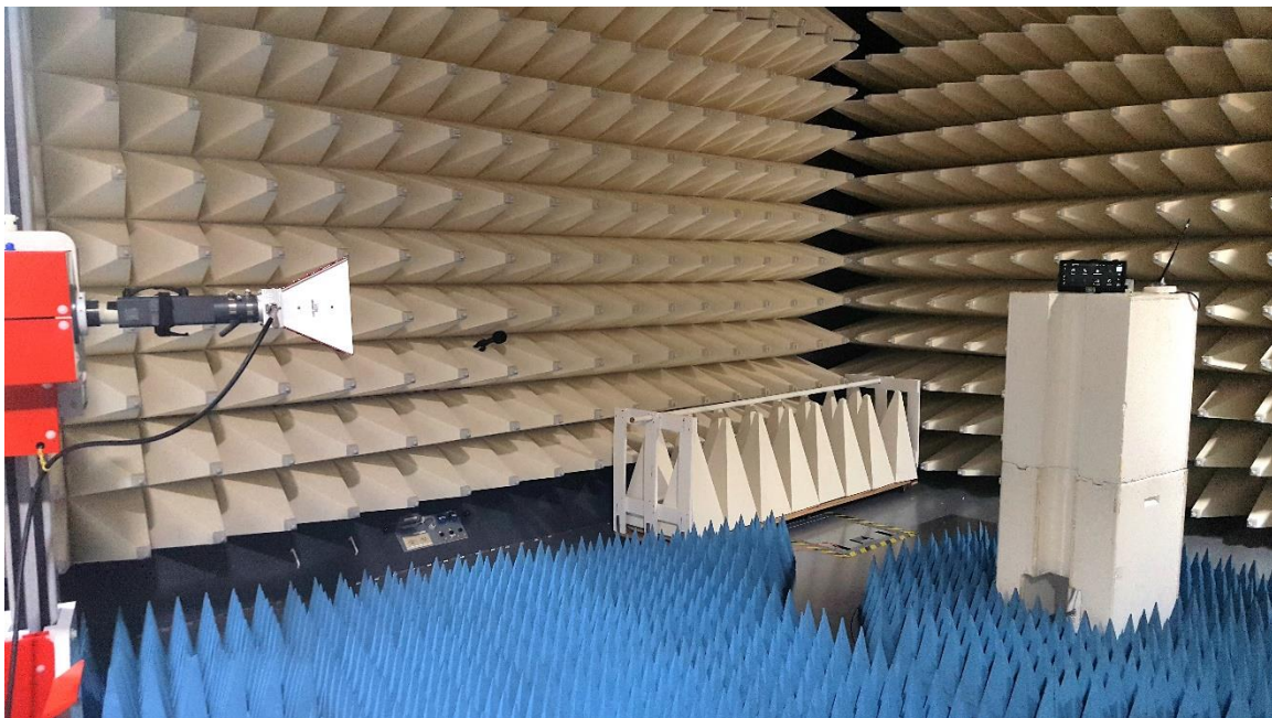
Figure B6. Radiated emission Setup 2
