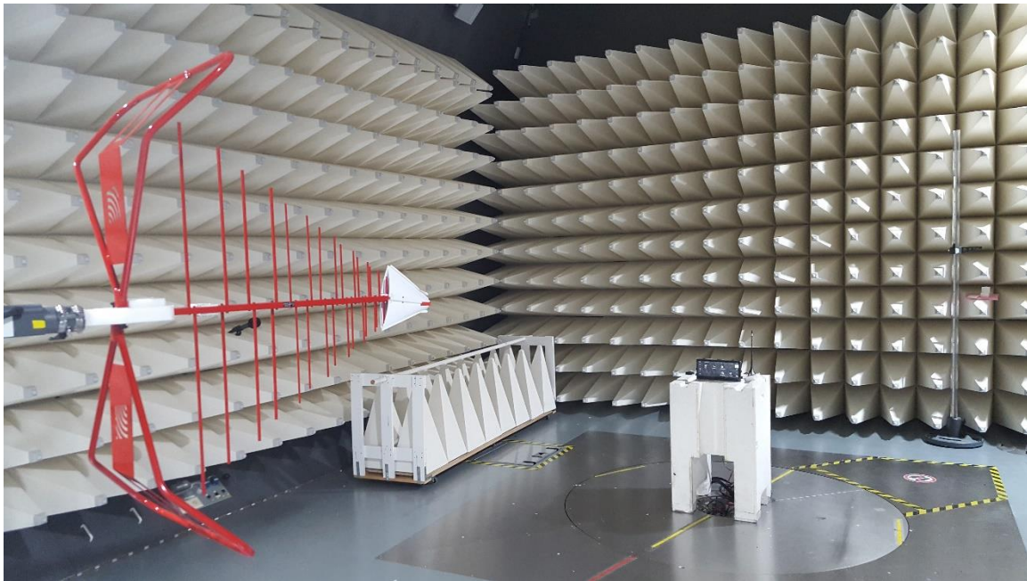
Figure B5. Radiated emission Setup 1
