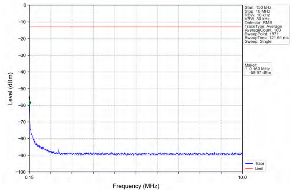
Band25_20MHz_QPSK_MCH_1882.5MHz_RB_1_0_NTNV
