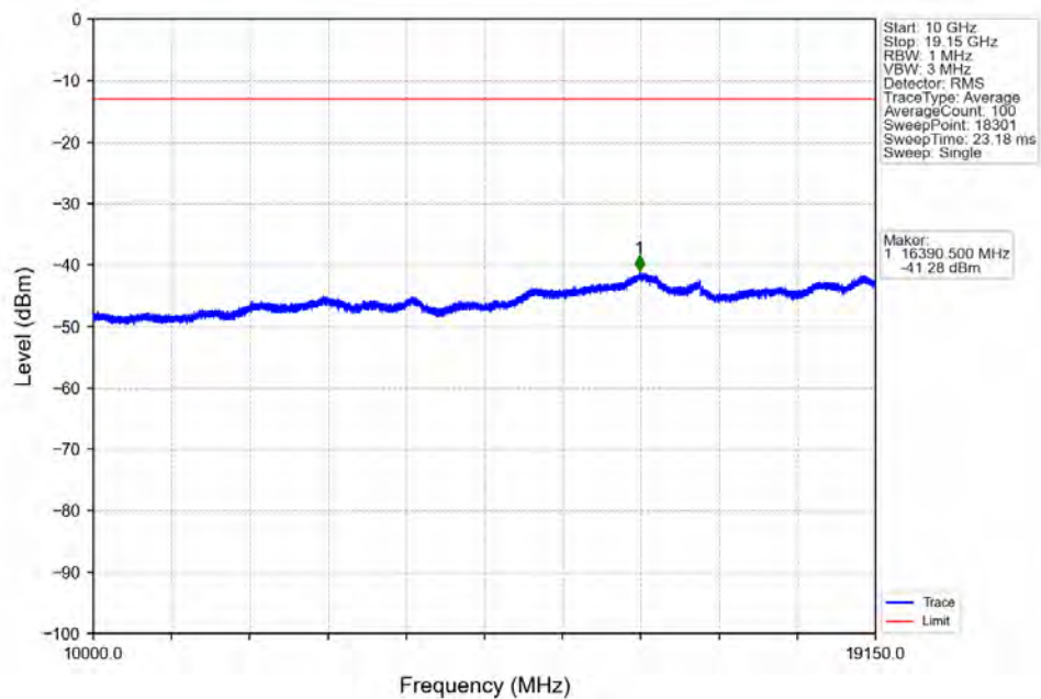
Band25_5MHz_QPSK_MCH_1882.5MHz_RB_1_0_NTV
