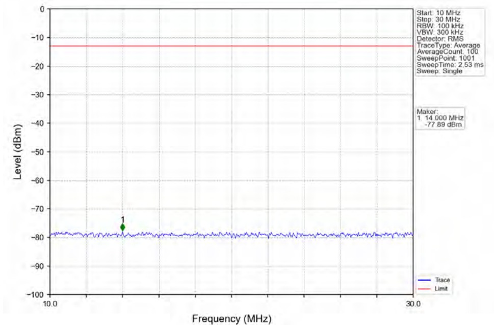
Band25_10MHz_QPSK_MCH_1882.5MHz_RB_1_0_NTNV
