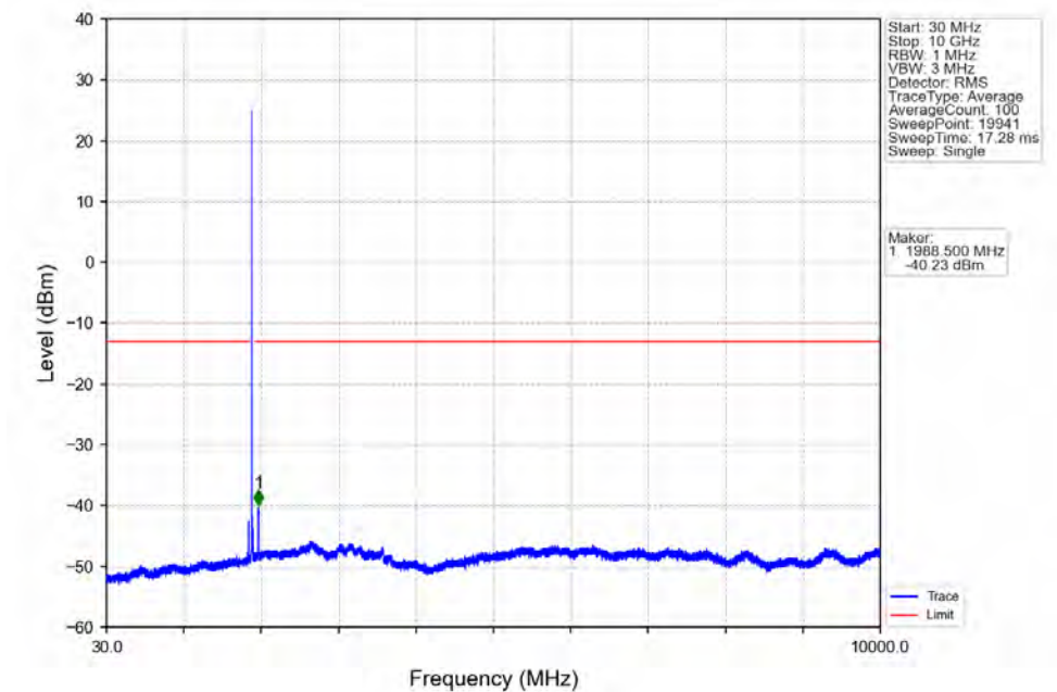
Band25_15MHz_QPSK_HCH_1907.5MHz_RB_1_0_NTNV
