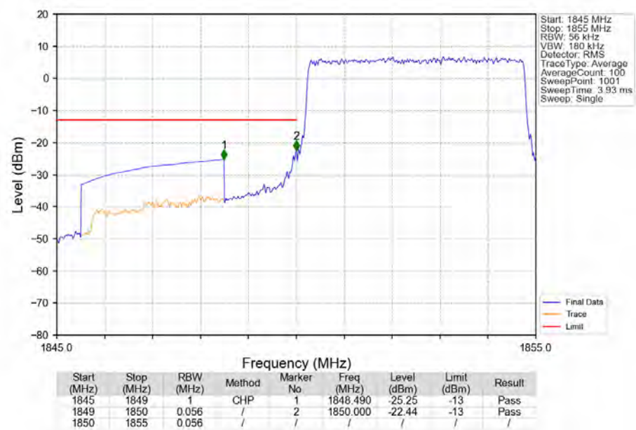
Band25_5MHz_QPSK_LCH_1852.5MHz_RB_25_0_NTNV
