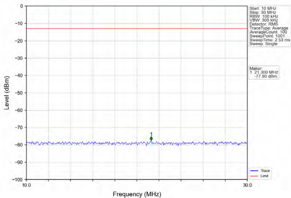
Band25_15MHz_QPSK_LCH_1857.5MHz_RB_1_0_NTNV
