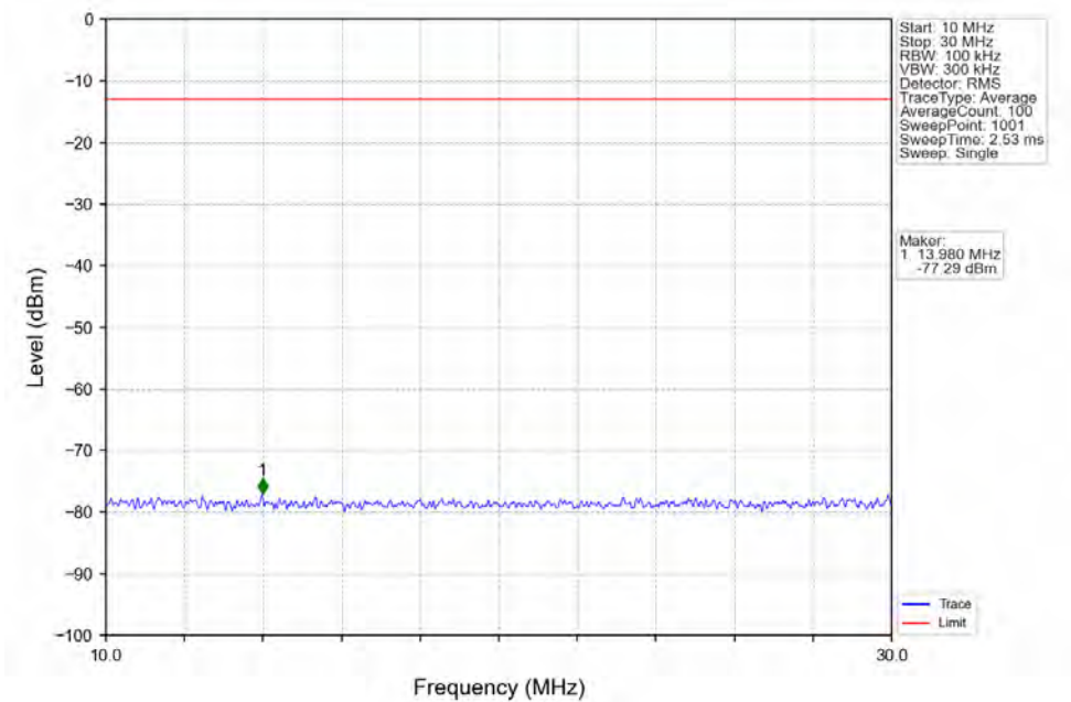
Band25_5MHz_QPSK_HCH_1912.5MHz_RB_1_0_NTV
