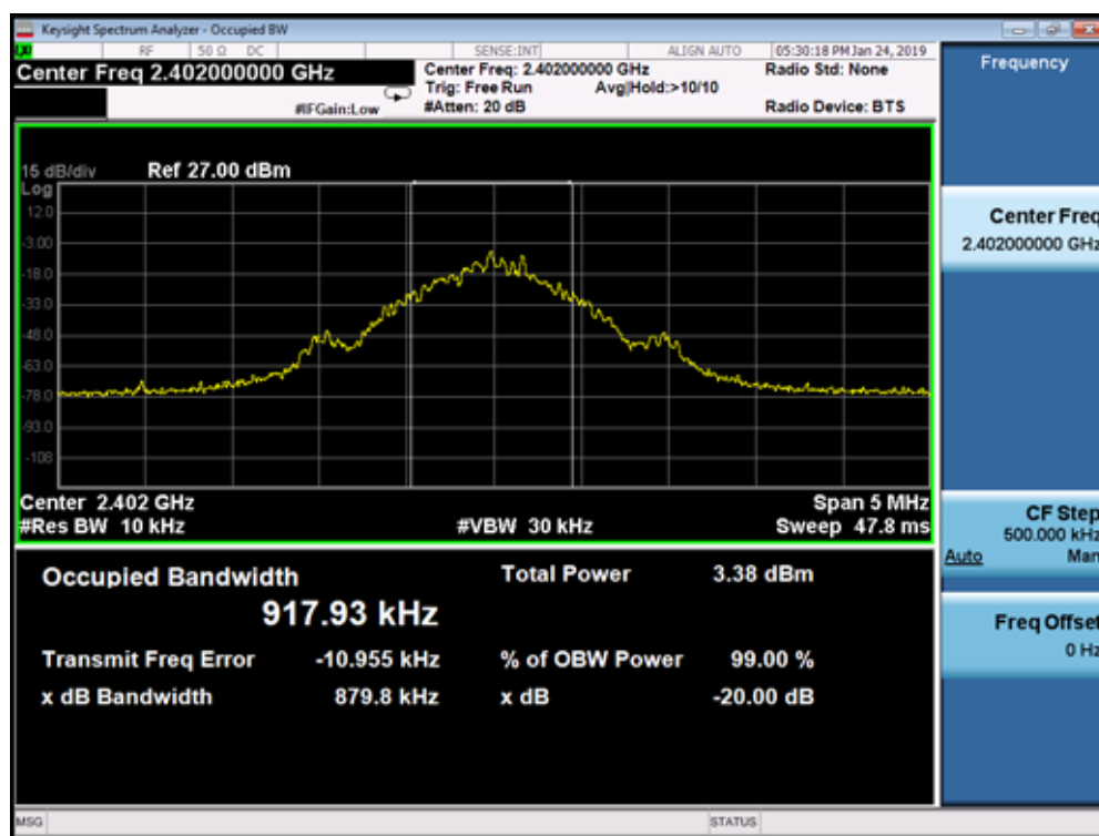
Channel 00 (2402MHz)
