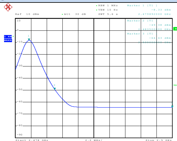
Channel 78 / 2480 MHz –Peak
