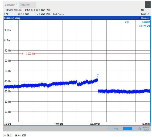
Band5-3MHz-QPSK-20635-1RB#14-3000~10000-PASS
