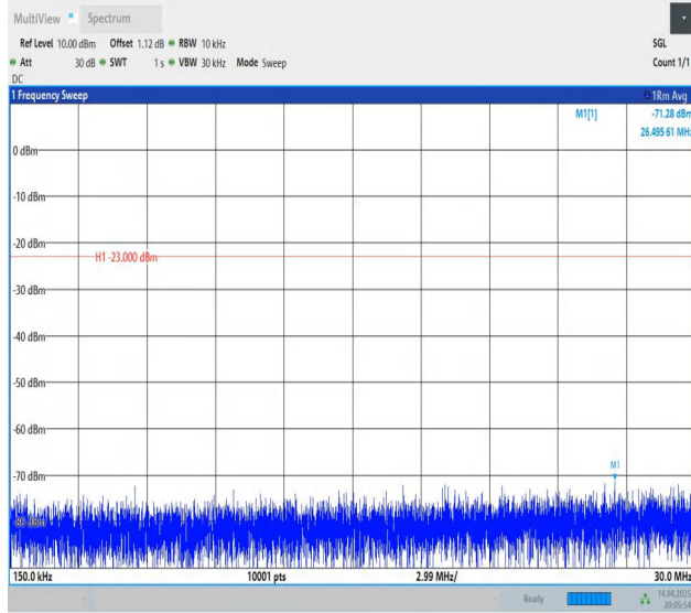
Band5-5MHz-QPSK-20525-1RB#24-0.15~30-PASS
