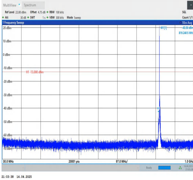
Band5-3MHz-QPSK-20415-1RB#0-30~1000-PASS
