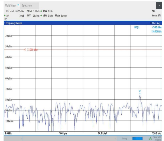
Band5-3MHz-QPSK-20635-1RB#14-0.009~0.15-PASS
