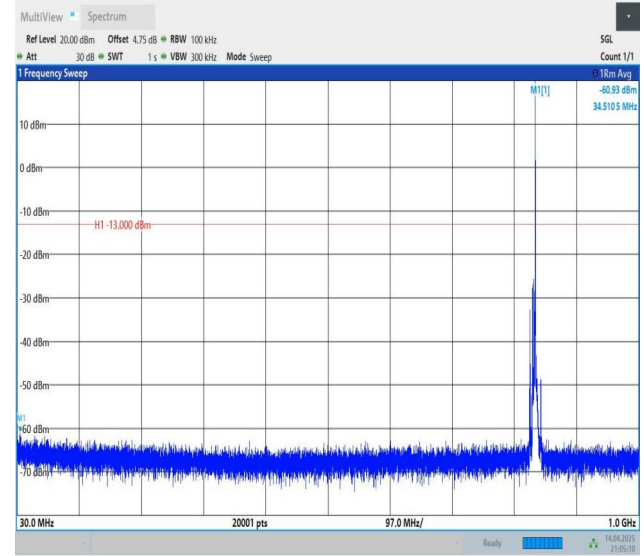
Band5-5MHz-QPSK-20525-1RB#24-30~1000-PASS
