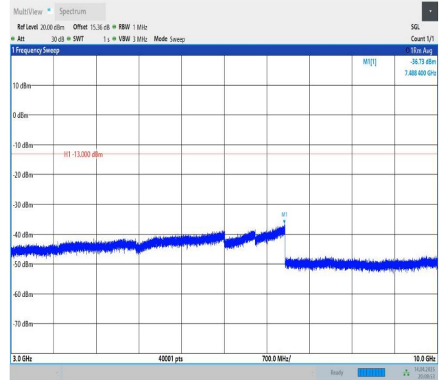
Band5-10MHz-QPSK-20525-1RB#49-3000~10000-PASS
