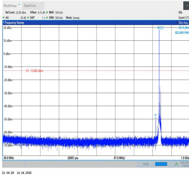
Band5-10MHz-QPSK-20600-1RB#0-30~1000-PASS
