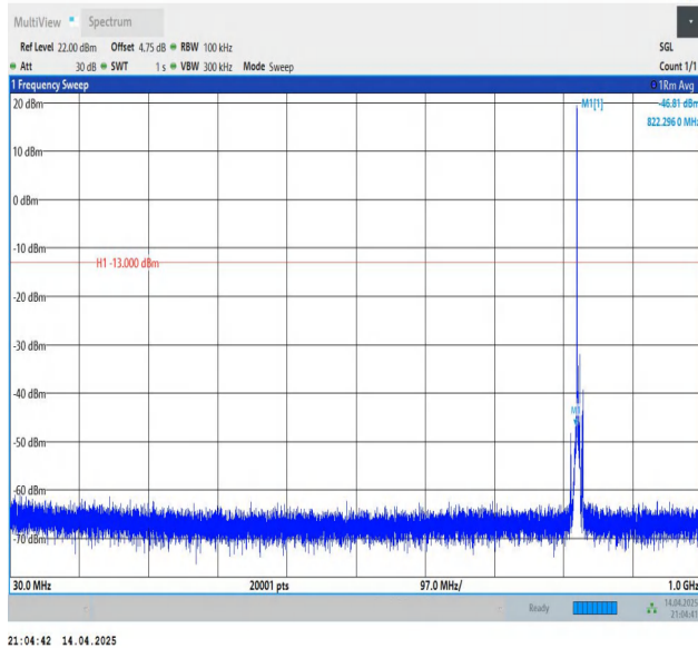
Band5-5MHz-QPSK-20425-1RB#0-30~1000-PASS
