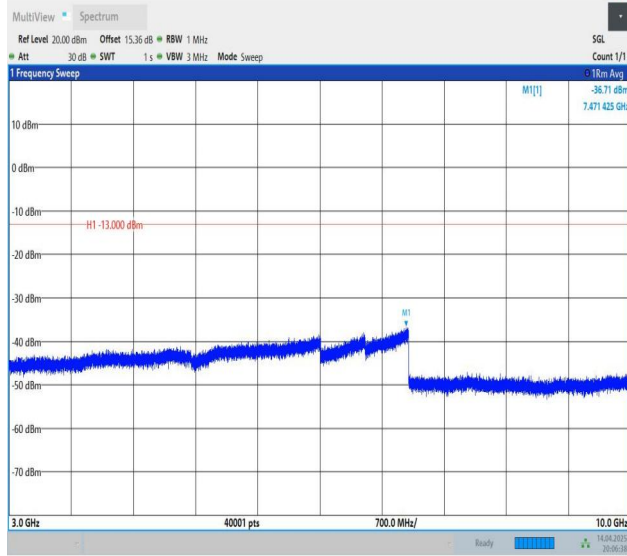
Band5-5MHz-QPSK-20625-1RB#0-3000~10000-PASS
