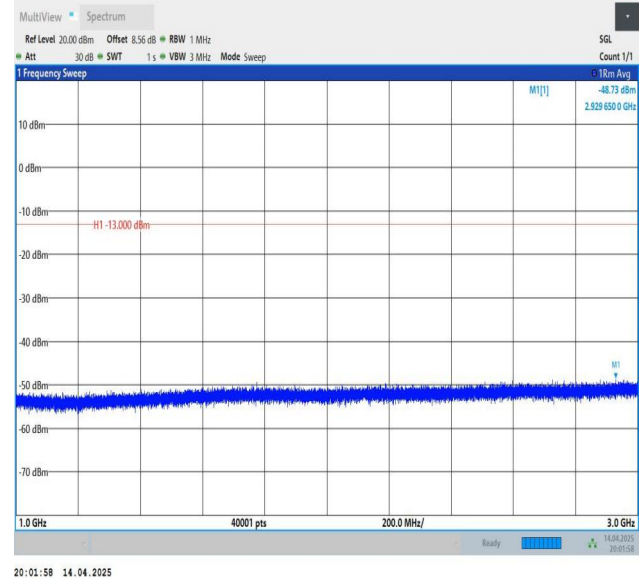
Band5-3MHz-QPSK-20415-1RB#0-1000~3000-PASS
