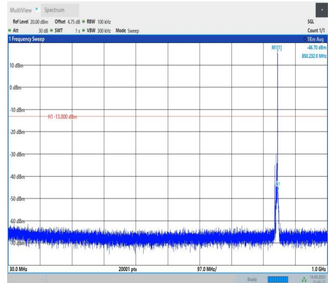
Band5-5MHz-QPSK-20625-1RB#24-30~1000-PASS
