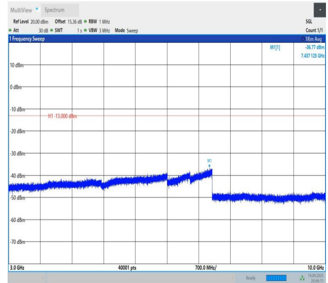
Band5-5MHz-QPSK-20525-1RB#24-3000~10000-PASS
