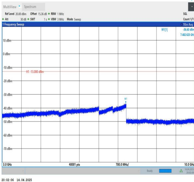
Band5-3MHz-QPSK-20415-1RB#0-3000~10000-PASS
