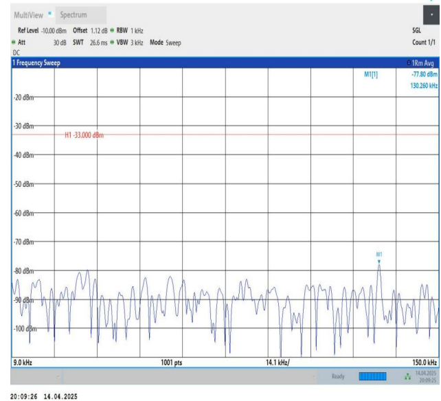
Band5-10MHz-QPSK-20600-1RB#49.0.009~0.15-PASS
