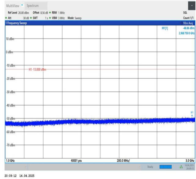
Band5-10MHz-QPSK-20600-1RB#0-1000~3000-PASS
