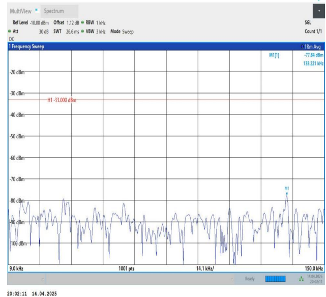
Band5-3MHz-QPSK-20415-1RB#14-0.009~0.15-PASS
