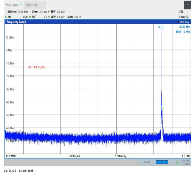
Band5-3MHz-QPSK-20635-1RB#14-30~1000-PASS
