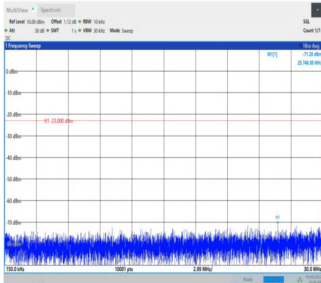
Band5-5MHz-QPSK-20625-1RB#24-0.15~30-PASS
