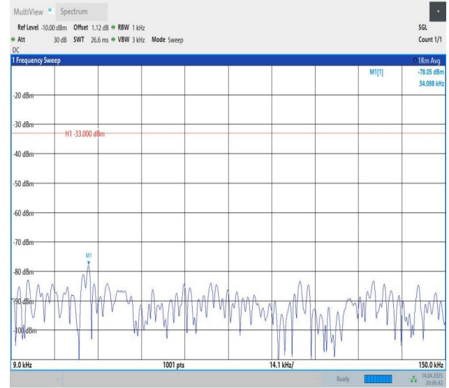
Band5-5MHz-QPSK-20625-1RB#24-0.009~0.15-PASS
