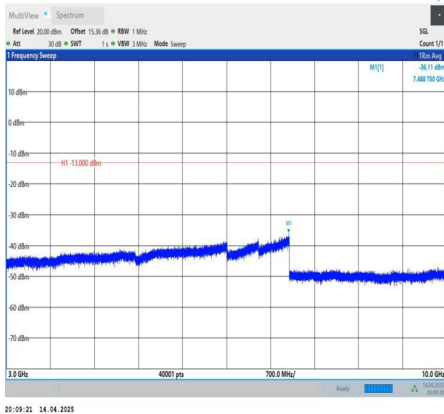
Band5-10MHz-QPSK-20600-1RB#0-3000~10000-PASS
