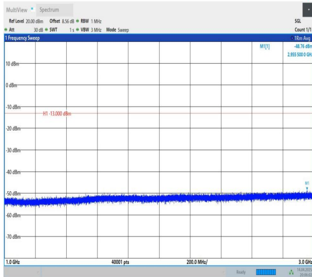
Band5-5MHz-QPSK-20525-1RB#24-1000~3000-PASS
