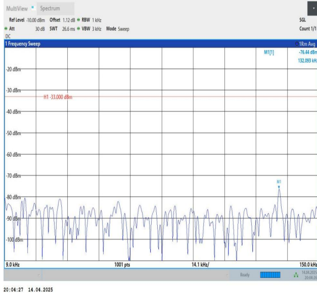
Band5-5MHz-QPSK-20425-1RB#0-0.009~0.15-PASS
