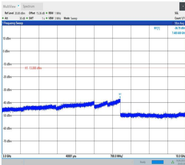
Band5-3MHz-QPSK-20635-1RB#0-3000~10000-PASS
