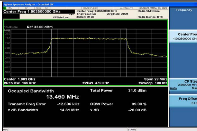
Band2-15MHz-QPSK-19125-75RB#0-13.450
