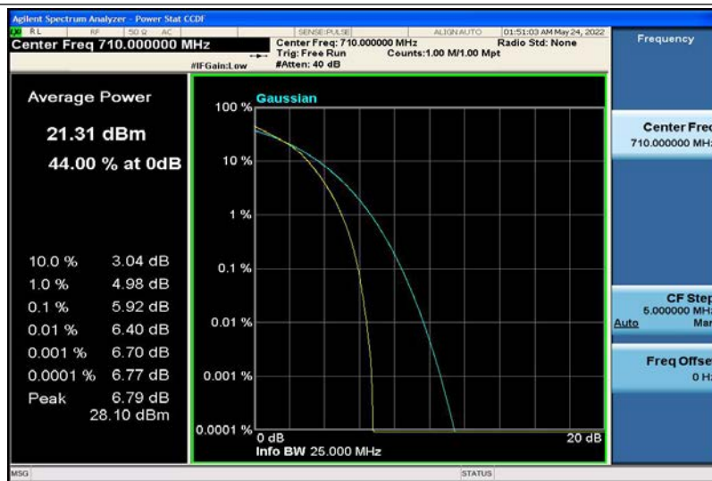
Band17-10MHz-16QAM-23790-50RB#0
