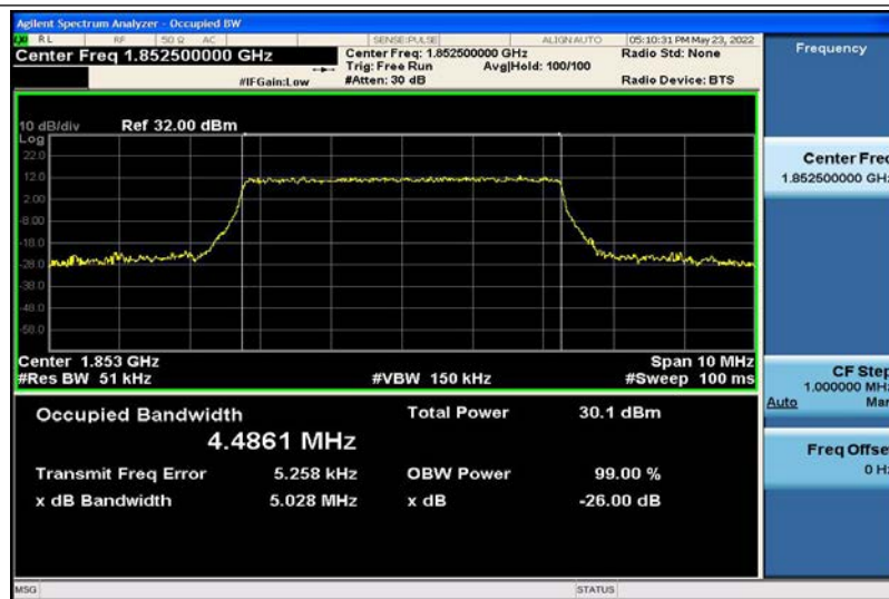
Band2-5MHz-16QAM-18625-25RB#0-4.4861
