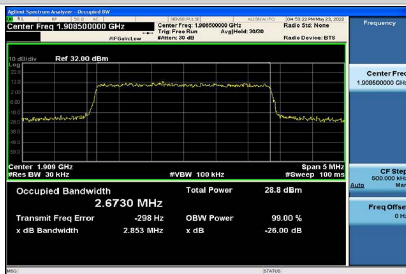
Band2-3MHz-16QAM-19185-15RB#0-2.6730
