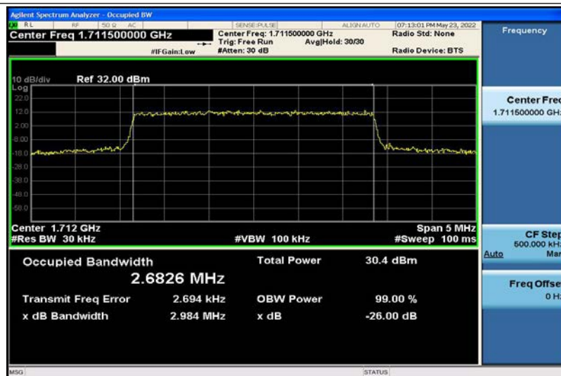
Band4-3MHz-QPSK-19965-15RB#0-2.6826
