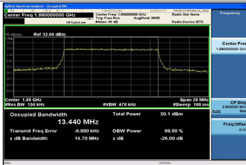
Band2-15MHz-16QAM-18900-75RB#0-13.440
