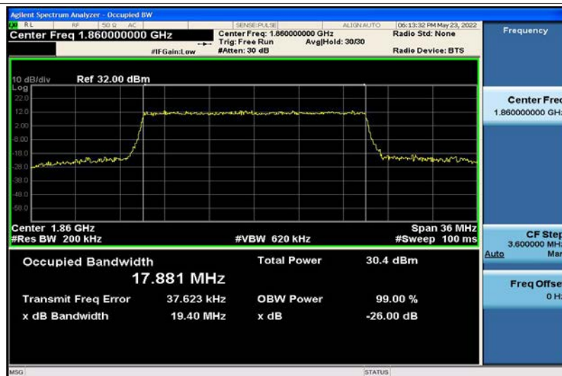
Band2-20MHz-16QAM-18700-100RB#0-17.881
