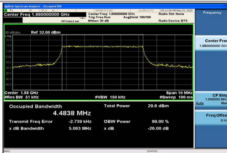
Band2-5MHz-16QAM-18900-25RB#0-4.4838
