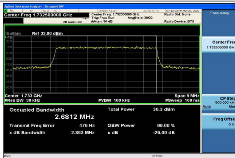
Band4-3MHz-QPSK-20175-15RB#0-2.6812
