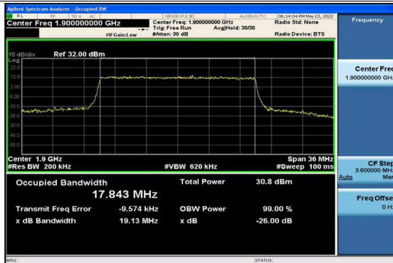
Band2-20MHz-QPSK-19100-100RB#0-17.843
