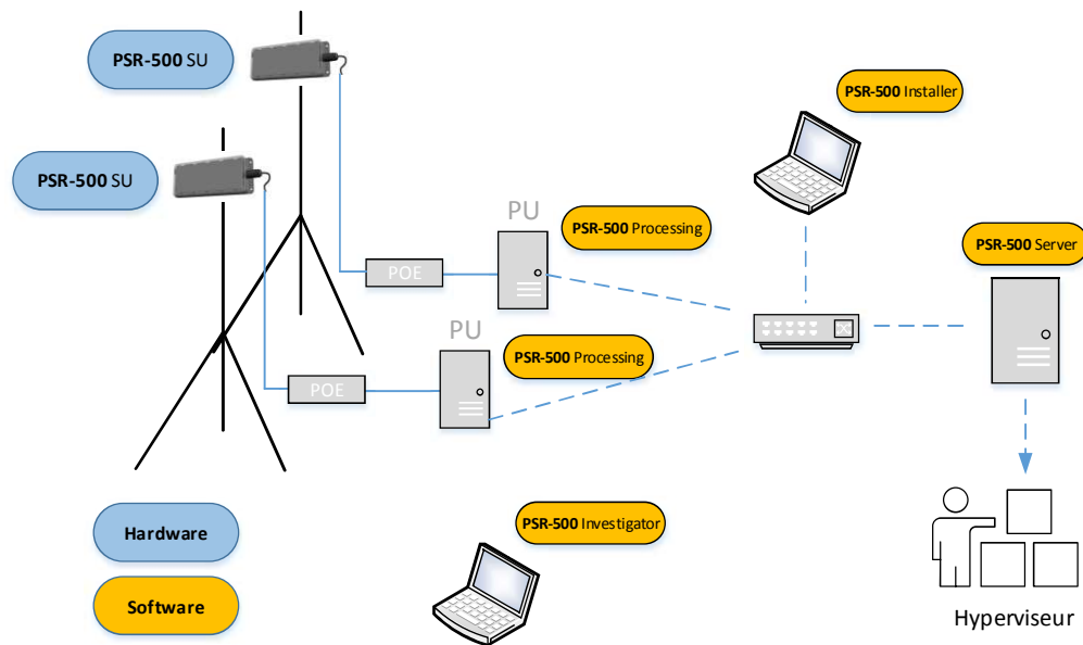
Figure 5: Integrated System architecture for PSR-500 System (two radars configuration)
