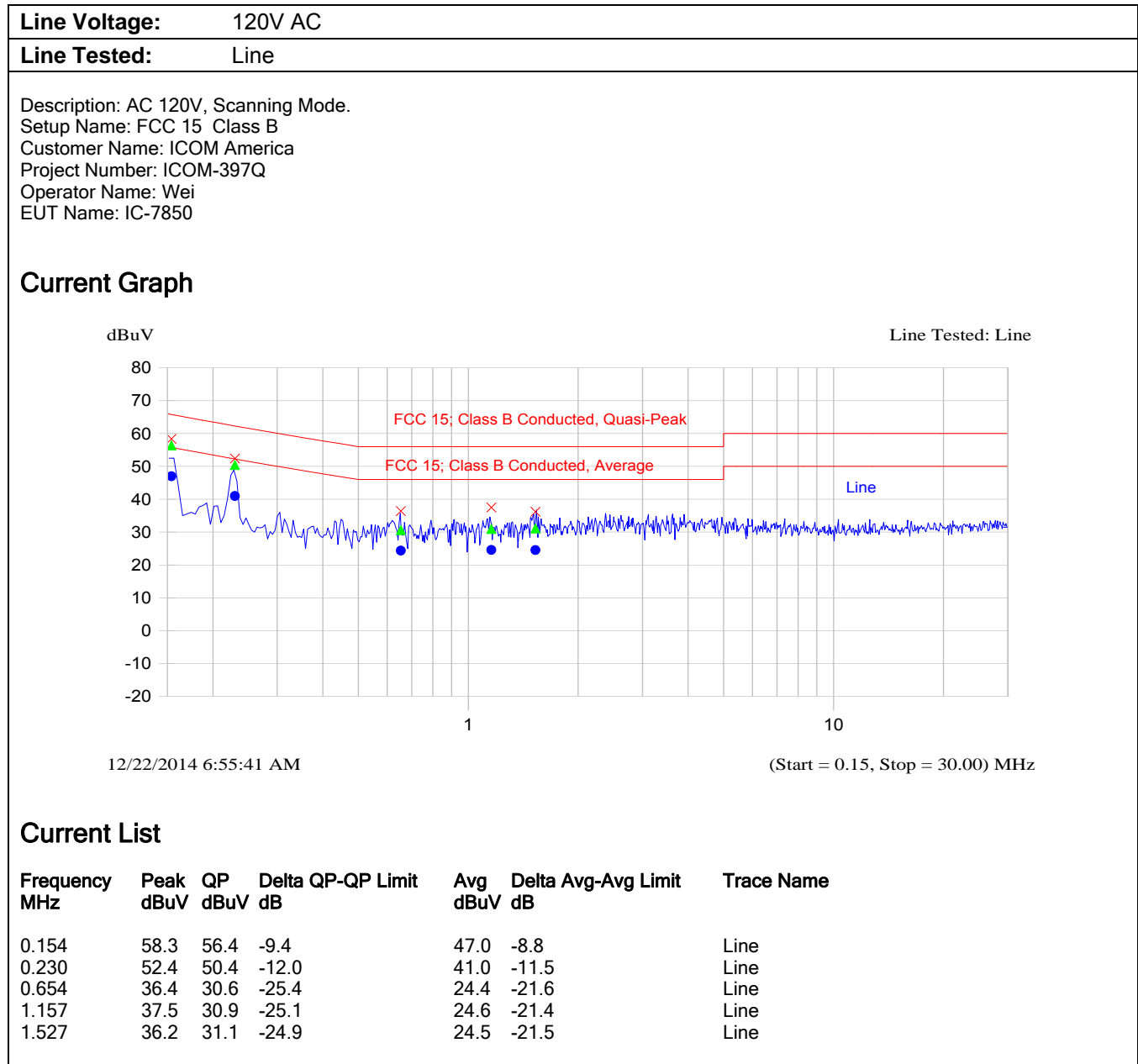
Plot 1: Power Line Conducted Emissions
