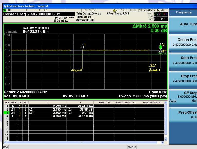
Duty_Cycle_NVNT_ANT1_1Mbps_2402
