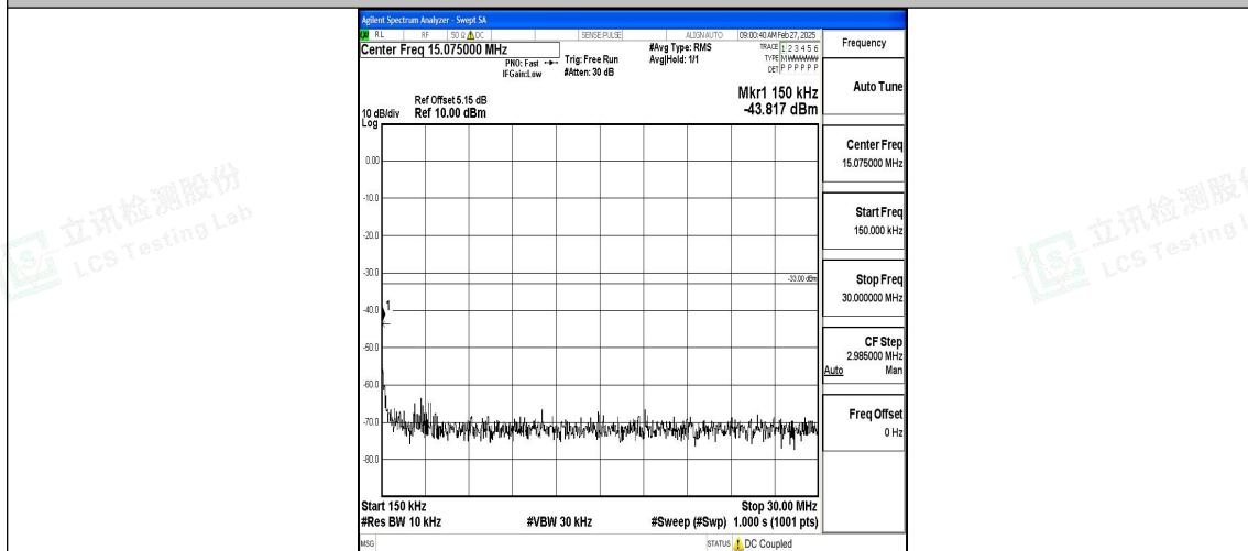
Band2_20MHz_16QAM_18700_1RB#0_0.15~30_0.15~30
