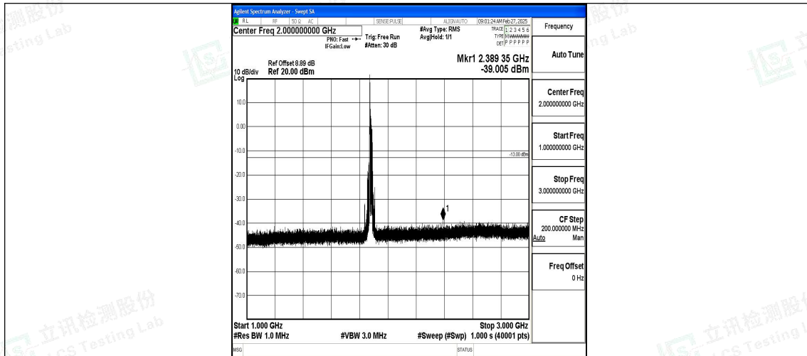
Band2_20MHz_QPSK_18900_1RB#0_1000~3000_1000~3000
