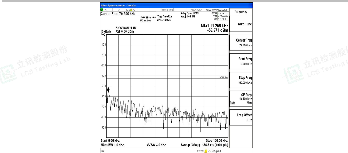
Band2_20MHz_16QAM_18900_1RB#0_0.009~0.15_0.009~0.15
