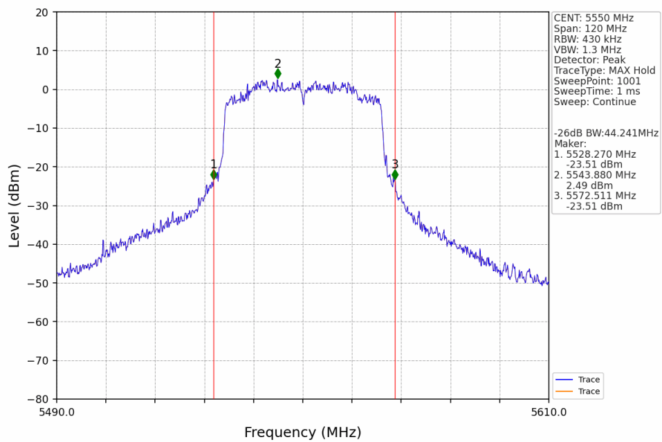
802.11ax(HEW40)_MCH_5550MHz_SU_ / Ant1_NTNV
