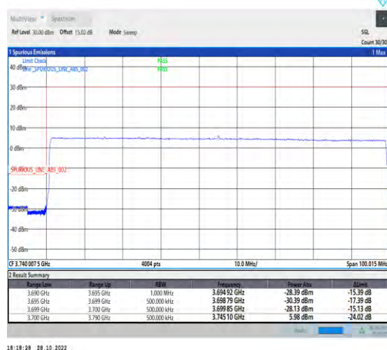
1-N77-3700-3980-PC2-30-90-L-6-CP-QPSK-Outer_Full-245@0-Ant1-1--PASS-see graph
