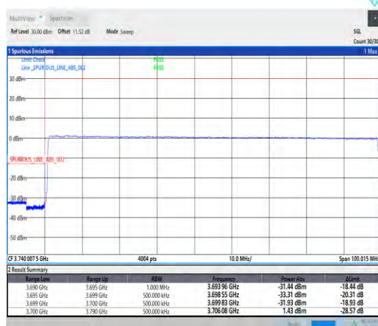
1-N77-3700-3980-PC2-30-90-L-6-CP-QPSK-Outer _Full-245@0-Ant1-1--PASS-see graph
