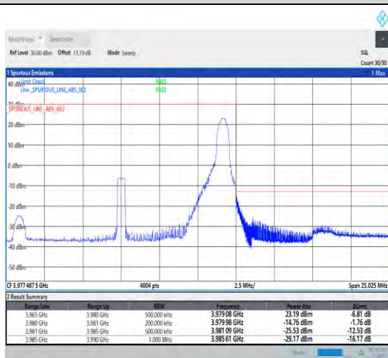
1-N77-3700-3980-PC2-30-15-H-2-DFT-PI2BPSK-Edge_1RB_Right-1@37-Ant1-1--PASS-see graph
