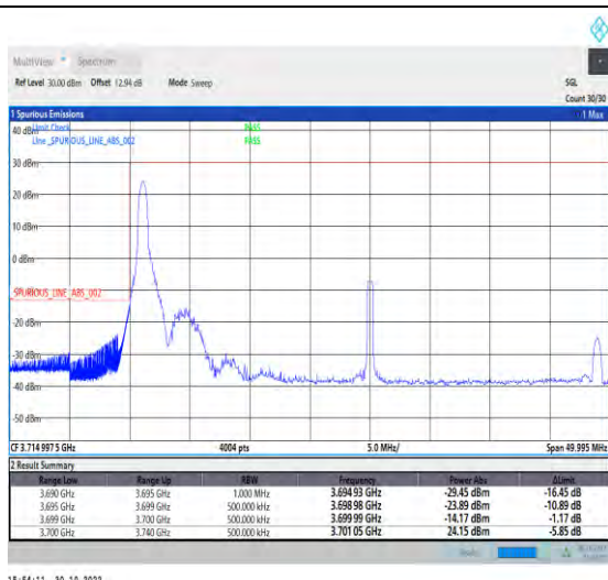
1-N77-3700-3980-PC2-30-40-L-1-DFT-PI2BPSK-Edge_1RB_Left-1@0-Ant1-1--PASS-see graph
