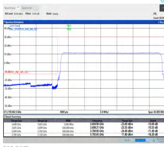
1-N77-3700-3980-PC2-30-20-L-6-CP-QPSK-Outer_Full-51@0-Ant1-1--PASS-see graph
