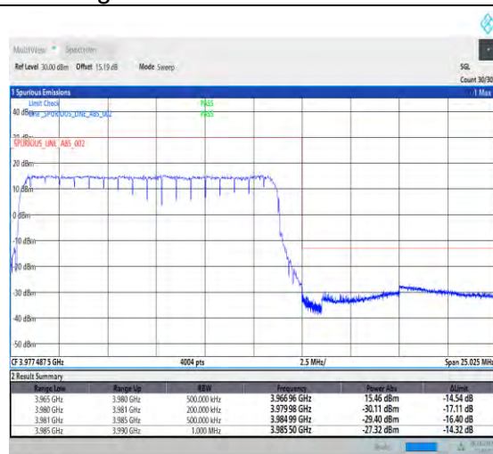
1-N77-3700-3980-PC2-30-15-H-3-DFT-PI2BPSK-Outer_Full-36@0-Ant1-1--PASS-see graph
