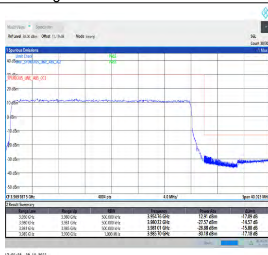
1-N77-3700-3980-PC2-30-30-H-3-DFT-PI2BPSK-Outer_Full-75@0-Ant1-1--PASS-see graph
