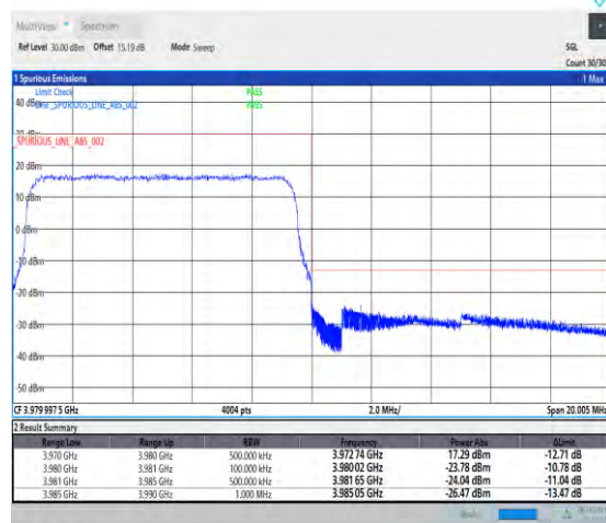
1-N77-3700-3980-PC2-30-10-H-3-DFT-PI2BPSK-Outer_Full-24@0-Ant1-1--PASS-see graph
