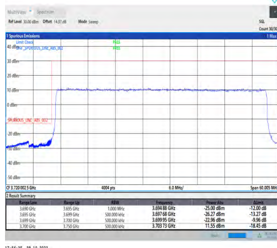
1-N77-3700-3980-PC2-30-50-L-3-DFT-PI2BPSK-Outer_Full-128@0-Ant1-1--PASS-see graph
