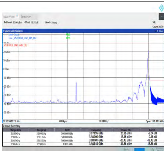
1-N77-3700-3980-PC2-30-100-H-2-DFT-QPSK-Edge_1RB_Right-1@272-Ant1-1--PASS-see graph
