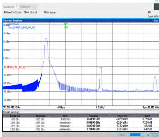
1-N77-3700-3980-PC2-30-30-L-1-DFT-PI2BPSK-Edge_1RB_Left-1@0-Ant1-1--PASS-see graph
