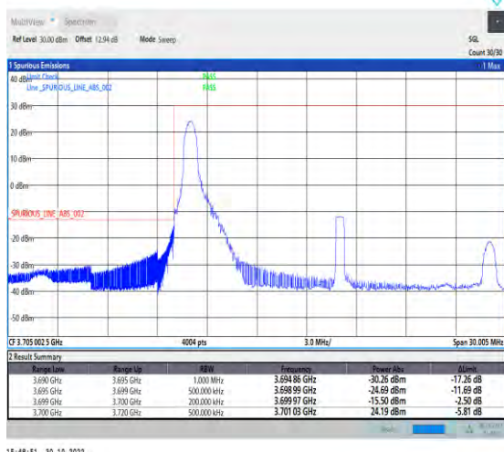
1-N77-3700-3980-PC2-30-20-L-1-DFT-PI2BPSK-Edge_1RB_Left-1@0-Ant1-1--PASS-see graph
