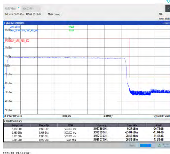
1-N77-3700-3980-PC2-30-30-H-6-CP-QPSK-Outer_Full-78@0-Ant1-1--PASS-see graph
