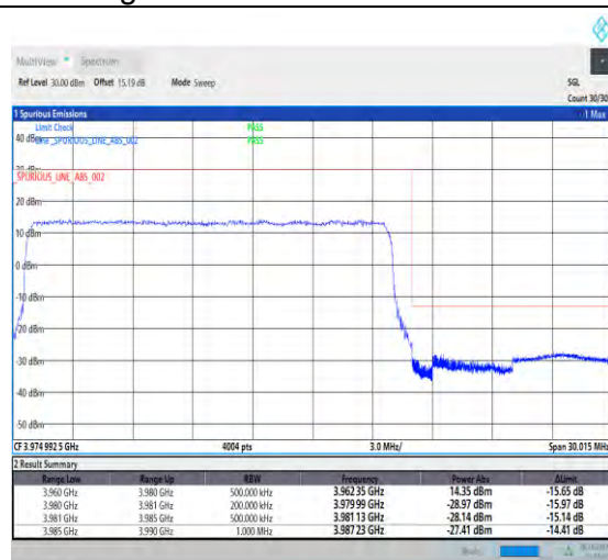
1-N77-3700-3980-PC2-30-20-H-3-DFT-PI2BPSK-Outer_Full-50@0-Ant1-1--PASS-see graph
