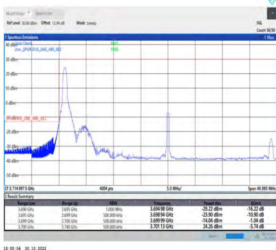
1-N77-3700-3980-PC2-30-40-L-4-CP-QPSK-Edge_1RB_Left-1@0-Ant1-1--PASS-see graph
