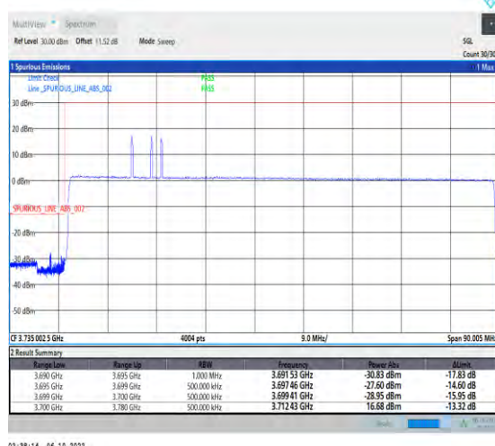
1-N77-3700-3980-PC2-30-80-L-6-CP-QPSK-Outer_Full-217@0-Ant1-1--PASS-see graph
