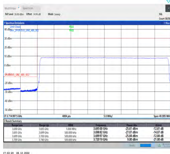
1-N77-3700-3980-PC2-30-40-L-6-CP-QPSK-Outer_Full-106@0-Ant1-1--PASS-see graph
