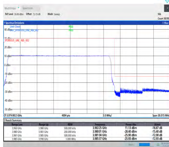
1-N77-3700-3980-PC2-30-20-H-6-CP-QPSK-Outer_Full-51@0-Ant1-1--PASS-see graph
