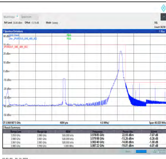
1-N77-3700-3980-PC2-30-30-H-2-DFT-PI2BPSK-Edge_1RB_Right-1@77-Ant1-1--PASS-see graph
