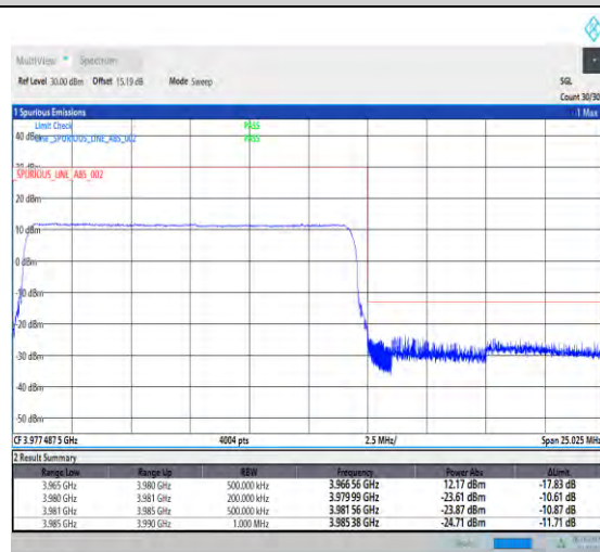
1-N77-3700-3980-PC2-30-15-H-3-DFT-PI2BPSK-Outer_Full-36@0-Ant1-1--PASS-see graph
