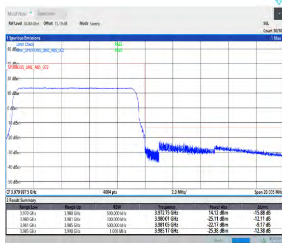
1-N77-3700-3980-PC2-30-10-H-6-CP-QPSK-Outer_Full-24@0-Ant1-1--PASS-see graph
