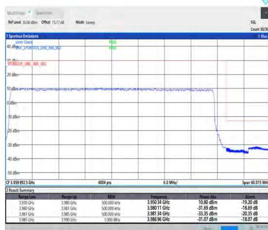
1-N77-3700-3980-PC2-30-50-H-6-CP-QPSK-Outer_Full-133@0-Ant1-1--PASS-see graph
