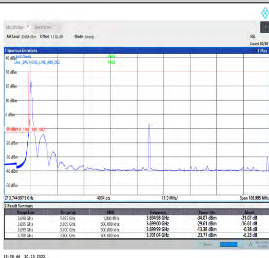
1-N77-3700-3980-PC2-30-100-L-4-CP-QPSK-Edge_1RB_Left-1@0-Ant1-1--PASS-see graph
