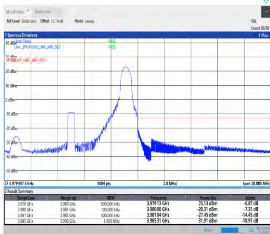
1-N77-3700-3980-PC2-30-10-H-2-DFT-PI2BPSK-Edge_1RB_Right-1@23-Ant1-1--PASS-see graph
