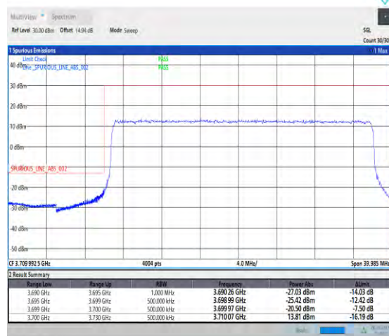
1-N77-3700-3980-PC2-30-30-L-3-DFT-PI2BPSK-Outer_Full-75@0-Ant1-1--PASS-see graph
