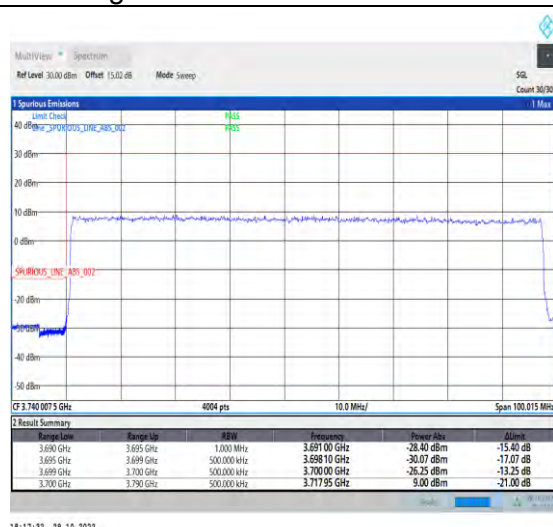
1-N77-3700-3980-PC2-30-90-L-3-DFT-PI2BPSK-Outer_Full-240@0-Ant1-1--PASS-see graph
