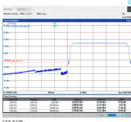
1-N77-3700-3980-PC2-30-10-L-6-CP-QPSK-Outer_Full-24@0-Ant1-1--PASS-see graph
