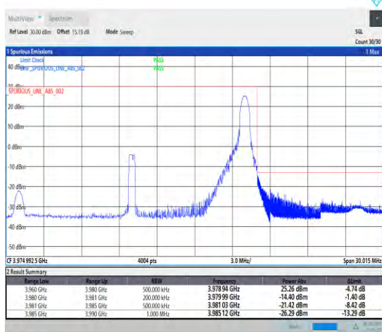
1-N77-3700-3980-PC2-30-20-H-5-CP-QPSK-Edge_1RB_Right-1@50-Ant1-1--PASS-see graph
