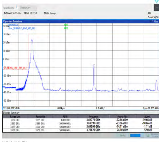
1-N77-3700-3980-PC2-30-50-L-4-CP-QPSK-Edge_1RB_Left-1@0-Ant1-1--PASS-see graph
