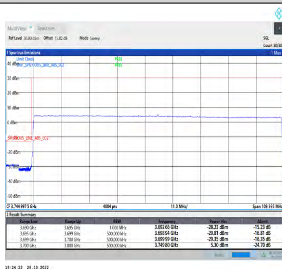
1-N77-3700-3980-PC2-30-100-L-6-CP-QPSK-Outer_Full-273@0-Ant1-1--PASS-see graph
