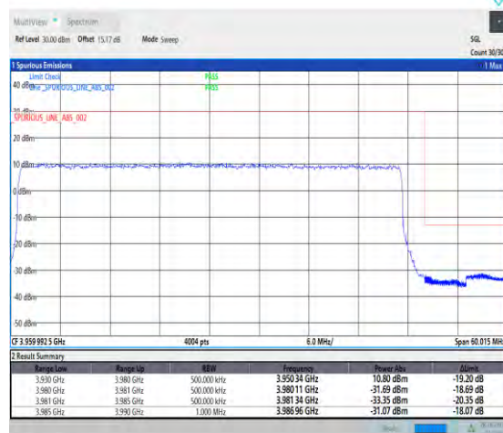
1-N77-3700-3980-PC2-30-50-H-3-DFT-PI2BPSK-Outer_Full-128@0-Ant1-1--PASS-see graph
