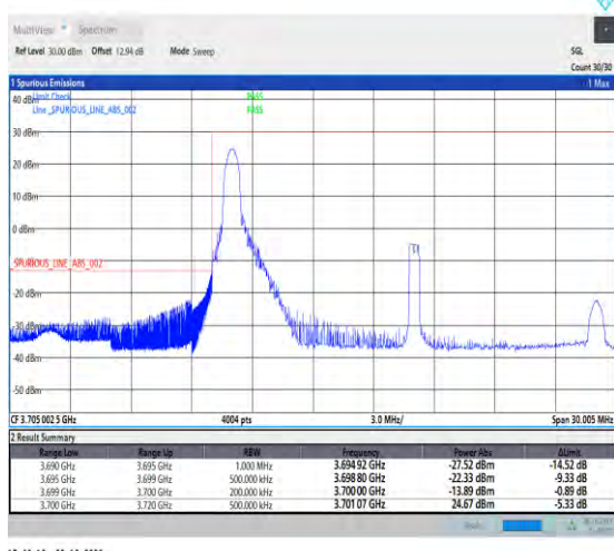
1-N77-3700-3980-PC2-30-20-L-4-CP-QPSK-Edge_1RB_Left-1@0-Ant1-1--PASS-see graph
