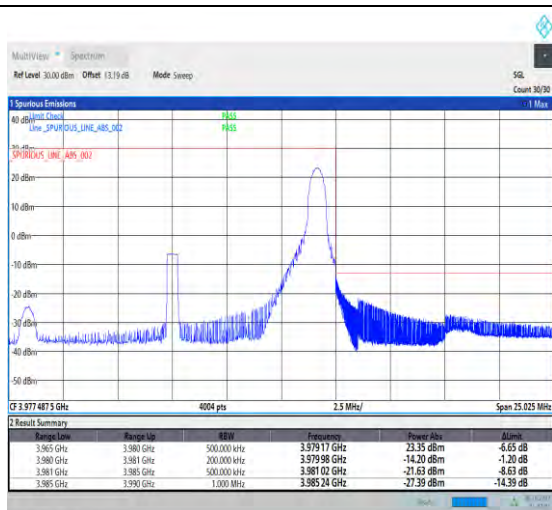
1-N77-3700-3980-PC2-30-15-H-2-DFT-PI2BPSK-Edge_1RB_Right-1@37-Ant1-1--PASS-see graph
