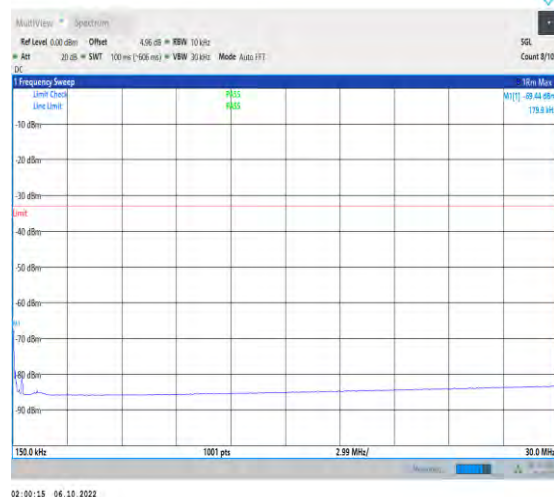
1-N77-3700-3980-PC2-30-100-L-1-DFT-QPSK-Inner _1RB_Left-1@1-0.15-30-Ant1-0.18--69.44--33-PASS
