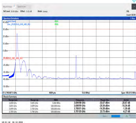
1-N77-3700-3980-PC2-30-90-L-4-CP-QPSK-Edge_1RB_Left-1@0-Ant1-1--PASS-see graph
