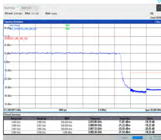
1-N77-3700-3980-PC2-30-40-H-3-DFT-PI2BPSK-Outer_Full-100@0-Ant1-1--PASS-see graph
