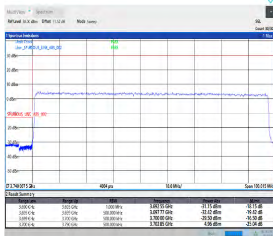
1-N77-3700-3980-PC2-30-90-L-3-DFT-QPSK-Outer _Full-240@0-Ant1-1--PASS-see graph
