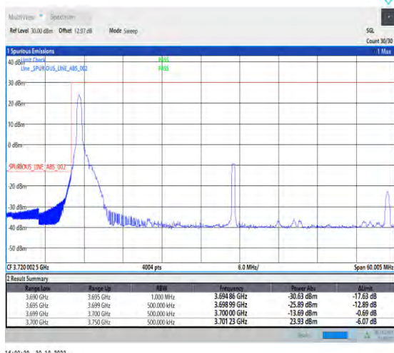
1-N77-3700-3980-PC2-30-50-L-1-DFT-PI2BPSK-Edge_1RB_Left-1@0-Ant1-1--PASS-see graph
