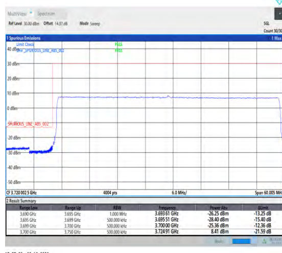
1-N77-3700-3980-PC2-30-50-L-6-CP-QPSK-Outer_Full-133@0-Ant1-1--PASS-see graph
