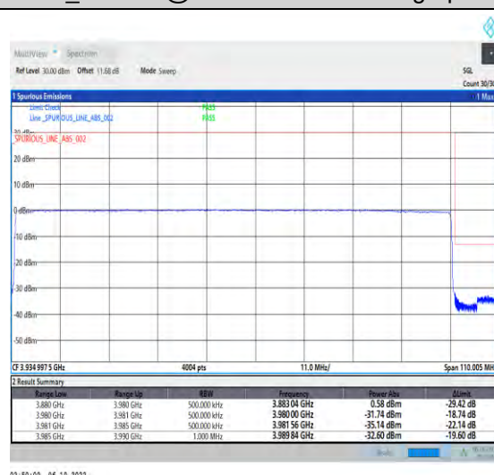
1-N77-3700-3980-PC2-30-100-H-6-CP-QPSK-Out_Full-273@0-Ant1-1--PASS-see graph
