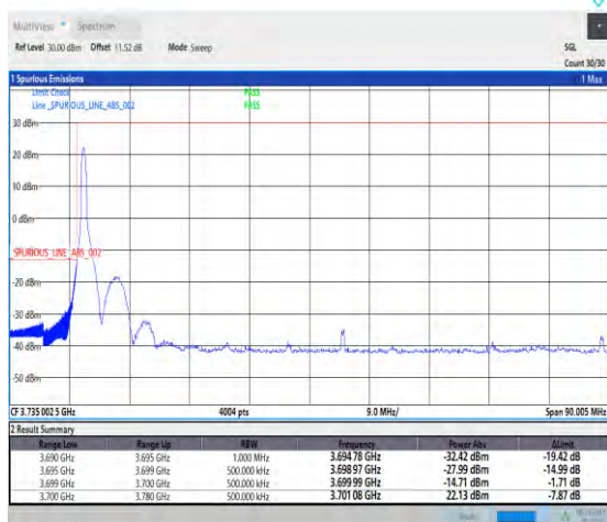
1-N77-3700-3980-PC2-30-80-L-1-DFT-QPSK-Edge_1 RB_Left-1@0-Ant1-1--PASS-see graph
