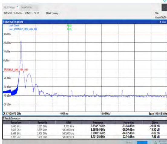
1-N77-3700-3980-PC2-30-90-L-1-DFT-QPSK-Edge_1 RB_Left-1@0-Ant1-1--PASS-see graph
