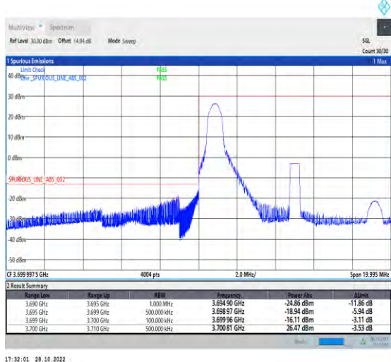
1-N77-3700-3980-PC2-30-10-L-4-CP-QPSK-Edge_1RB_Left-1@0-Ant1-1--PASS-see graph
