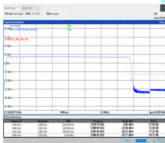
1-N77-3700-3980-PC2-30-40-H-6-CP-QPSK-Outer_Full-106@0-Ant1-1--PASS-see graph
