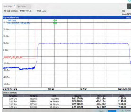
1-N77-3700-3980-PC2-30-30-L-6-CP-QPSK-Outer_Full-78@0-Ant1-1--PASS-see graph
