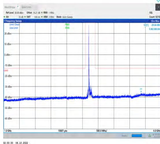
1-N77-3700-3980-PC2-30-100-L-1-DFT-QPSK-Inner _1RB_Left-1@1-1000-6000-Ant1-5362.00--35.64--13
