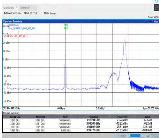
1-N77-3700-3980-PC2-30-40-H-5-CP-QPSK-Edge_1RB_Right-1@105-Ant1-1--PASS-see graph
