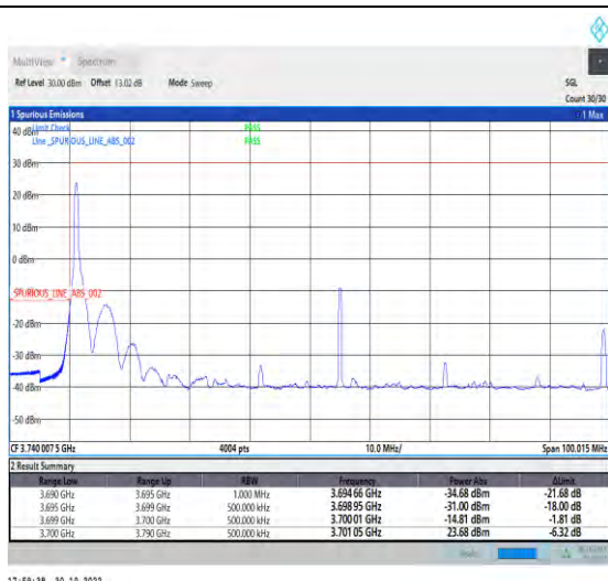
1-N77-3700-3980-PC2-30-90-L-1-DFT-PI2BPSK-Edge_1RB_Left-1@0-Ant1-1--PASS-see graph
