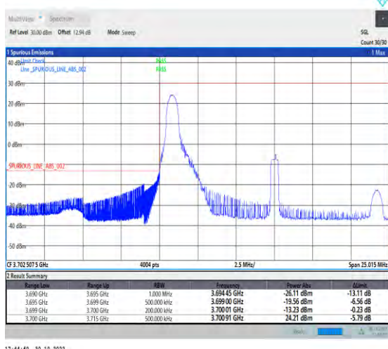
1-N77-3700-3980-PC2-30-15-L-4-CP-QPSK-Edge_1RB_Left-1@0-Ant1-1--PASS-see graph
