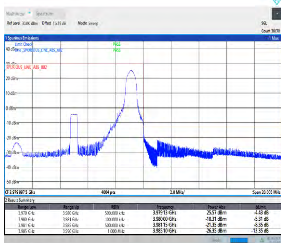
1-N77-3700-3980-PC2-30-10-H-5-CP-QPSK-Edge_1RB_Right-1@23-Ant1-1--PASS-see graph
