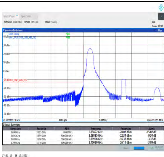
1-N77-3700-3980-PC2-30-10-L-1-DFT-PI2BPSK-Edge_1RB_Left-1@0-Ant1-1--PASS-see graph
