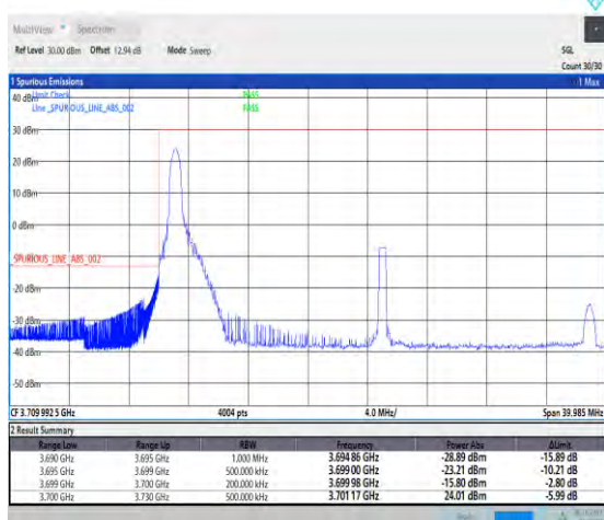
1-N77-3700-3980-PC2-30-30-L-4-CP-QPSK-Edge_1RB_Left-1@0-Ant1-1--PASS-see graph
