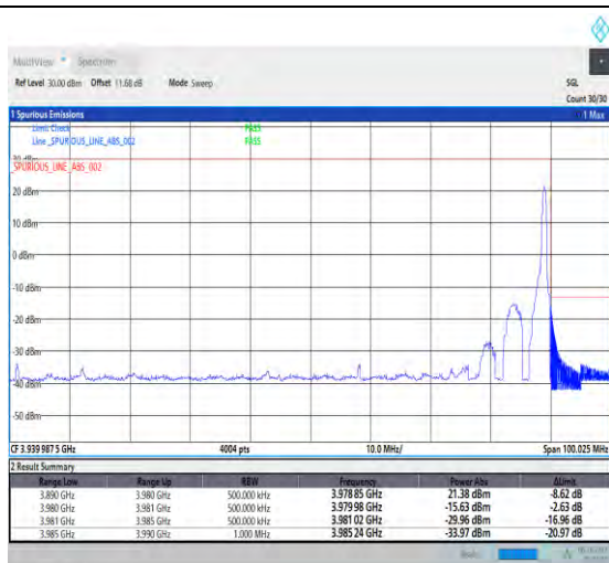
1-N77-3700-3980-PC2-30-90-H-2-DFT-QPSK-Edge_1 RB_Right-1@244-Ant1-1--PASS-see graph
