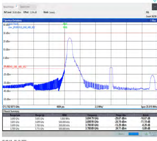
1-N77-3700-3980-PC2-30-15-L-1-DFT-PI2BPSK-Edge_1RB_Left-1@0-Ant1-1--PASS-see graph
