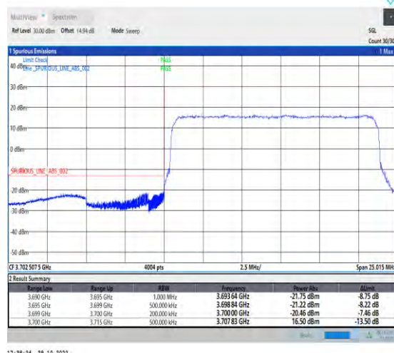
1-N77-3700-3980-PC2-30-15-L-3-DFT-PI2BPSK-Outer_Full-36@0-Ant1-1--PASS-see graph
