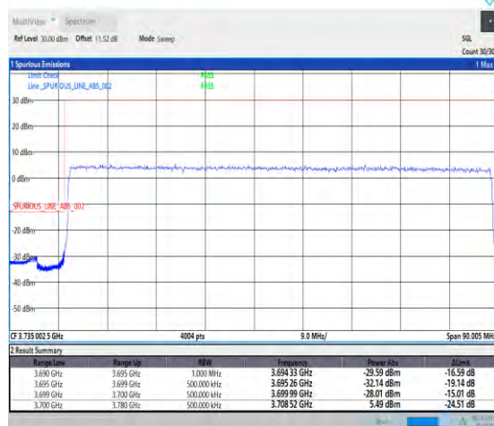
1-N77-3700-3980-PC2-30-80-L-3-DFT-QPSK-Outer_Full-216@0-Ant1-1--PASS-see graph
