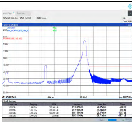
1-N77-3700-3980-PC2-30-20-H-2-DFT-PI2BPSK-Edge_1RB_Right-1@50-Ant1-1--PASS-see graph
