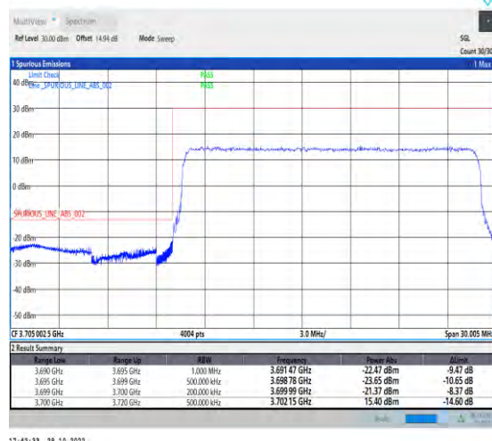
1-N77-3700-3980-PC2-30-20-L-3-DFT-PI2BPSK-Outer_Full-50@0-Ant1-1--PASS-see graph
