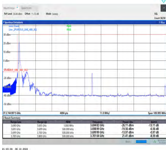
1-N77-3700-3980-PC2-30-100-L-4-CP-QPSK-Edge_1 RB_Left-1@0-Ant1-1--PASS-see graph
