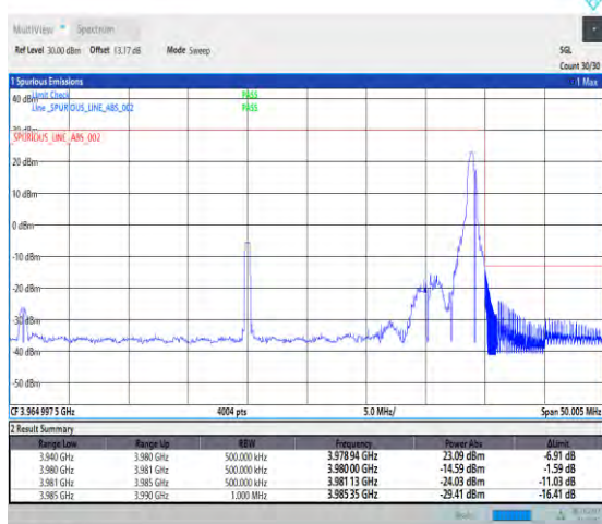
1-N77-3700-3980-PC2-30-40-H-2-DFT-PI2BPSK-Edge_1RB_Right-1@105-Ant1-1--PASS-see graph
