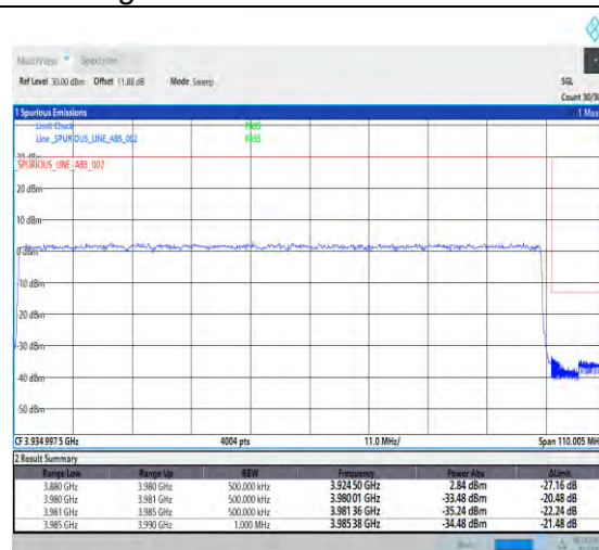
1-N77-3700-3980-PC2-30-100-H-3-DFT-QPSK-Out_Full-270@0-Ant1-1--PASS-see graph
