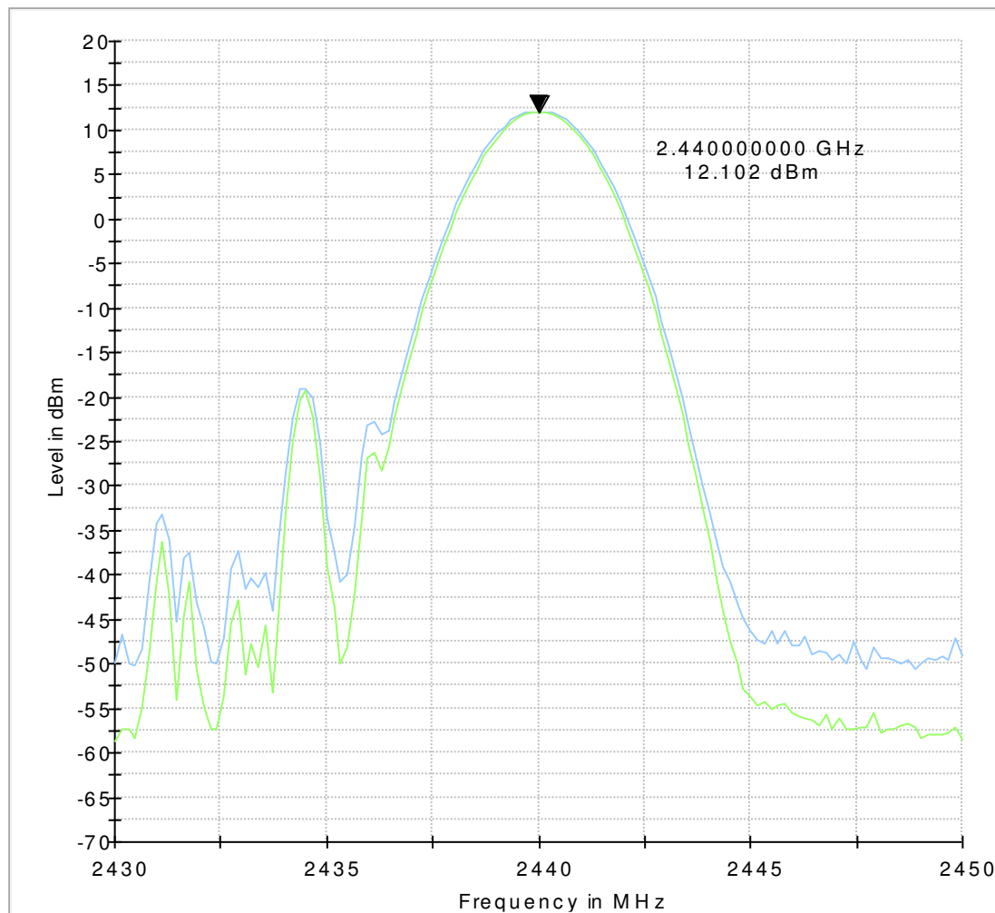
FCC_15_247_EIRP_1GHz_3GHz
