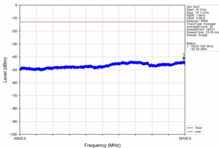
Band2 HSUPA MCH 1880MHz Subtest 1 NTN
