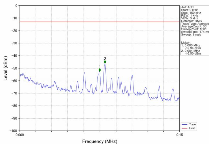
Band2_RMC_HCH_1907.6MHz_12.2kbps_RMC_NTNV
