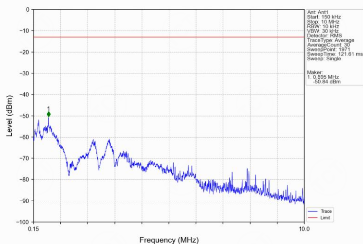
Band2_HSDPA_MCH_1880MHz_Subtest 1_NTNV
