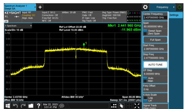
Channel 06 (2437MHz)
