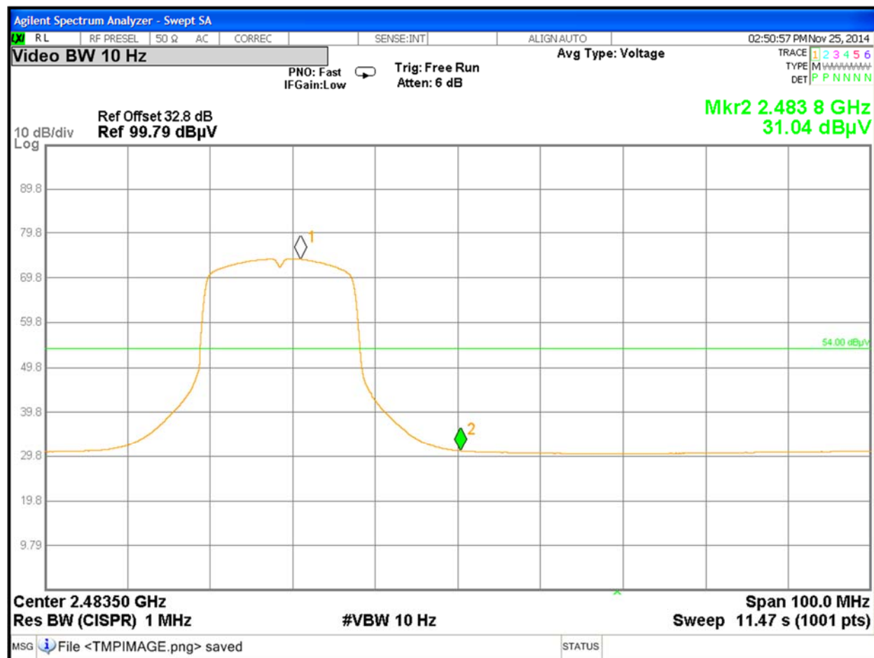
Figure 39: Radiated Emission at the Edge for Channel 2480 MHz at 6.5Mbps– Horizontal (Avg)
