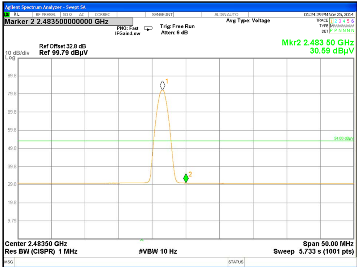
Figure 49: Radiated Emission at the Edge for Channel 2480 MHz at 1Mbps BLE mode– Vertical (Avg)
