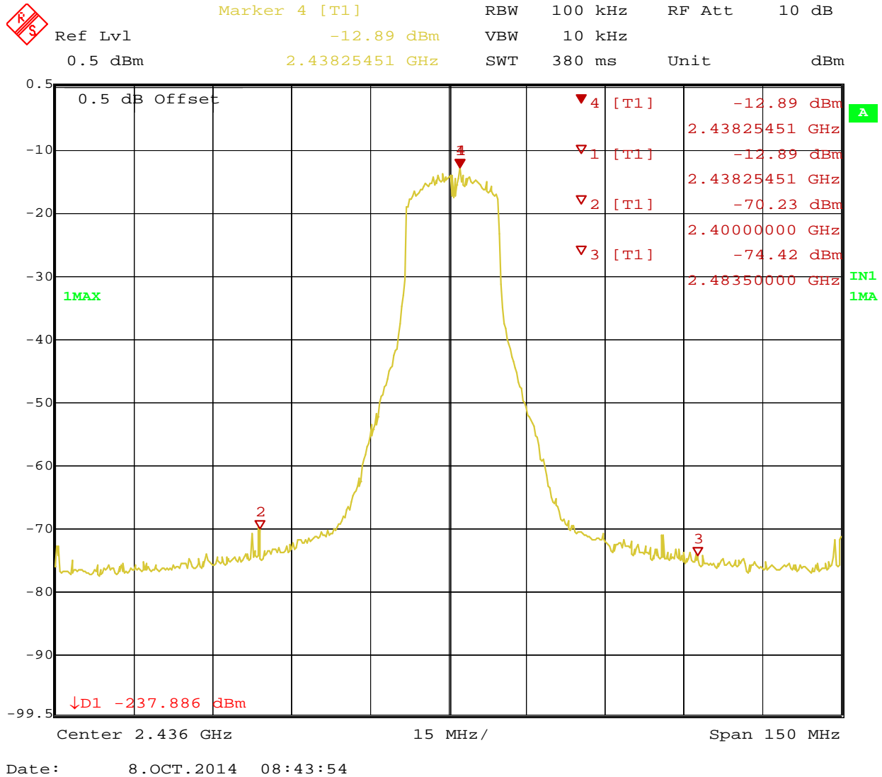
Figure 14: Band-edge Requirement at Operating Channel 2437 MHz
