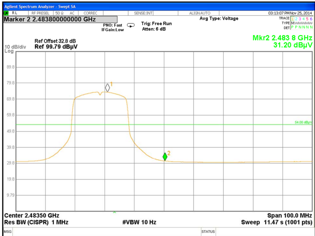
Figure 41: Radiated Emission at the Edge for Channel 2462 MHz at 6.5Mbps HT20 mode– Horizontal (Avg)
