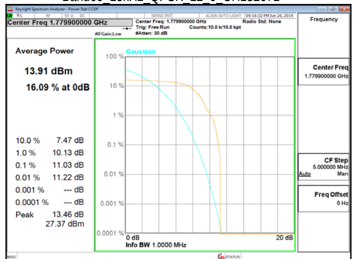
Band66 15kHz QPSK 12 0 CH132671
