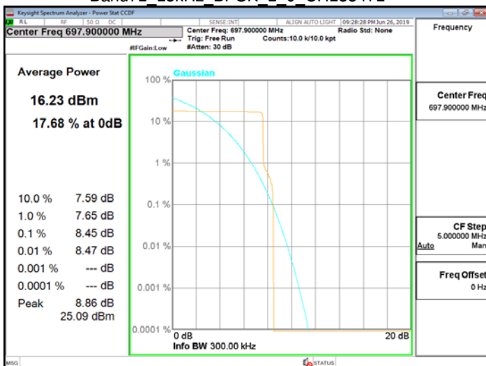
Band71 15kHz BPSK 1 0 CH133471
