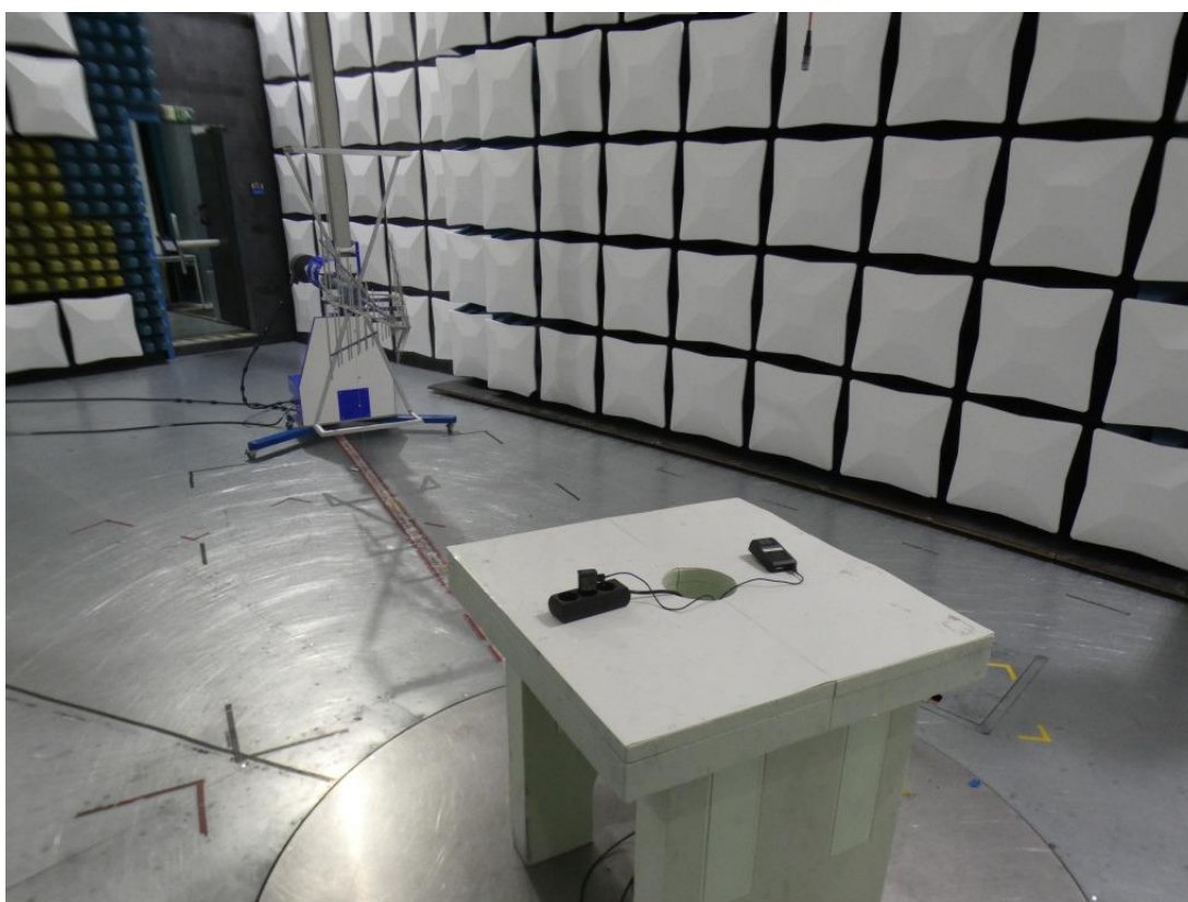
Photo 4: Test setup S02_AA01 for radiated emissions measurements below 1 GHz
