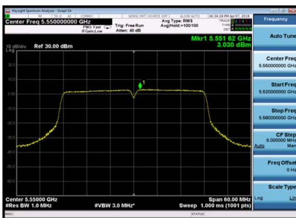
U-NII-2C, 802.11n HT40, Channel No.: 110
