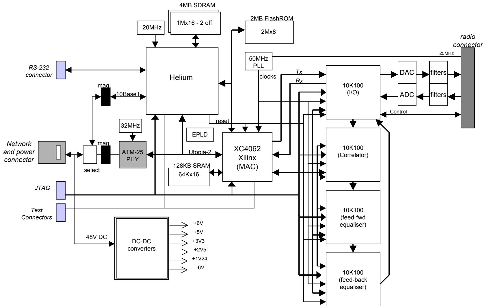
Figure 2 : System Motherboard
