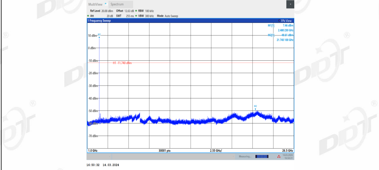
2DH5_Left side_2480_0~Reference
