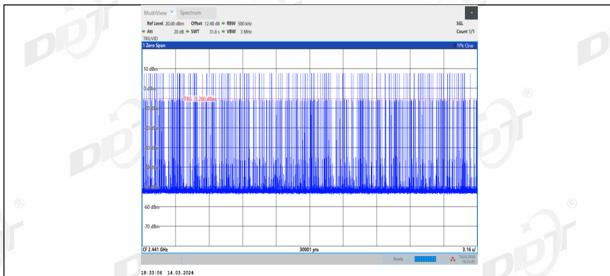
3DH3_Right side_Hop
