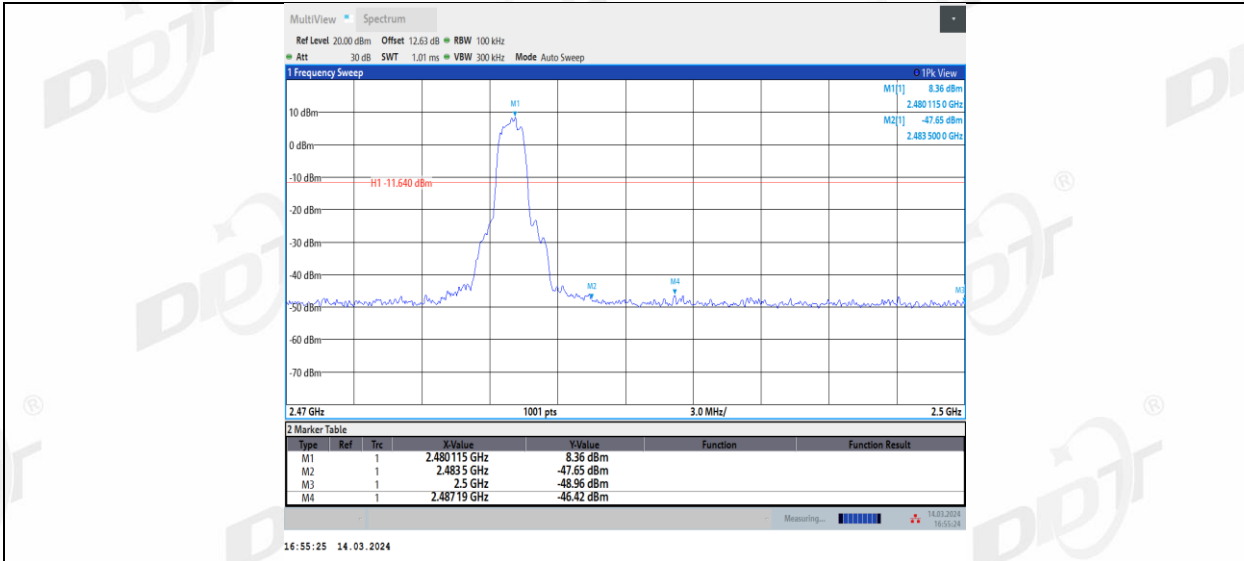
3DH5_Left side_High_2480
