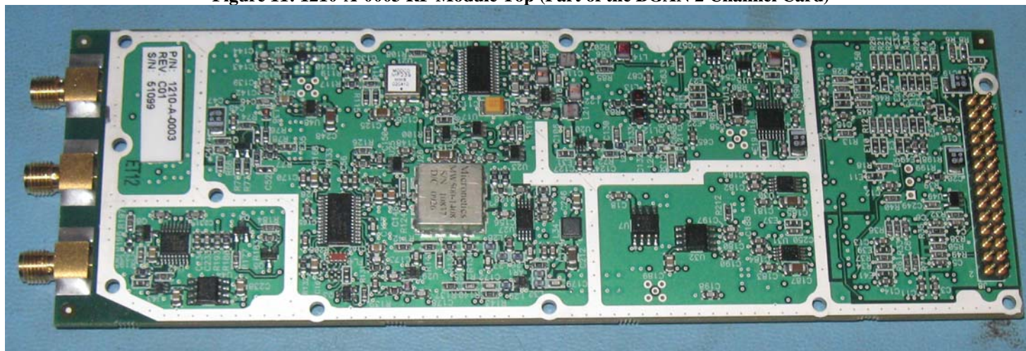
Figure 12: 1210-A-0003 RF Module Bottom (Part of the BGAN 2 Channel Card)
