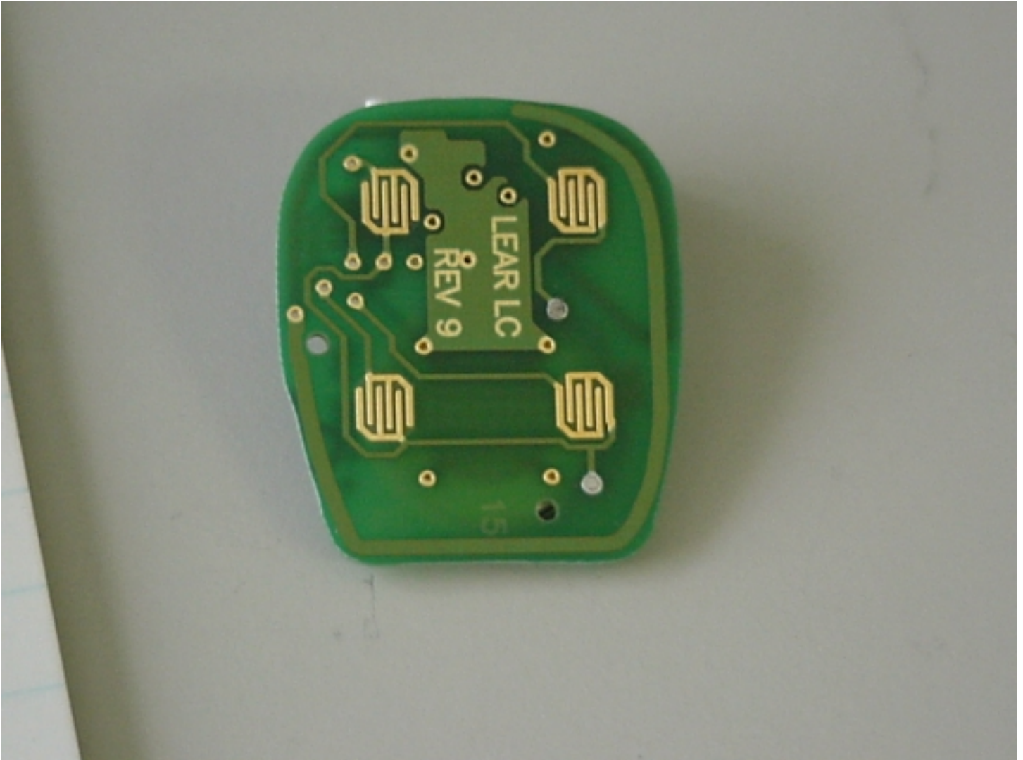
Bottom side of Board
