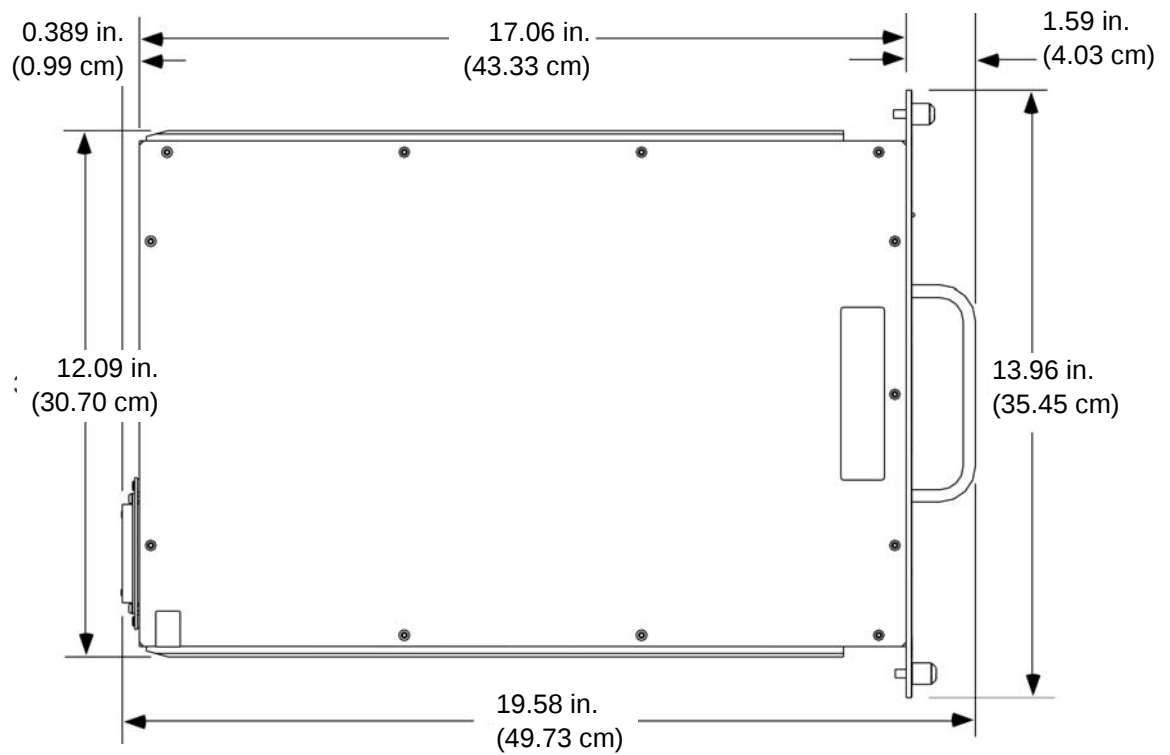
Figure 1-2. Model G3H-851-80 Amplifier Side View
