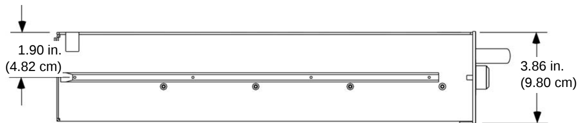
Figure 1-3. Model G3H-851-80 Amplifier Bottom View
