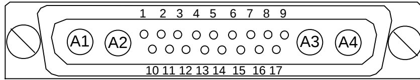
Figure 2-2. Combo Connector (Male, on Rear of G3H-851-80 Amplifier Module)
