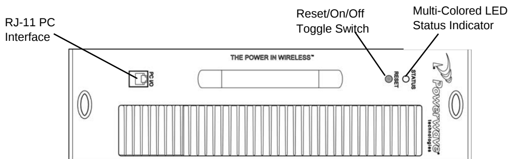
Figure 3-1. G3H-851-80 Controls and Indicators
