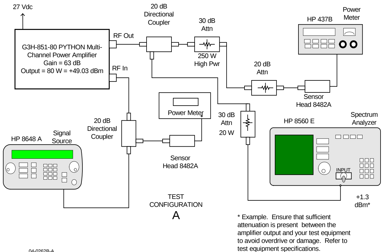
Figure 5-1. Amplifier Test Setup Diagram – Configuration A
