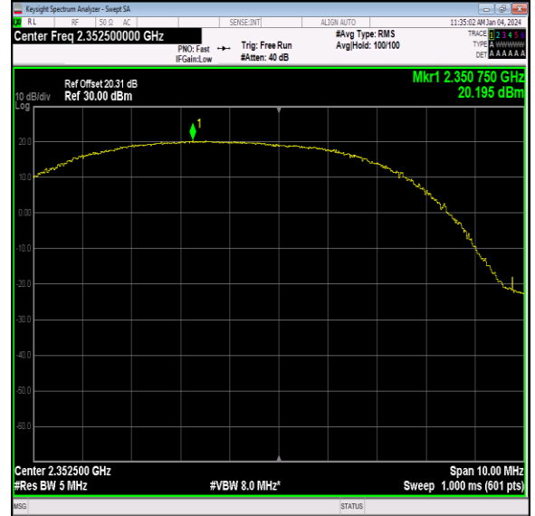
40(2350-2360)-5MHz-QPSK-39175-12RB#0-PASS
