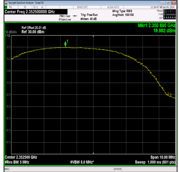
40(2350-2360)-5MHz-QPSK-39175-1RB#12-PASS
