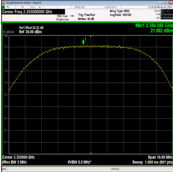
40(2350-2360)-5MHz-QPSK-39200-1RB#12-PASS
