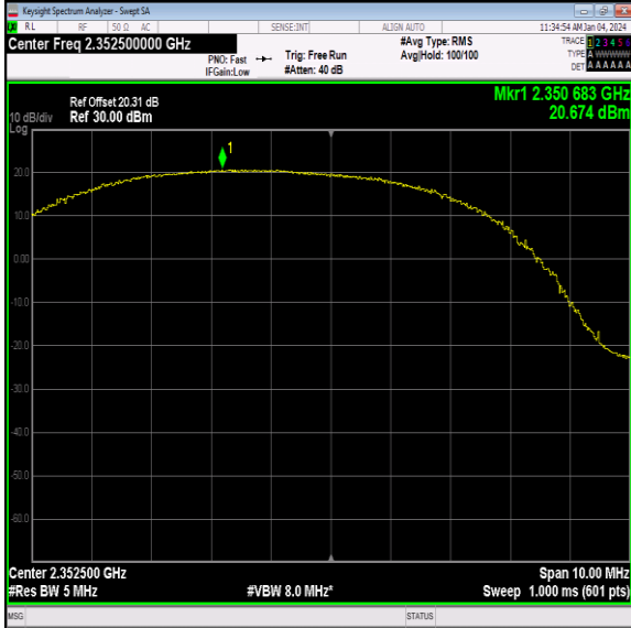
40(2350-2360)-5MHz-QPSK-39175-1RB#24-PASS
