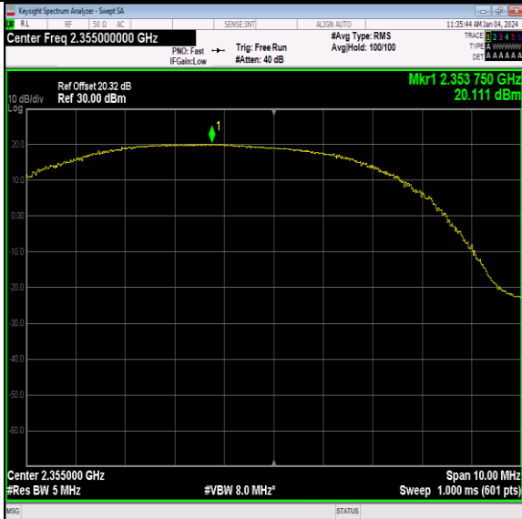
40(2350-2360)-5MHz-QPSK-39200-12RB#0-PASS
