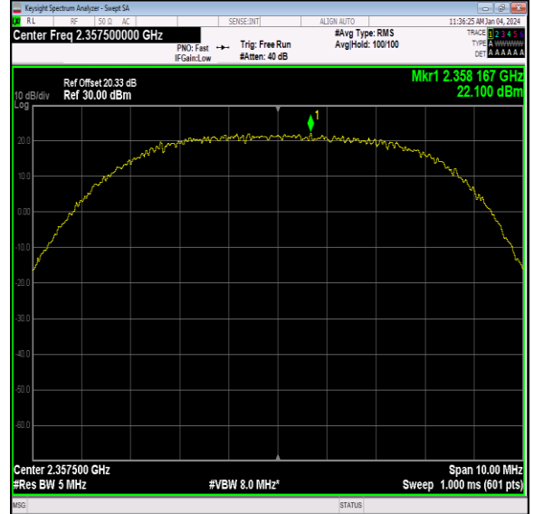
40(2350-2360)-5MHz-QPSK-39225-1RB#12-PASS
