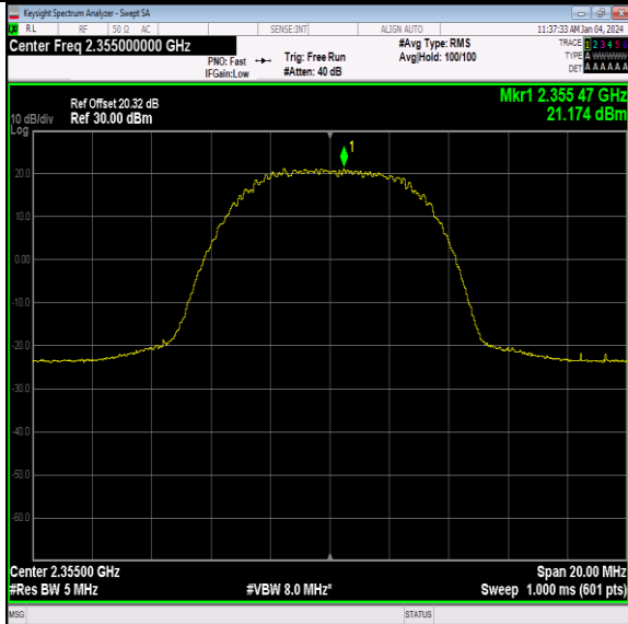
40(2350-2360)-10MHz-QPSK-39200-1RB#24-PASS
