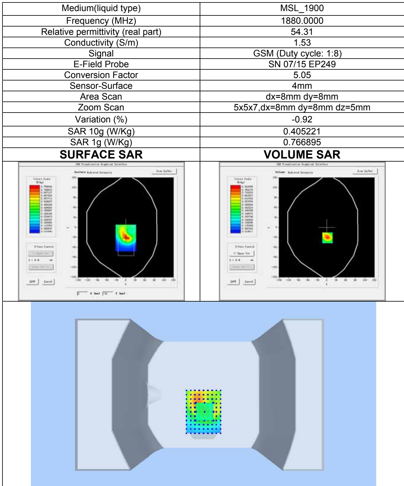
Plot 5: GSM1900, Middle channel (Body-worn, Back Surface) Product Description: MOBILE PHONE Test Date: Apr 21,2017
