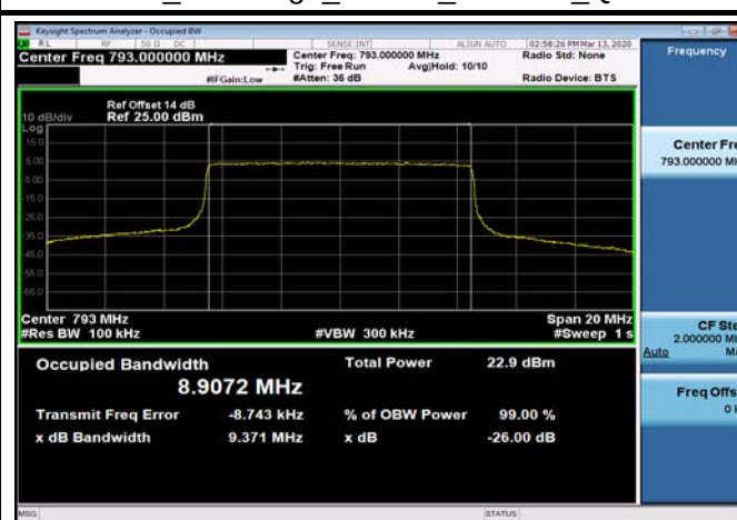
FDD14_MidRange_10MHz_793MHz_QPSK
