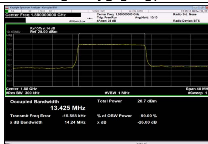
FDD02_MidRange_15_1880_QPSK
