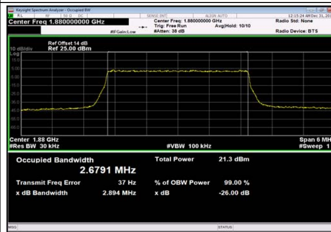
FDD02_MidRange_3_1880_QPSK
