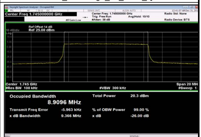
FDD66_MidRange_10_1745_Q16
