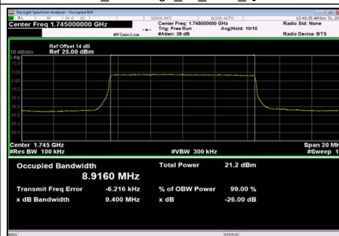
FDD66_MidRange_10_1745_QPSK
