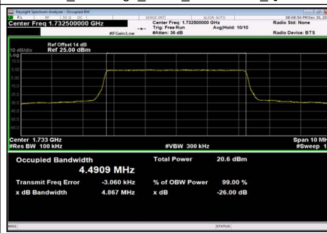
FDD04_MidRange_5MHz_1732.5MHz_QPSK
