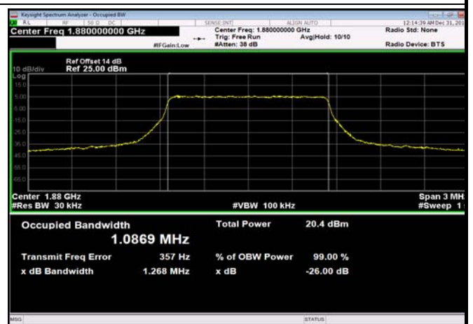
FDD02_MidRange_3_1880_Q16
