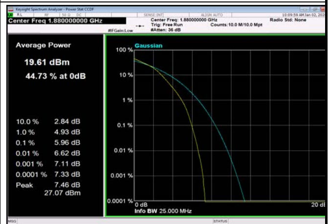
FDD02_HighRange_20MHz_1900_fullRB _Q16
