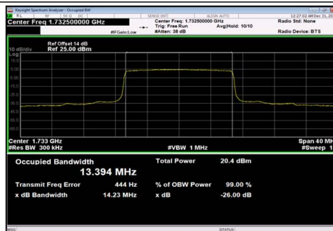
FDD04_MidRange_15_1732.5_QPSK
