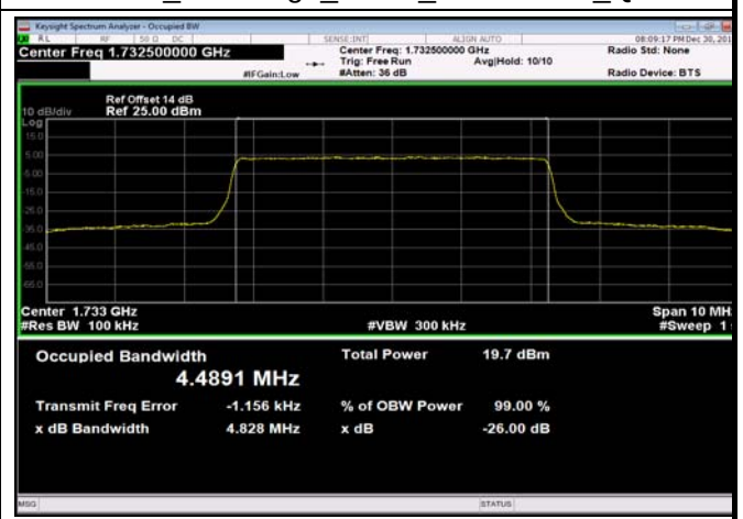
FDD04_MidRange_5MHz_1732.5MHz_Q16
