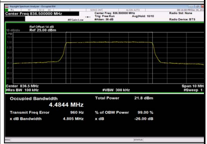
FDD05_MidRange_5MHz_836.5MHz_Q16
