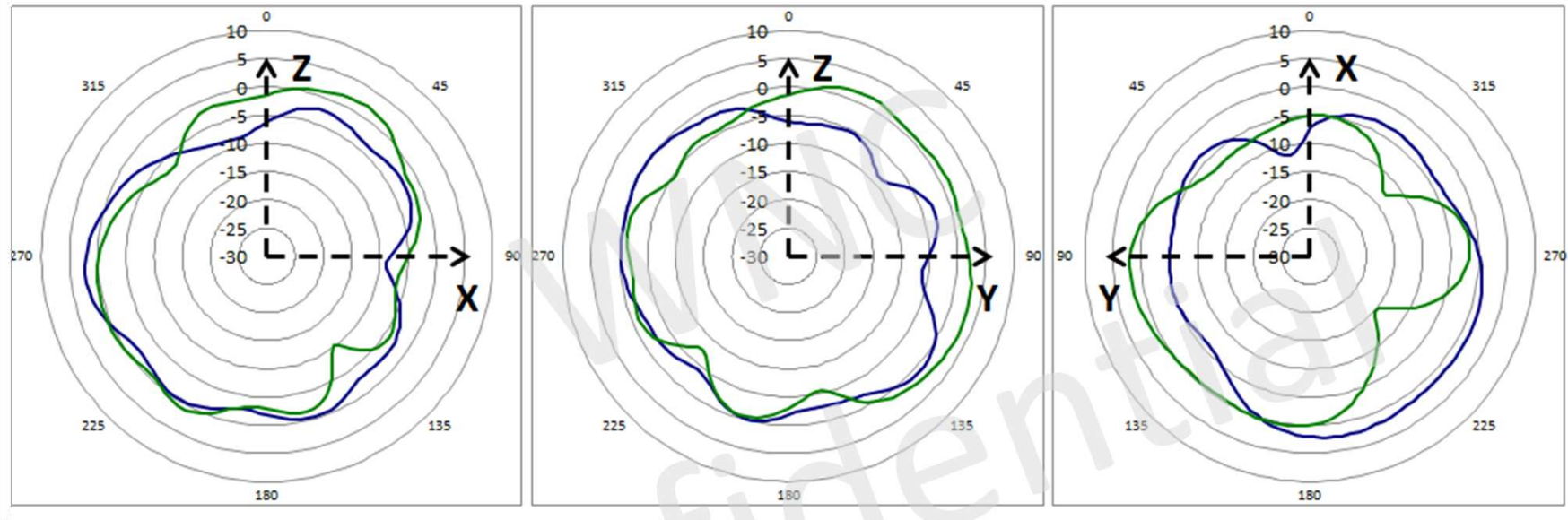
2450 MHz Radiation Pattern
