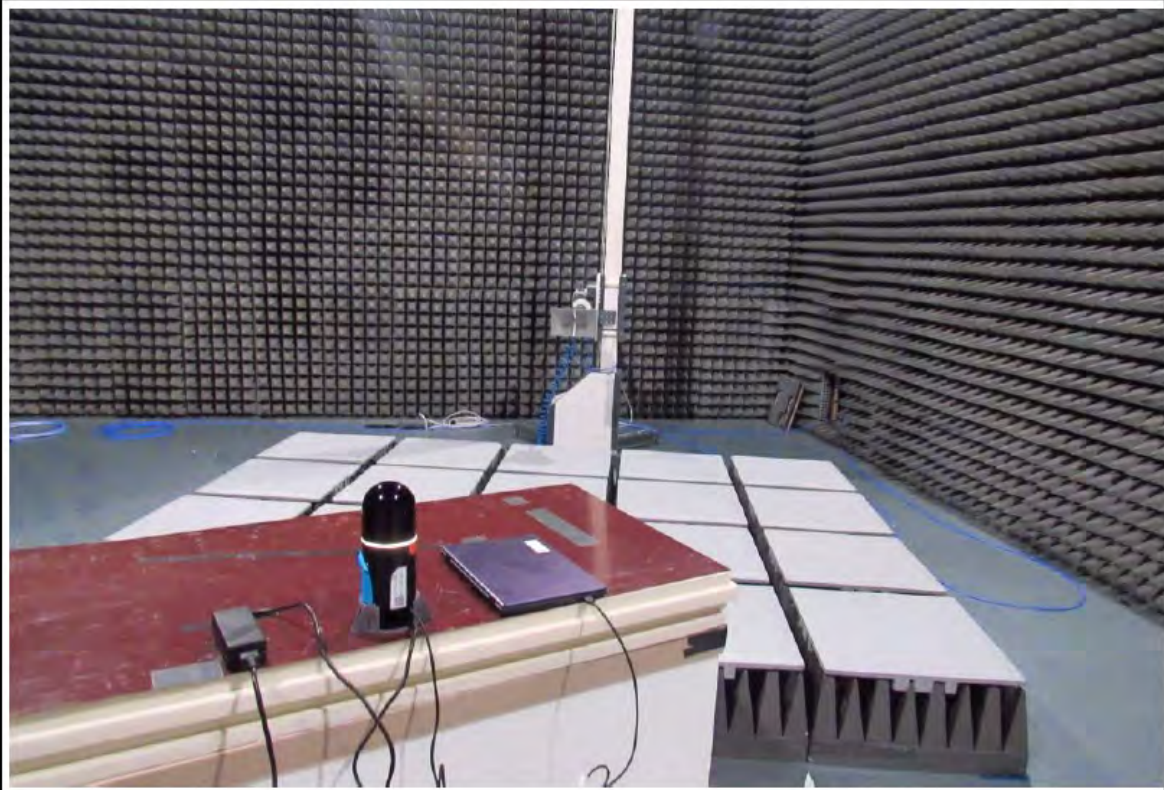
Setup 1-6.5 GHz
