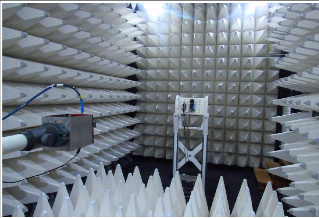
Setup 18-26 GHz
