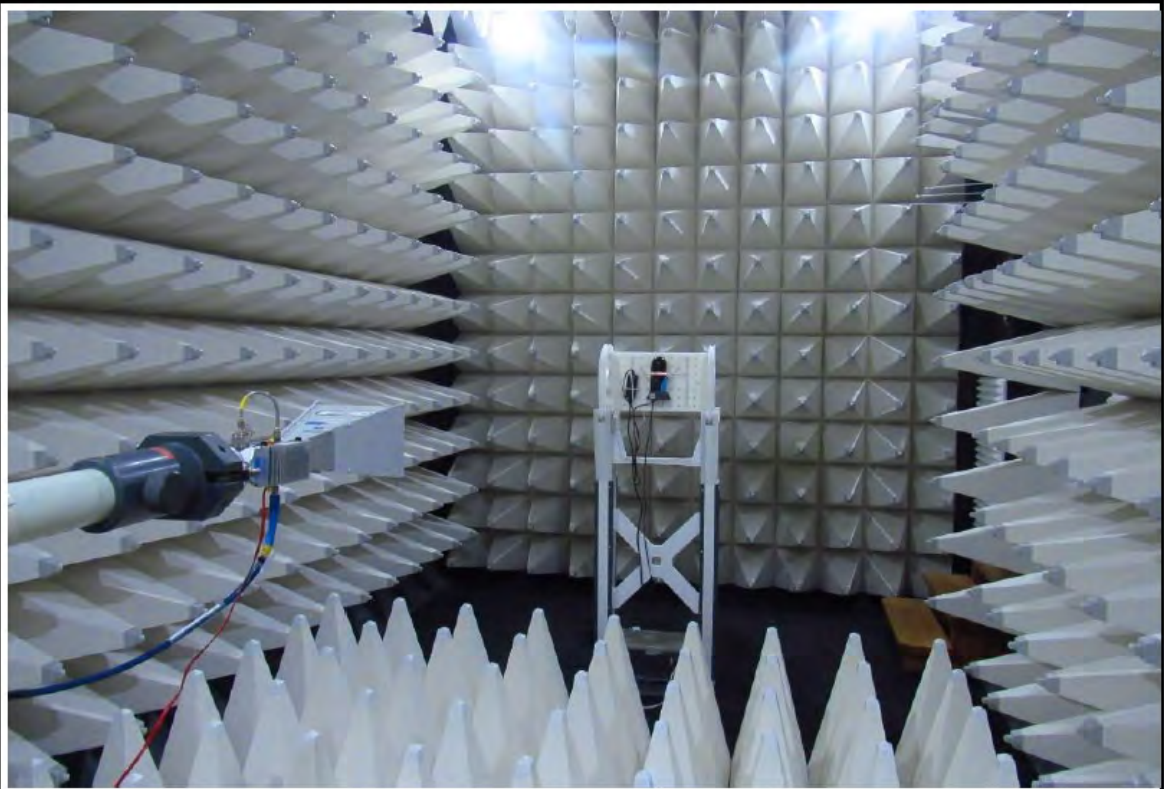
Setup 6.5-18 GHz
