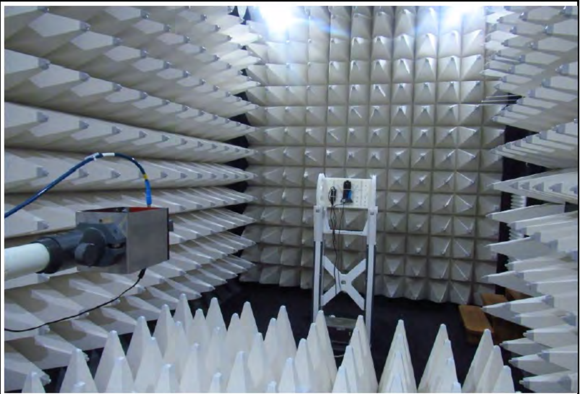
Setup 18-26 GHz
