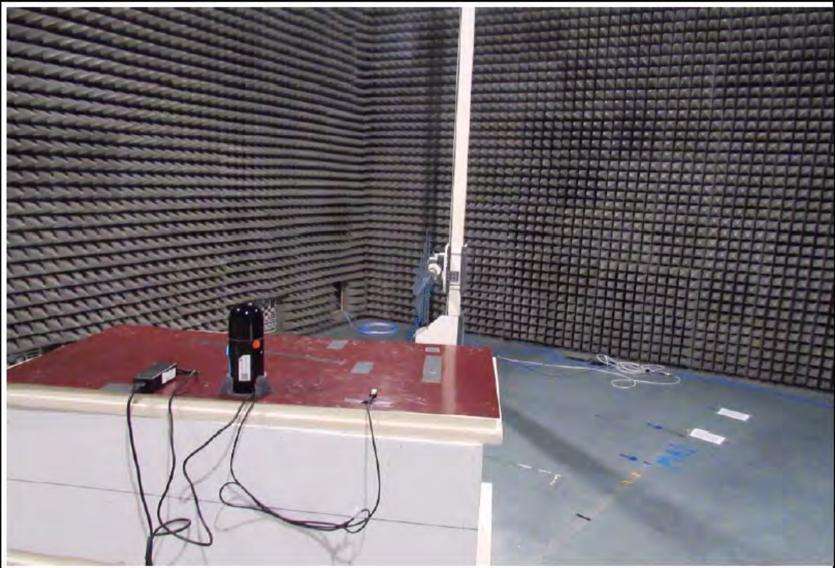
Setup 200 – 1000 MHz
