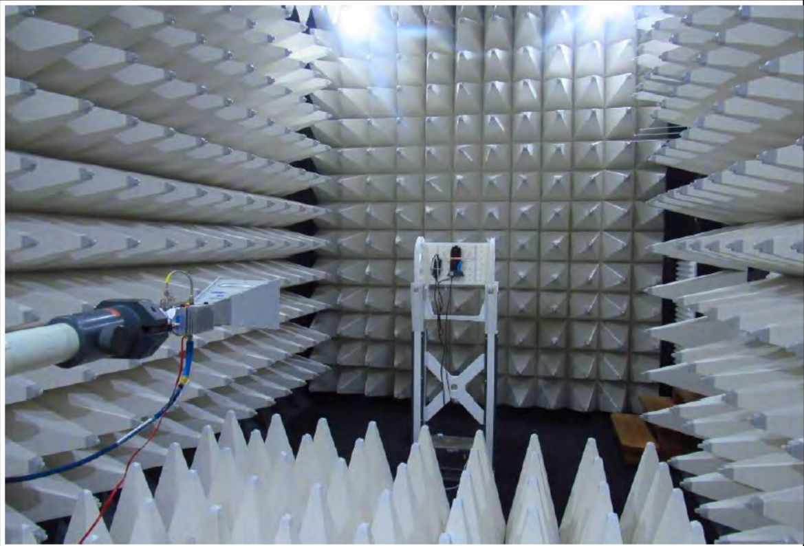
Setup 6.5-18 GHz
