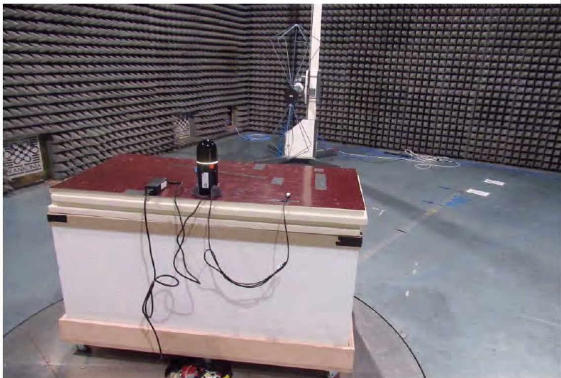
Setup 30 - 200 MHz
