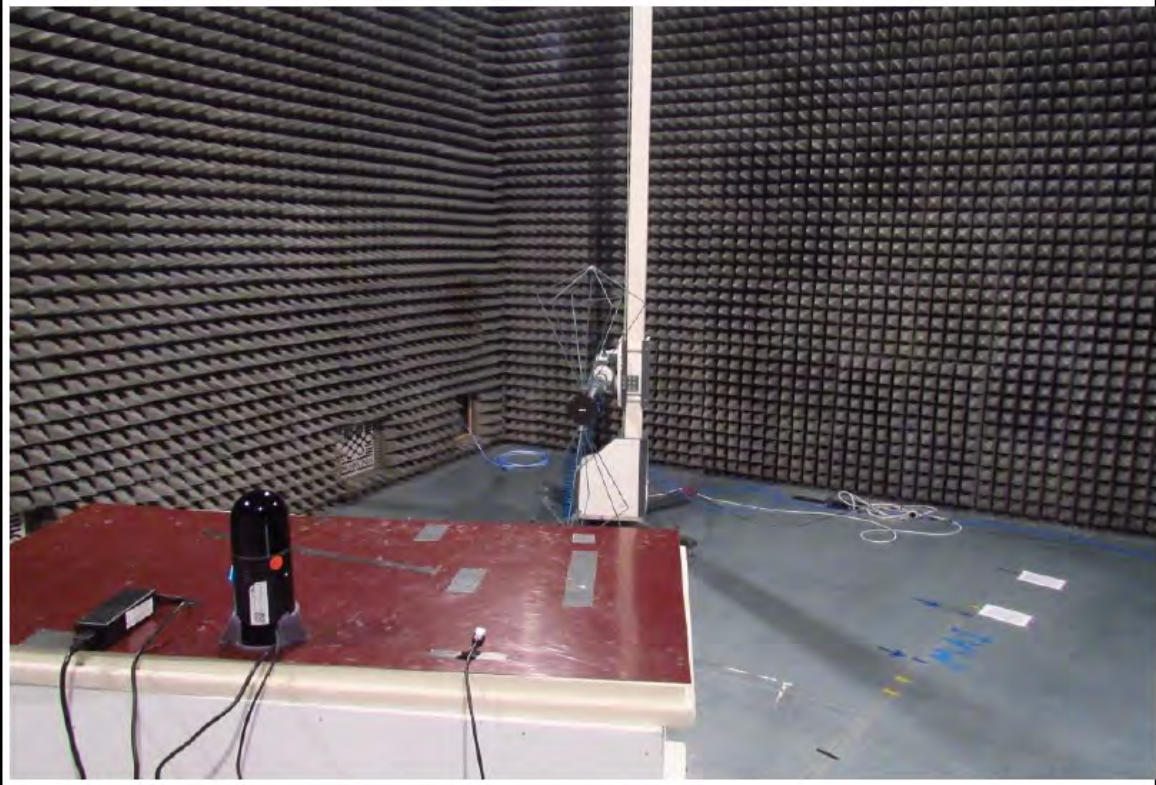
Setup 30 - 200 MHz
