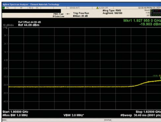
3G WCDMA PCS Band II Test Case 1 QPSK Modulation Low Channel, 1932.4 MHz
