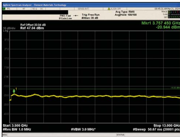
3G WCDMA PCS Band II Test Case 1 16QAM Modulation (WCDMA) and QPSK Modulation (LTE)
