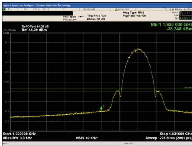
2G GSM/EDGE Band 2 Test Case 3 8PSK Modulation Lower Band Edge
