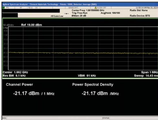
2G GSM/EDGE Band 2 Test Case 2 8PSK Modulation Upper Band Edge
