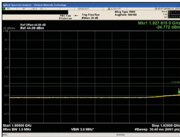
2G GSM/EDGE Band 2 8PSK Modulation Reduced Power Low Channel, 1930.2 MHz
