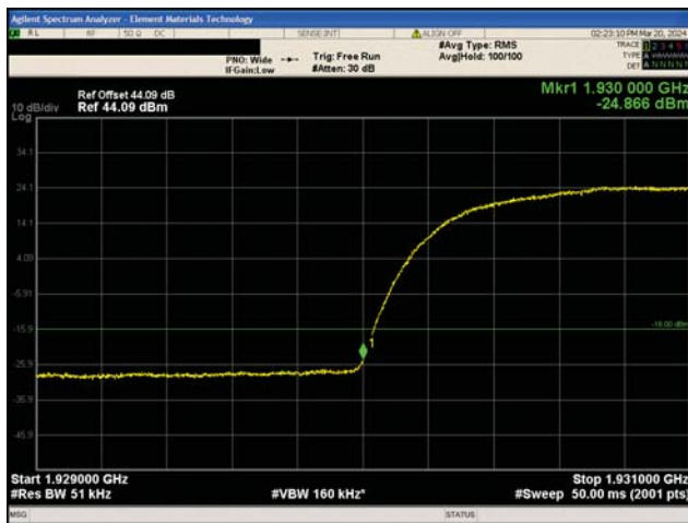
3G WCDMA PCS Band II Test Case 1 16QAM Modulation Low Channel, 1932.4 MHz
