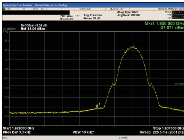
2G GSM/EDGE Band 2 GMSK Modulation One Channel Inside Low Channel, 1930.4 MHz
