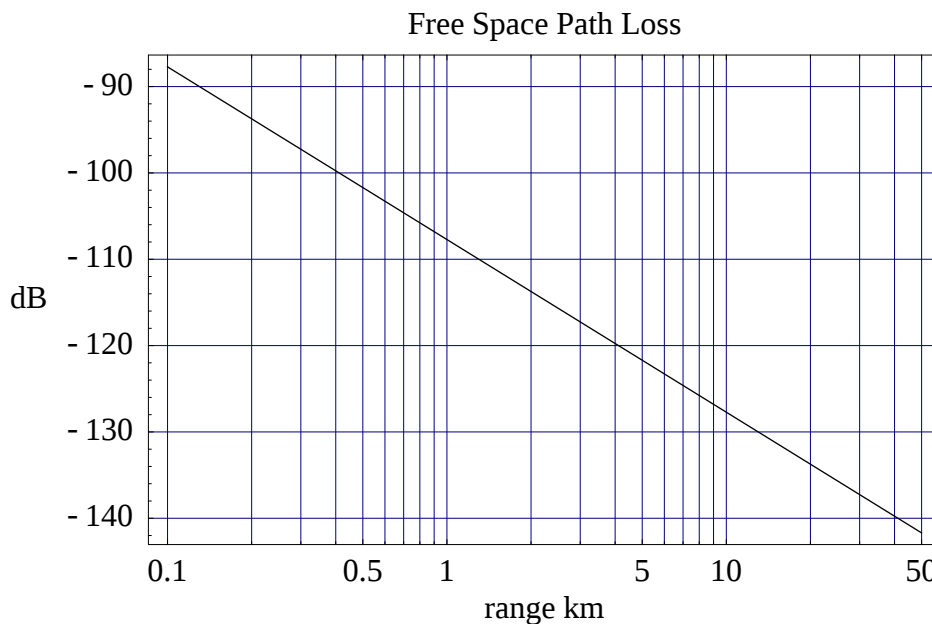
Figure 8 Free Space Path Loss at 5.8 GHz
