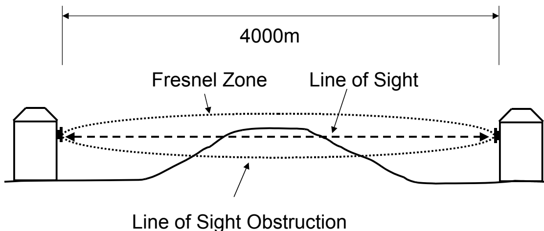
Figure 11 Worked Example over a hill
