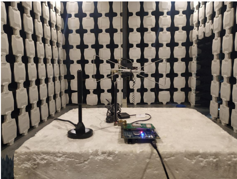
Pic 1.ERP and EIRP Test Setup photo first step
