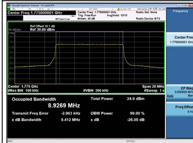
LTE band 66 - High CH QPSK-10
