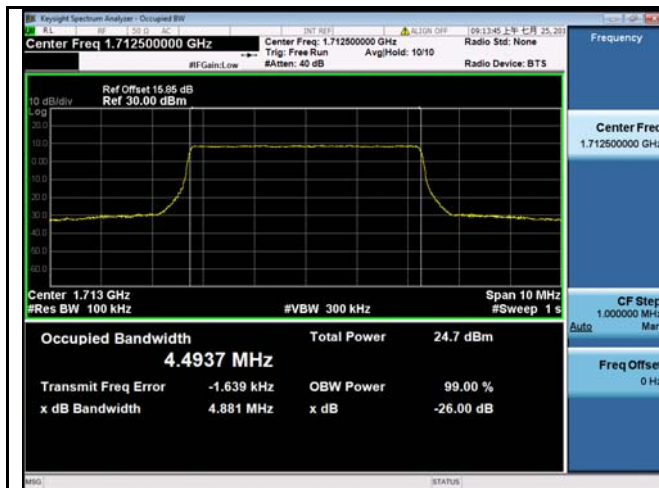
LTE band 66 - Low CH QPSK-5
