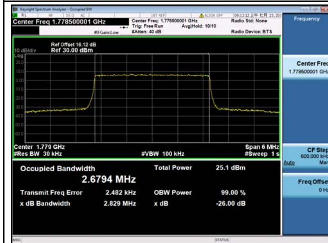
LTE band 66 - High CH QPSK-3
