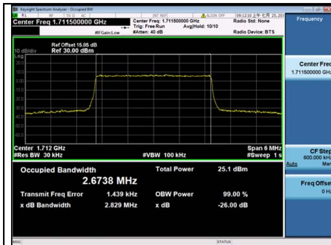
LTE band 66 - Low CH QPSK-3
