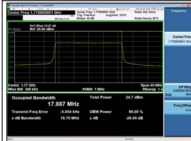
LTE band 66 - High CH QPSK-20
