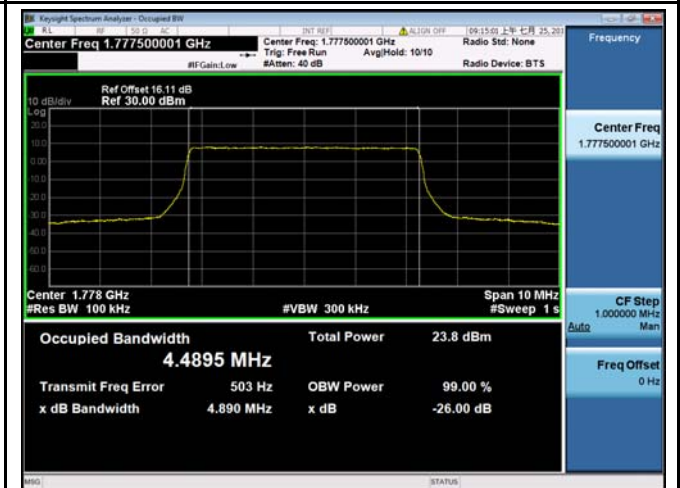
LTE band 66 - High CH 16QAM-5
