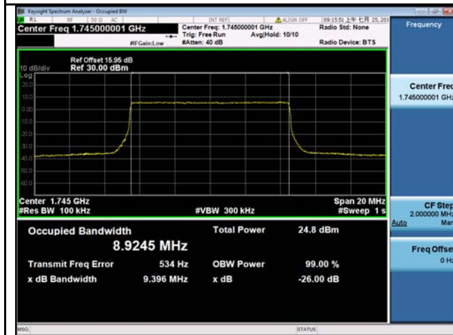
LTE band 66 - Middle CH QPSK-10
