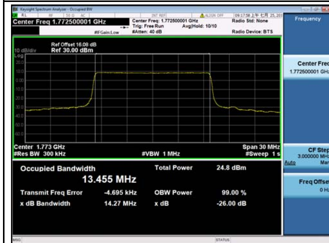
LTE band 66 - High CH QPSK-15
