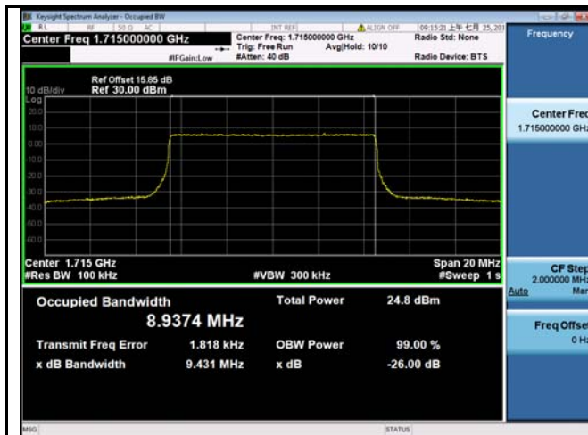
LTE band 66 - Low CH QPSK-10
