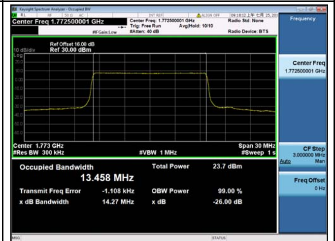
LTE band 66 - High CH 16QAM-15
