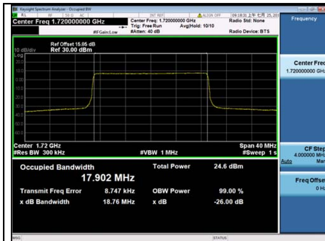
LTE band 66 - Low CH QPSK-20
