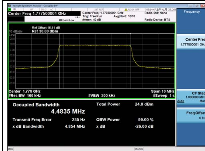
LTE band 66 - High CH QPSK-5
