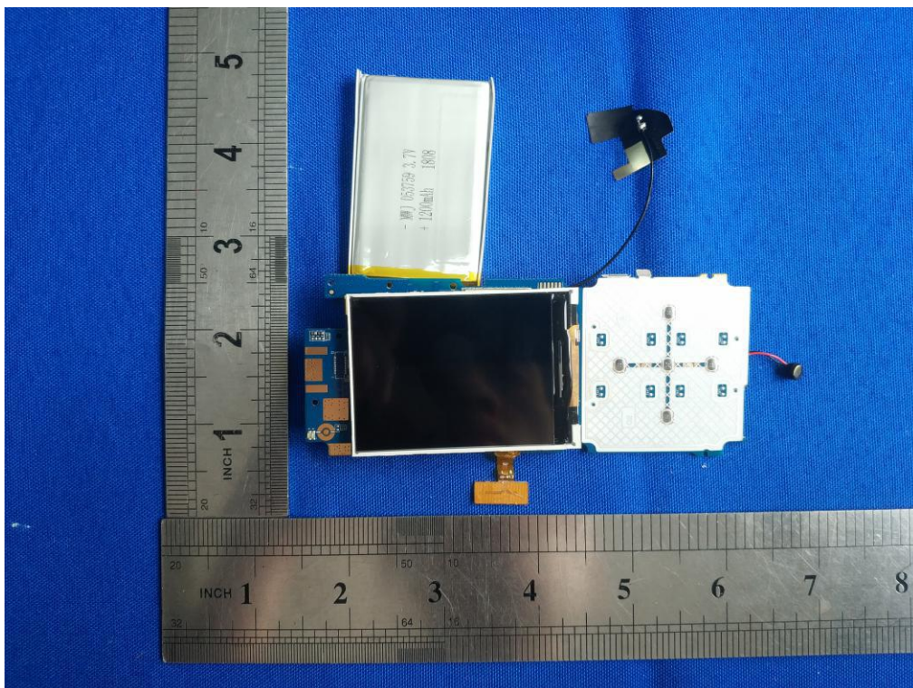
EUT – PCB View 7
