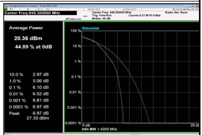
FDD05_1.4MHz_848.3_fullRB_Q16
