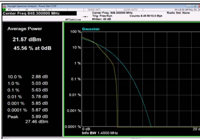
FDD05_1.4MHz_848.3_OneRB_high_Q16
