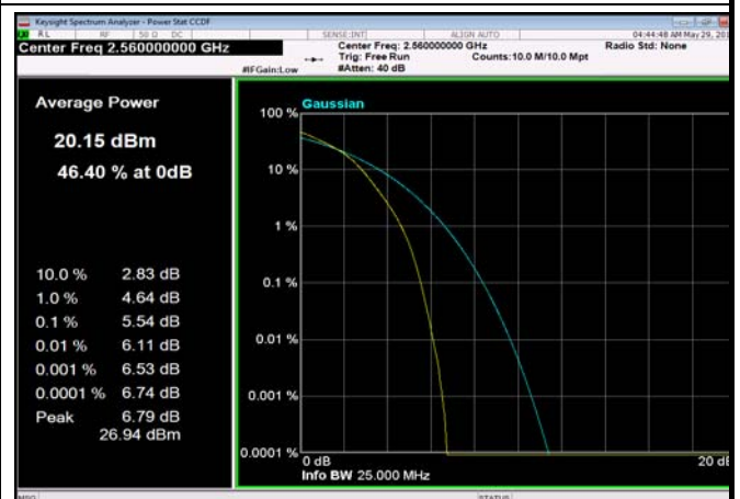
FDD07_20MHz_2560_fullRB_Q16
