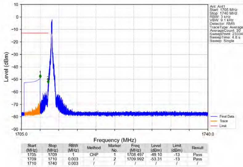
n66_15kHz_SISO_NTNV_30MHz_CP-OFDM_QPSK_1725MHz_Edge_1RB_Left
