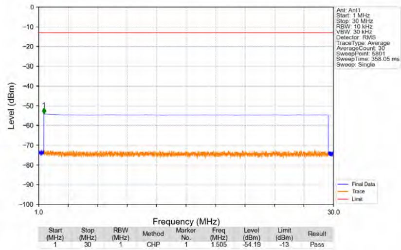
n66_15kHz_SISO_NTNV_25MHz_DFT-s-OFDM_QPSK_1722.5MHz_Edge_1RB_Left
