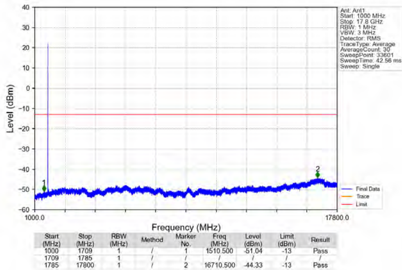
n66_15kHz_SISO_NTNV_40MHz_DFT-s-OFDM_PI/2_BPSK_1745MHz_Edge_1RB_Left
