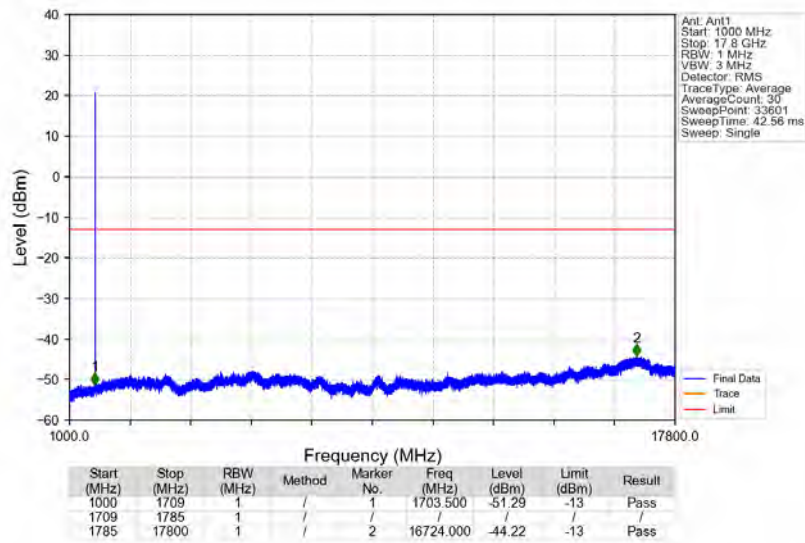
n66_15kHz_SISO_NTNV_40MHz_CP-OFDM_QPSK_1730MHz_Edge_1RB_Left
