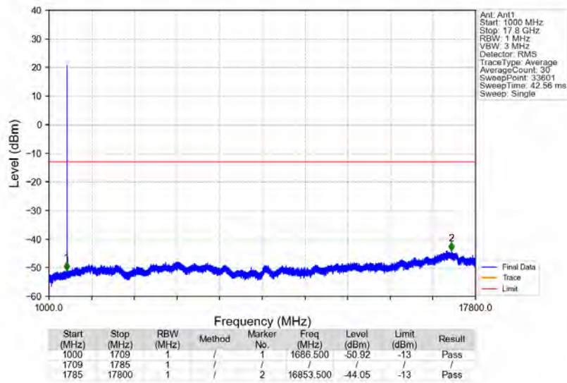
n66_15kHz_SISO_NTNV_40MHz_DFT-s-OFDM_QPSK_1730MHz_Edge_1RB_Left
