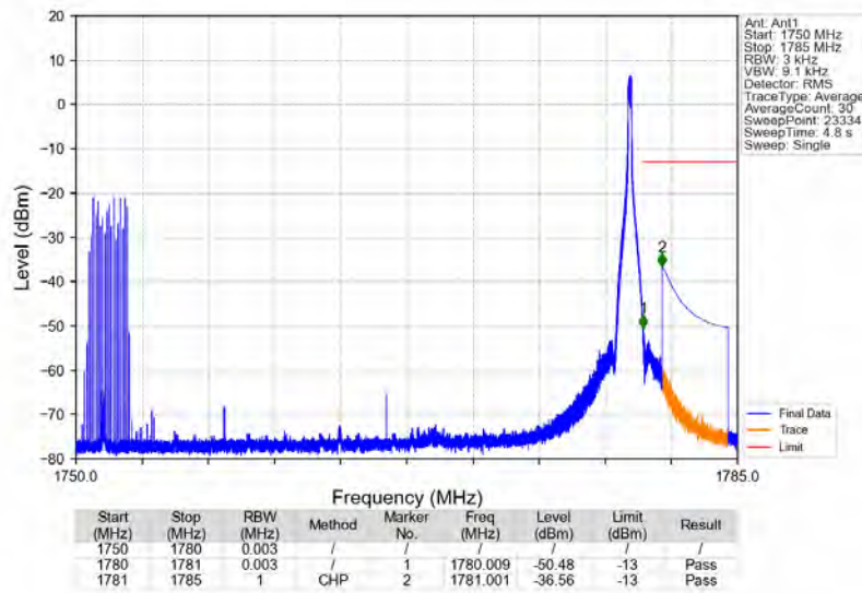
n66_15kHz_SISO_NTNV_30MHz_DFT-s-OFDM_PI/2_BPSK_1765MHz_Edge_1RB_Right
