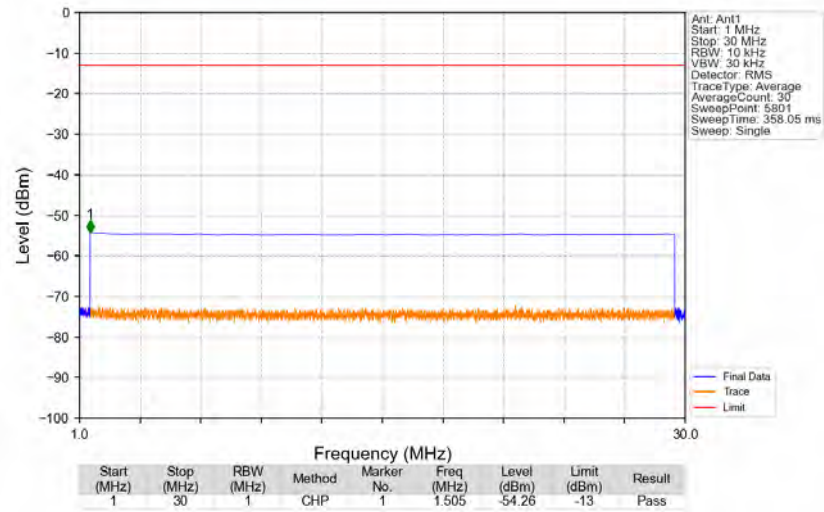
n66_15kHz_SISO_NTNV_40MHz_CP-OFDM QPSK_1760MHz_Edge_1RB_Right
