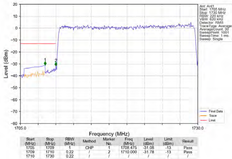
n66_15kHz_SISO_NTNV_20MHz_CP-OFDM_QPSK_1720MHz_Outer_Full
