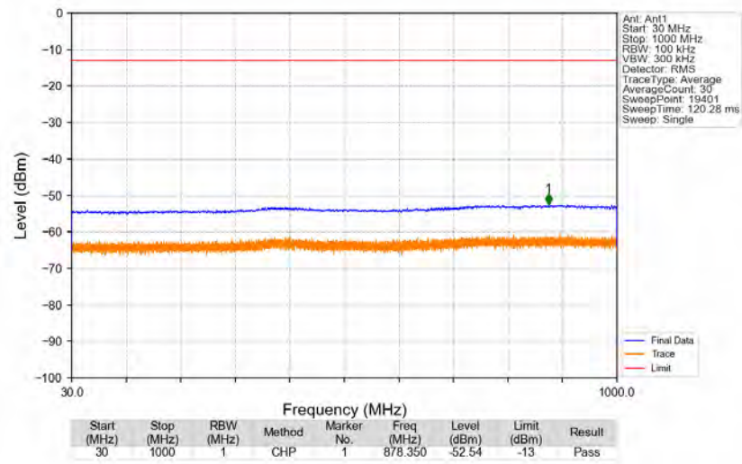
n66_15kHz_SISO_NTNV_25MHz_DFT-s-OFDM_PI/2_BPSK_1745MHz_Edge_1RB_Left
