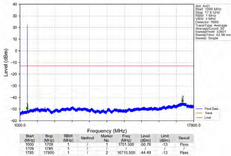
n66_15kHz_SISO_NTNV_40MHz_DFT-s-OFDM_PI/2_BPSK_1730MHz_Edge_1RB_Left
