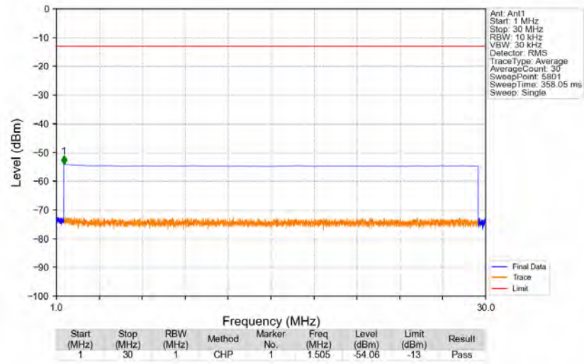
n66_15kHz_SISO_NTNV_40MHz_DFT-s-OFDM_QPSK_1730MHz_Edge_1RB_Left
