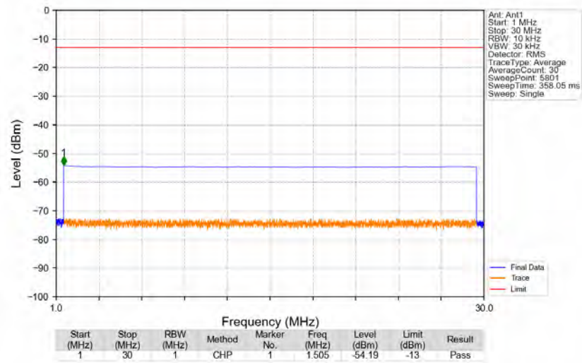
n66_15kHz_SISO_NTNV_40MHz_DFT-s-OFDM_QPSK_1760MHz_Edge_1RB_Right
