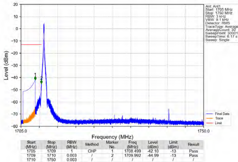
n66_15kHz_SISO_NTNV_40MHz_CP-OFDM_QPSK_1730MHz_Edge_1RB_Left
