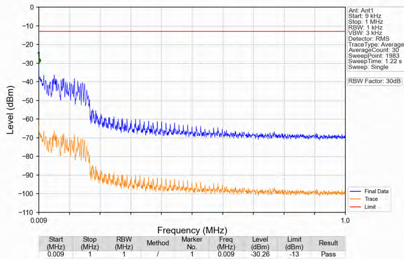
n66_15kHz_SISO_NTNV_30MHz_DFT-s-OFDM_QPSK_1725MHz_Edge_1RB_Left
