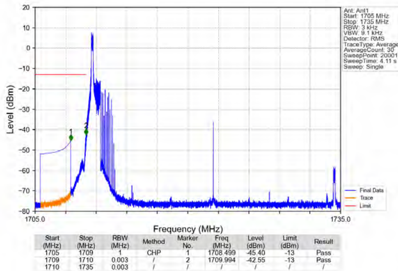
n66_15kHz_SISO_NTNV_25MHz_DFT-s-OFDM_QPSK_1722.5MHz_Edge_1RB_Left
