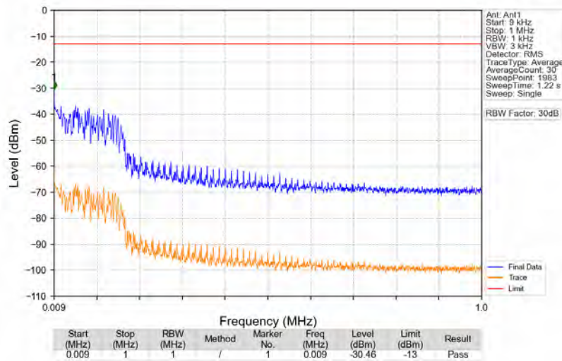
n66_15kHz_SISO_NTNV_40MHz_DFT-s-OFDM_QPSK_1730MHz_Edge_1RB_Left
