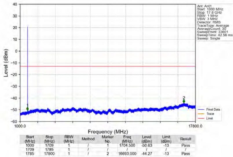
n66_15kHz_SISO_NTNV_30MHz_CP-OFDM_QPSK_1725MHz_Edge_1RB_Left
