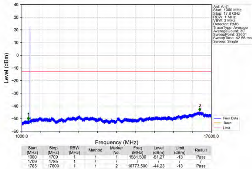
n66_15kHz_SISO_NTNV_40MHz_DFT-s-OFDM_QPSK_1745MHz_Edge_1RB_Left
