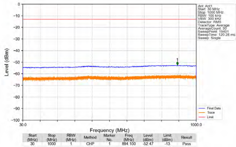
n66_15kHz_SISO_NTNV_40MHz_DFT-s-OFDM_PI/2_BPSK_1760MHz_Edge_1RB_Right
