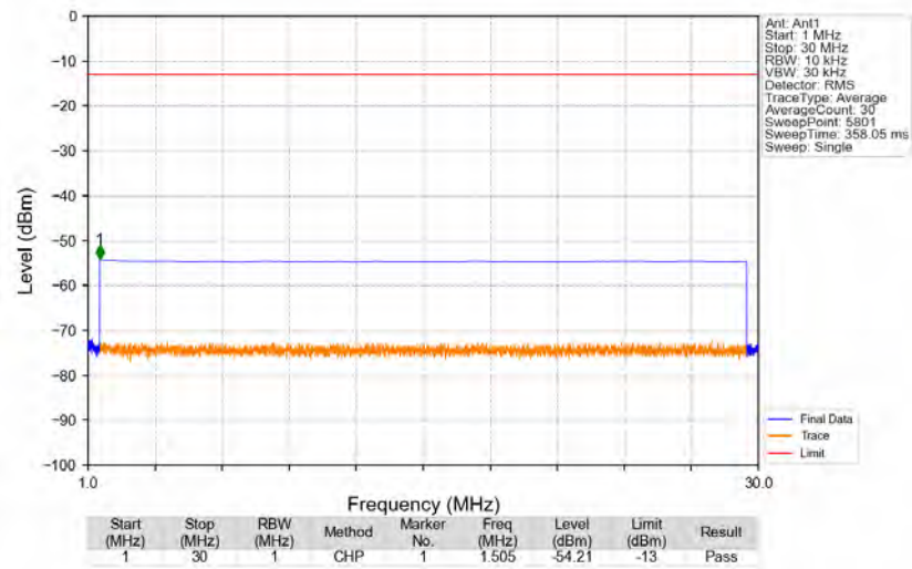
n66_15kHz_SISO_NTNV_30MHz_DFT-s-OFDM_PI/2_BPSK_1765MHz_Edge_1RB_Right
