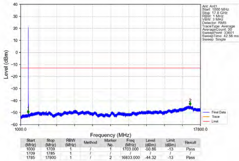
n66_15kHz_SISO_NTNV_25MHz_DFT-s-OFDM_QPSK_1722.5MHz_Edge_1RB_Left
