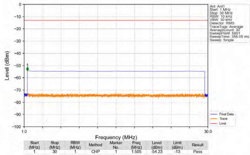
n66_15kHz_SISO_NTNV_25MHz_DFT-s-OFDM_QPSK_1745MHz_Edge_1RB_Left
