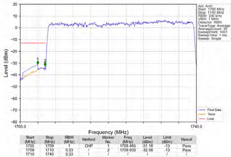
n66_15kHz_SISO_NTNV_30MHz_DFT-s-OFDM_PI/2_BPSK_1725MHz_Outer_Full
