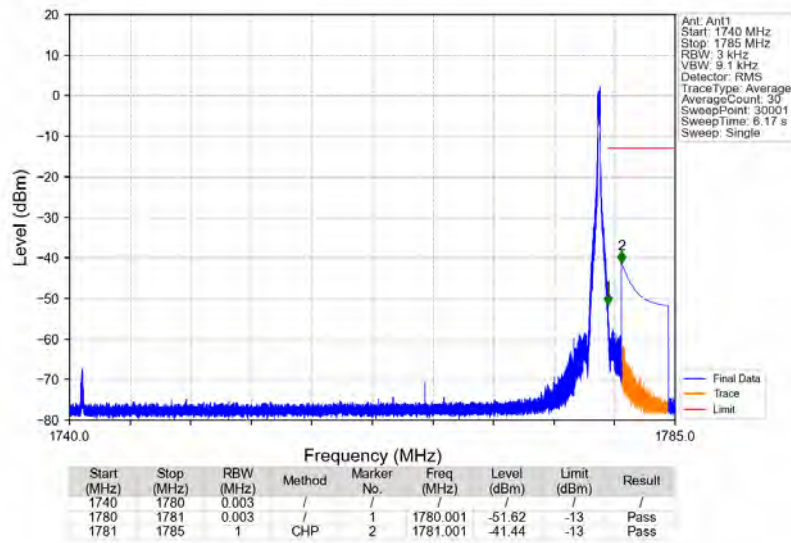
n66_15kHz_SISO_NTNV_40MHz_DFT-s-OFDM_PI/2_BPSK_1760MHz_Edge_1RB_Right
