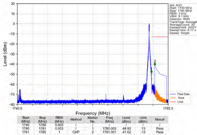
n66_15kHz_SISO_NTNV_40MHz_CP-OFDM_QPSK_1760MHz_Edge_1RB_Right
