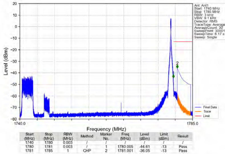
n66_15kHz_SISO_NTNV_40MHz_DFT-s-OFDM_QPSK_1760MHz_Edge_1RB_Right
