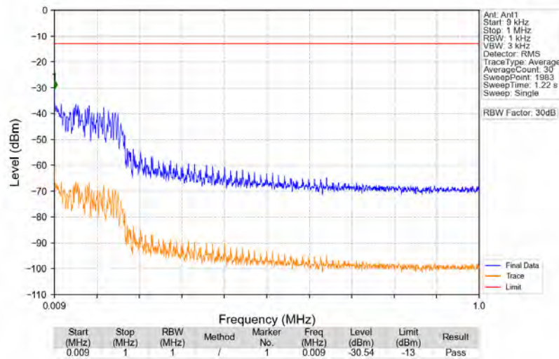
n66_15kHz_SISO_NTNV_40MHz_DFT-s-OFDM_QPSK_1760MHz_Edge_1RB_Right
