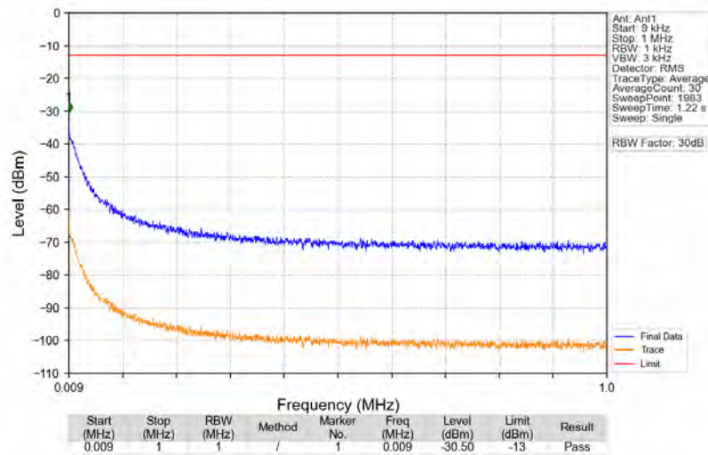
n66_15kHz_SISO_NTNV_25MHz_CP-OFDM_QPSK_1767.5MHz_Edge_1RB_Right
