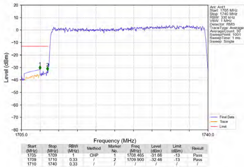
n66_15kHz_SISO_NTNV_30MHz_CP-OFDM_QPSK_1725MHz_Outer_Full
