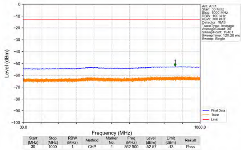
n66_15kHz_SISO_NTNV_30MHz_DFT-s-OFDM_QPSK_1765MHz_Edge_1RB_Right
