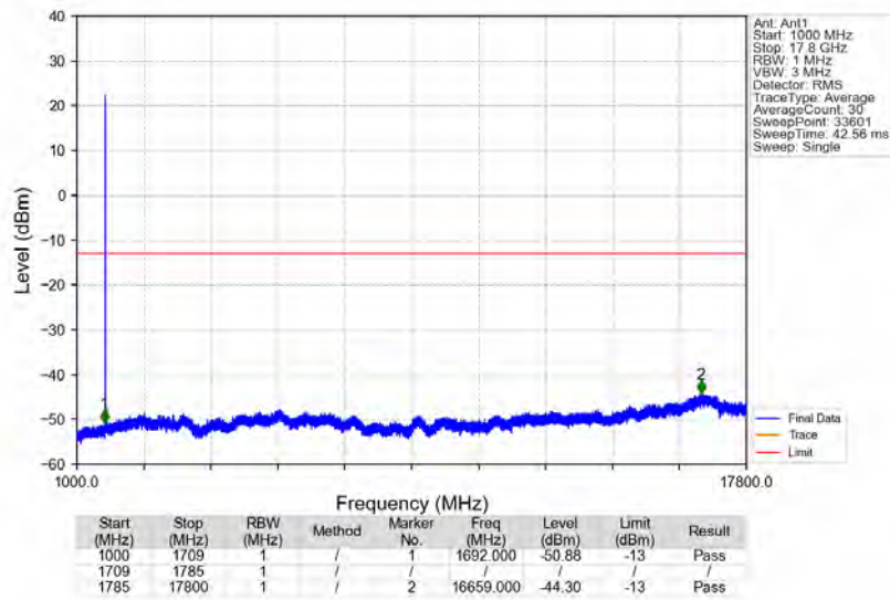
n66_15kHz_SISO_NTNV_30MHz_DFT-s-OFDM_PI/2_BPSK_1725MHz_Edge_1RB_Left
