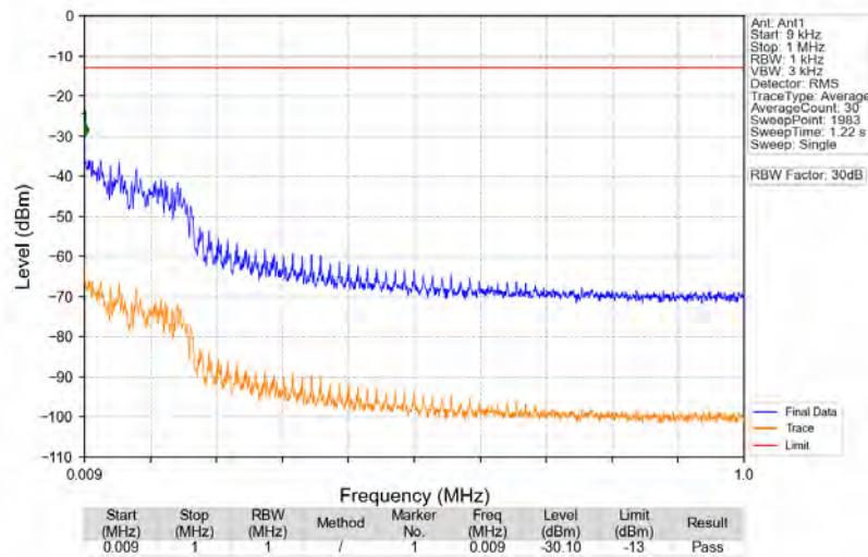
n66_15kHz_SISO_NTNV_30MHz_CP-OFDM_QPSK_1765MHz_Edge_1RB_Right
