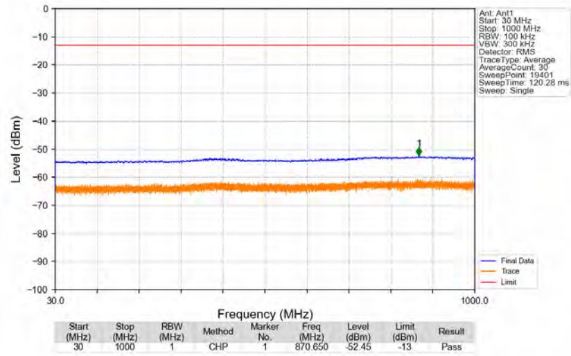
n66_15kHz_SISO_NTNV_40MHz_CP-OFDM_QPSK_1745MHz_Edge_1RB_Left
