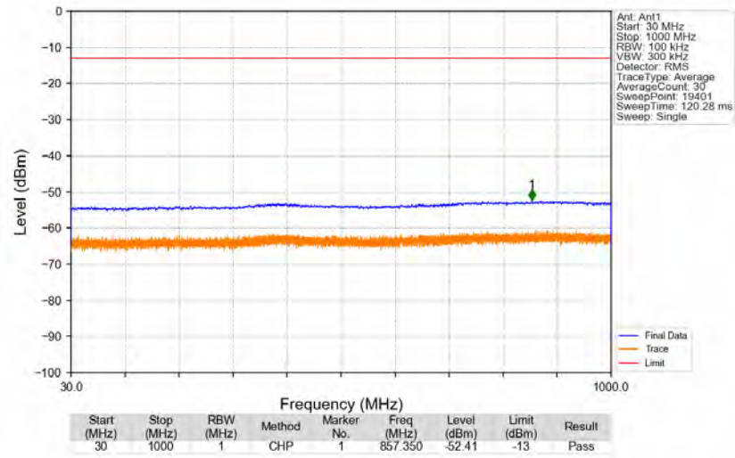
n66_15kHz_SISO_NTNV_20MHz_CP-OFDM_QPSK_1745MHz_Edge_1RB_Left
