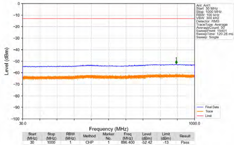
n66_15kHz_SISO_NTNV_25MHz_CP-OFDM_QPSK_1722.5MHz_Edge_1RB_Left
