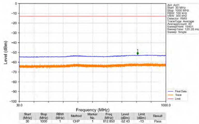
n66_15kHz_SISO_NTNV_30MHz_DFT-s-OFDM_QPSK_1725MHz_Edge_1RB_Left
