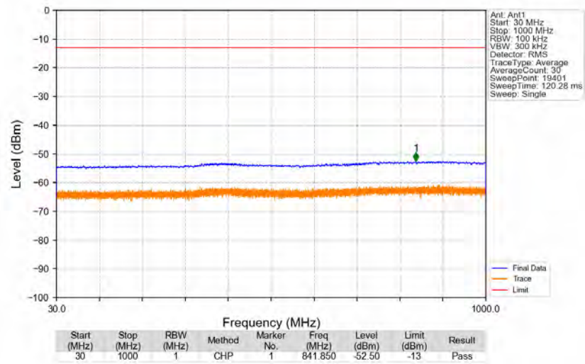
n66_15kHz_SISO_NTNV_20MHz_DFT-s-OFDM_QPSK_1770MHz_Edge_1RB_Right
