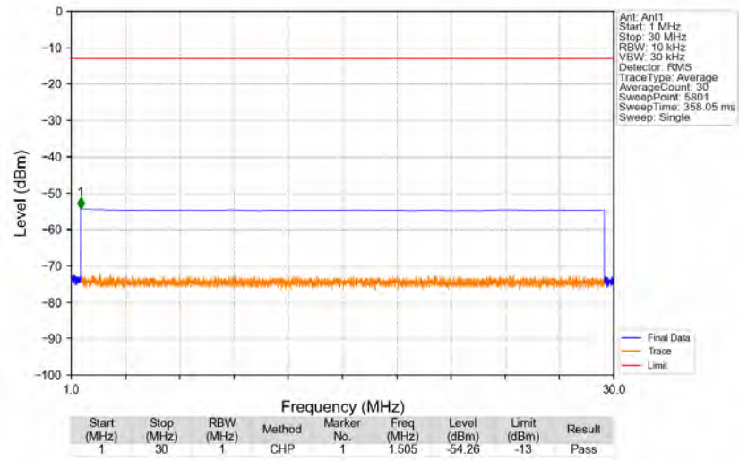
n66_15kHz_SISO_NTNV_40MHz_CP-OFDM_QPSK_1730MHz_Edge_1RB_Left
