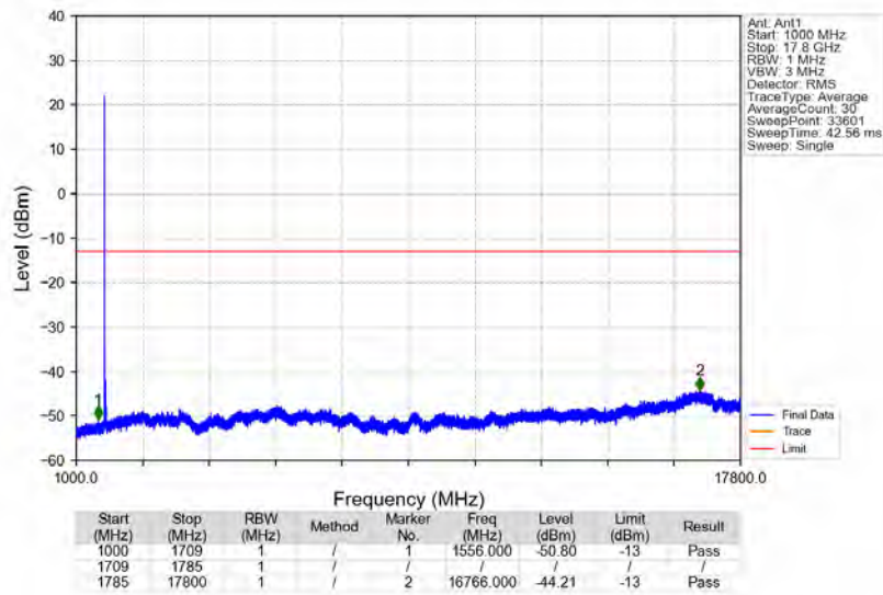
n66_15kHz_SISO_NTNV_25MHz_DFT-s-OFDM_PI/2_BPSK_1722.5MHz_Edge_1RB_Left
