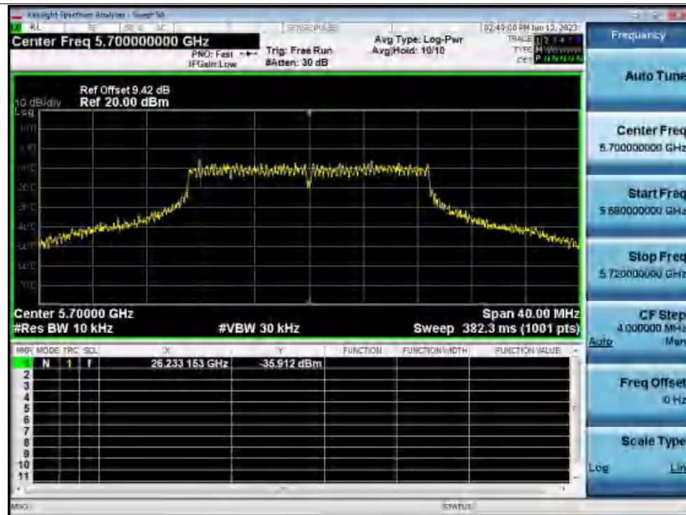
Freq. Stability 20C 102V ac20 5700MHz Ant1 0 Minutes
