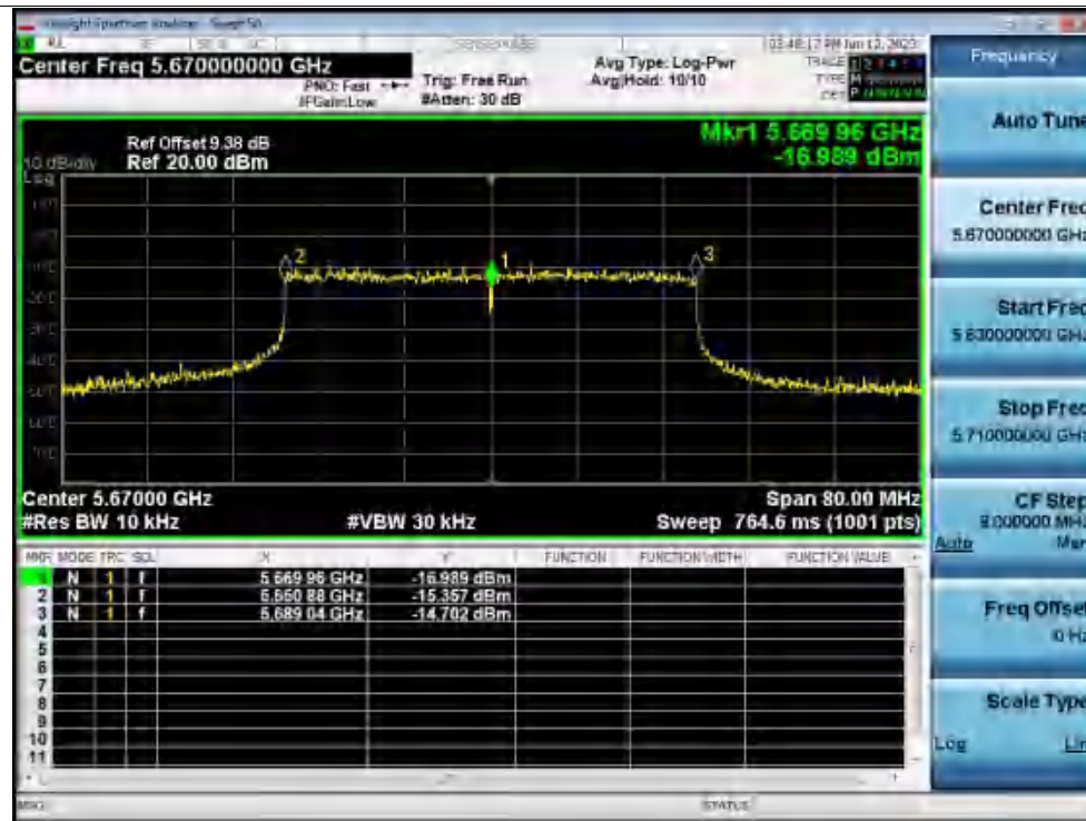
Freq. Stability 50C 120V ax40 5670MHz Ant1 0 Minutes
