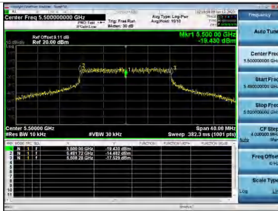
Freq. Stability -20C 120V a 5500MHz Ant1 0 Minutes
