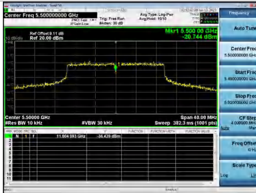
Freq. Stability 20C 120V ax20 5500MHz Ant1 0 Minutes
