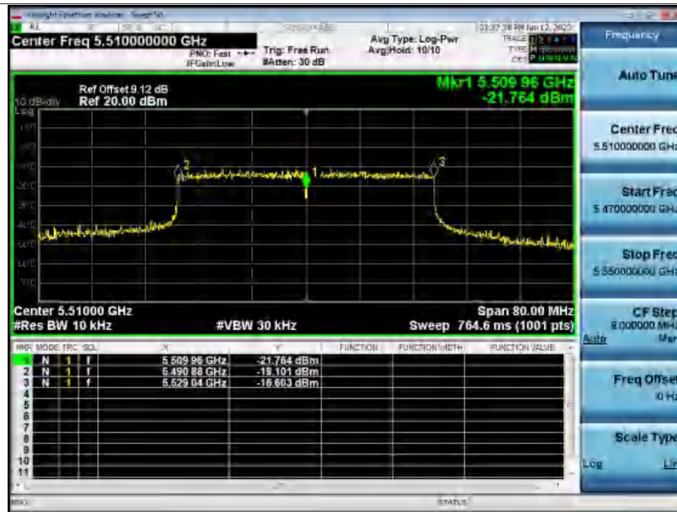
Freq. Stability 0C 120V ax40 5510MHz Ant1 0 Minutes
