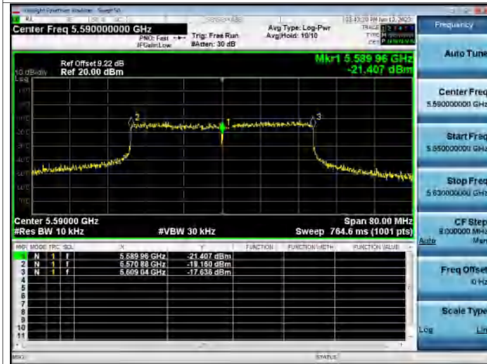
Freq. Stability 0C 120V ax40 5590MHz Ant1 0 Minutes
