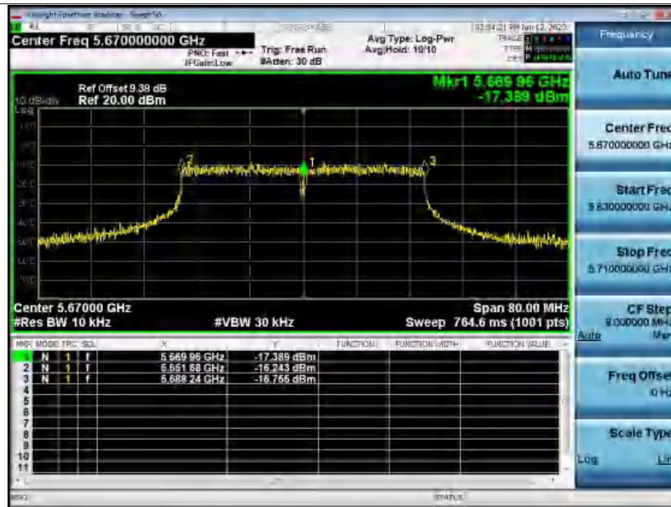
Freq. Stability 30C 120V ac40 5670MHz Ant1 0 Minutes
