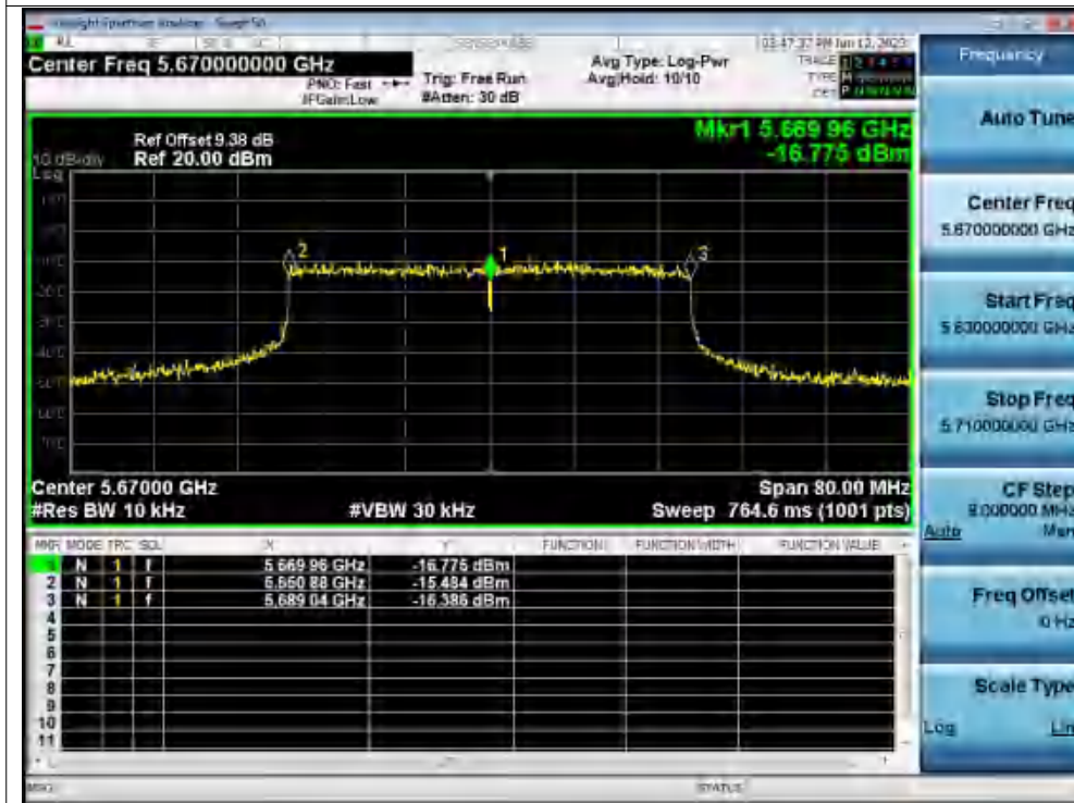
Freq. Stability 0C 120V ax40 5670MHz Ant1 0 Minutes
