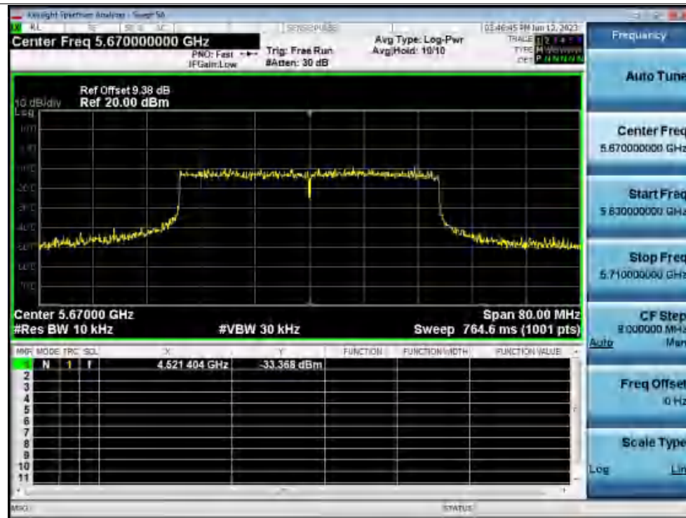
Freq. Stability 20C 120V ax40 5670MHz Ant1 0 Minutes
