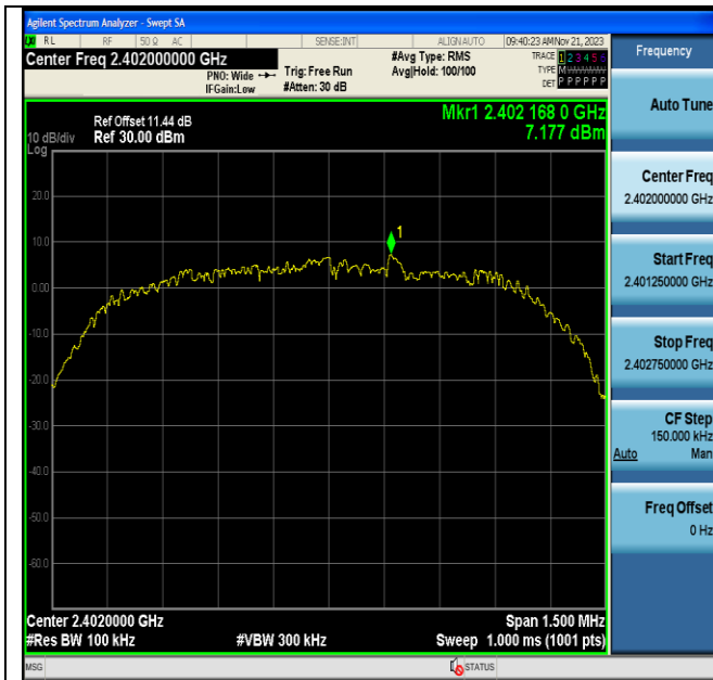
3DH5-Ant6-2402-0-Reference-PASS
