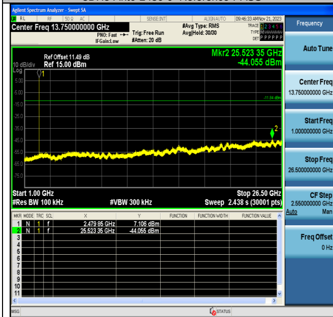
3DH5-Ant6-2480-1000~26500-PASS
