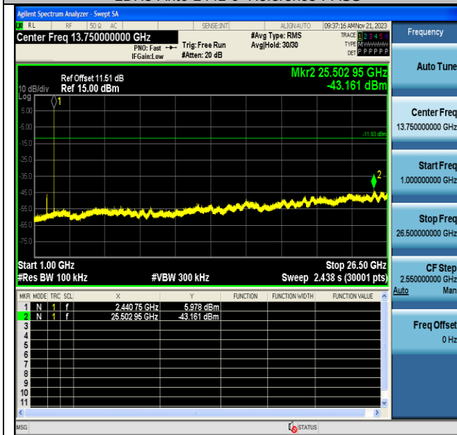
2DH5-Ant6-2441-1000-26500-PASS
