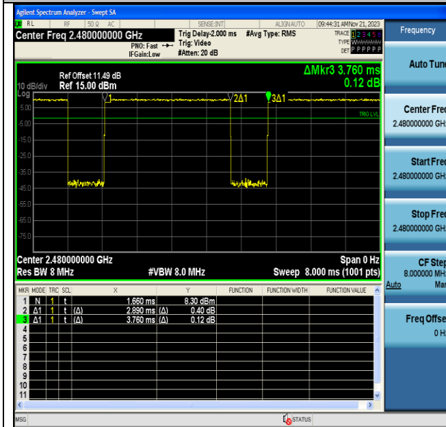
NTNV-3DH5-Ant6-2480
