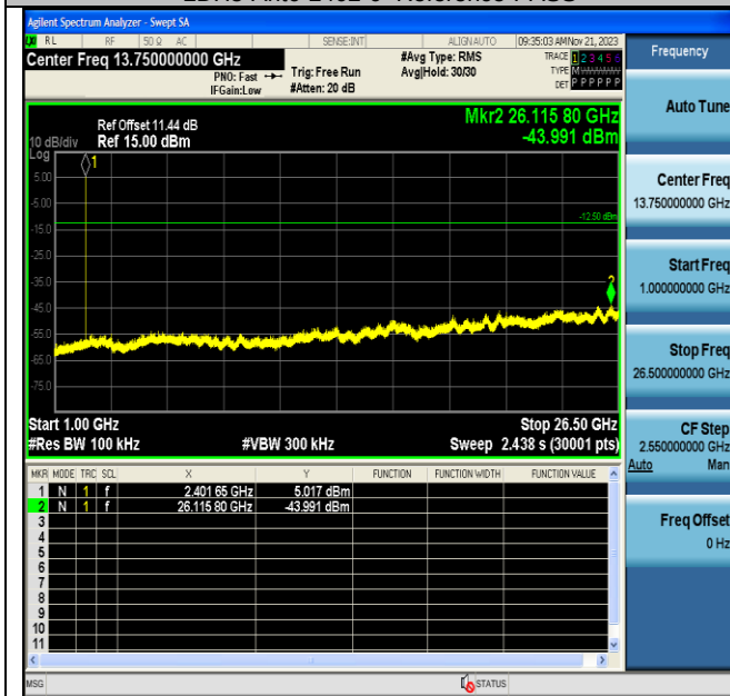
2DH5-Ant6-2402-1000-26500-PASS
