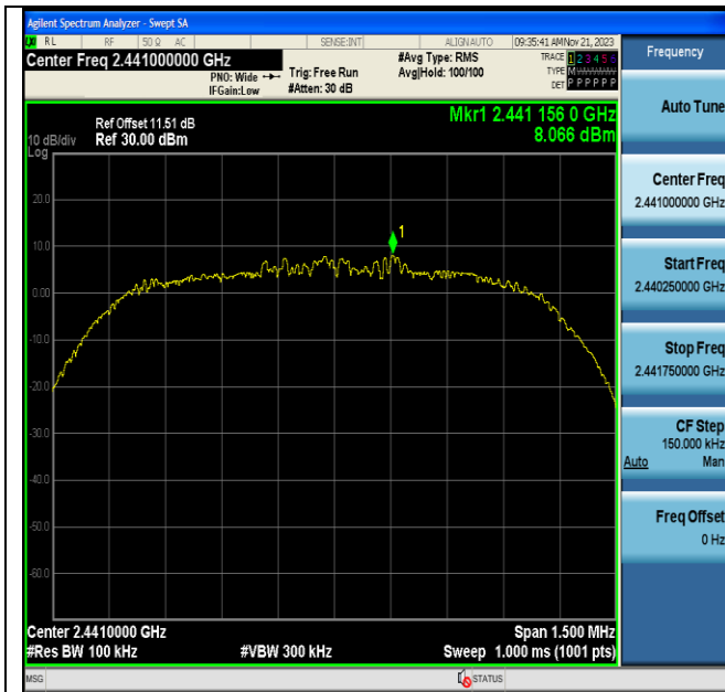
2DH5-Ant6-2441-0-Reference-PASS
