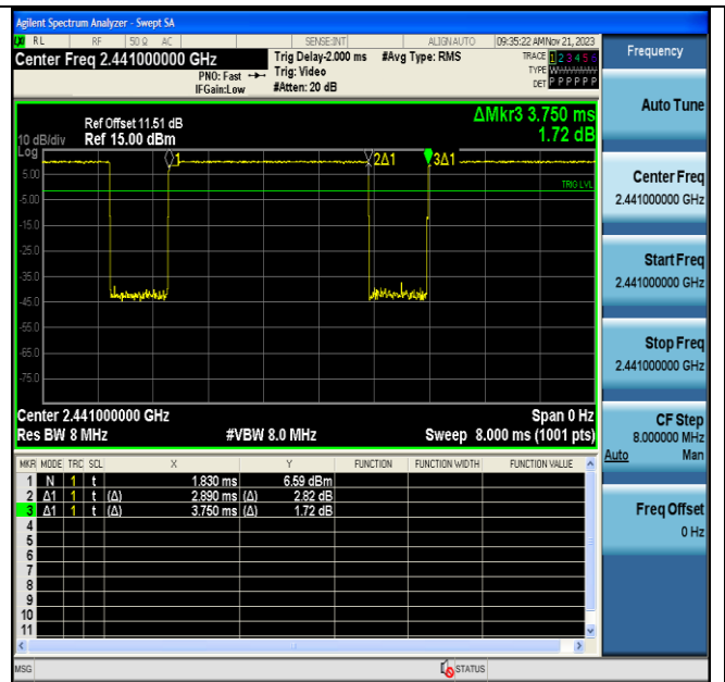
NTNV-2DH5-Ant6-2441
