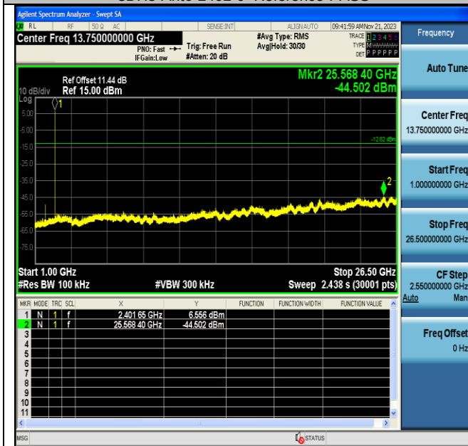
3DH5-Ant6-2402-1000-26500-PASS
