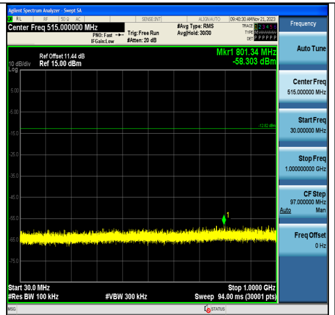
3DH5-Ant6-2402-30-1000-PASS
