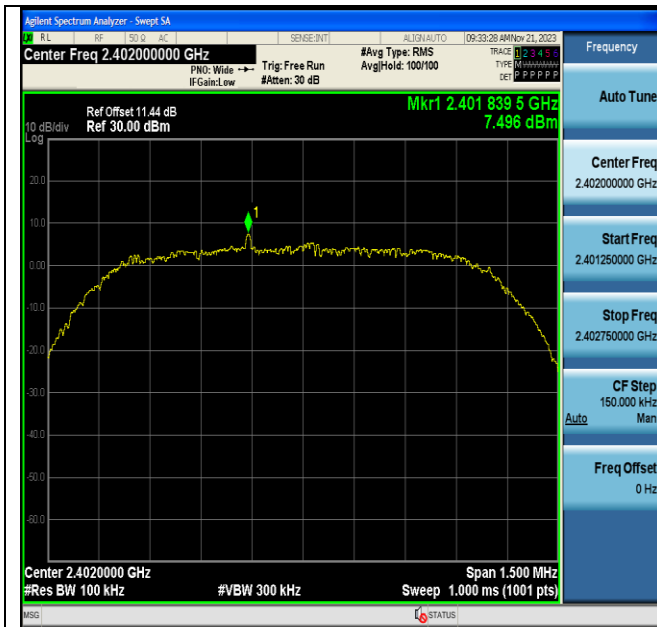
2DH5-Ant6-2402-0-Reference-PASS
