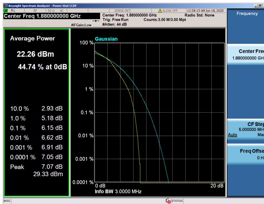
LTE Band 2 / 3 MHz / 16QAM - RB Size 15
