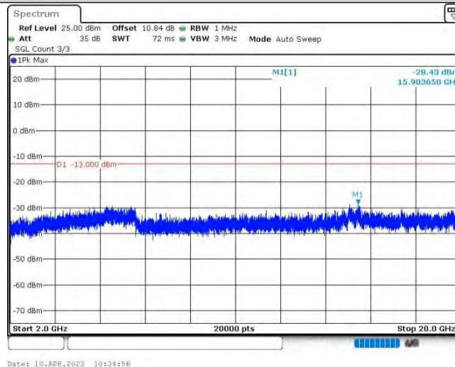
Band25-5MHz-16QAM-26365-1RB#0-Range3:2000~20000MHz
