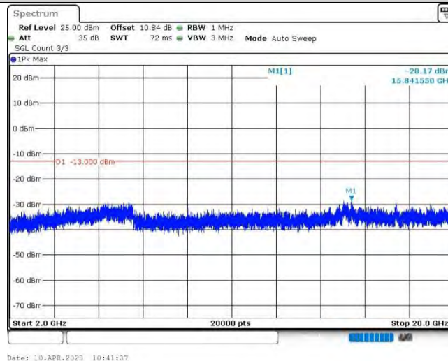
Band25-20MHz-QPSK-26140-1RB#0-Range3:2000~20000MHz
