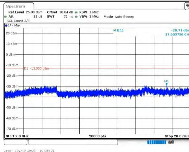
Band25-5MHz-QPSK-26665-1RB#0-Range3:2000~20000MHz
