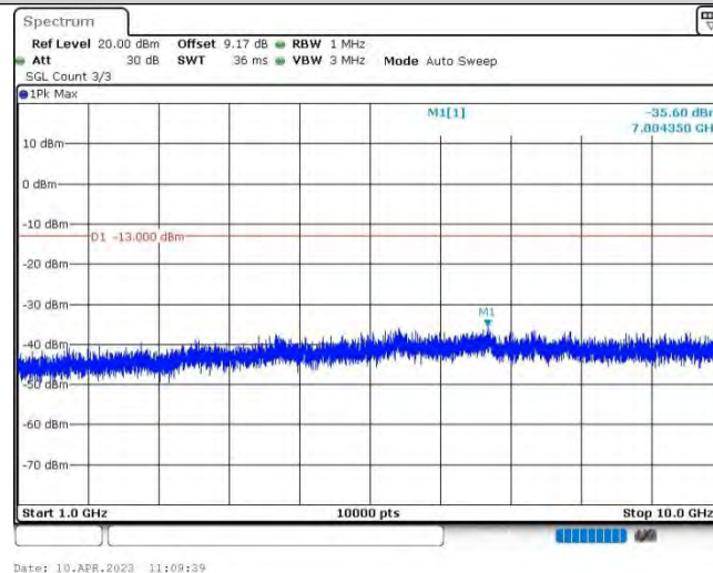
Band26@22-15MHz-QPSK-26765-1RB#0-Range2:1000~10000MHz
