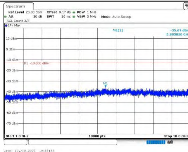
Band26@22-3MHz-QPSK-26775-1RB#0-Range2:1000~10000MHz
