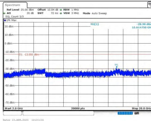
Band25-3MHz-QPSK-26055-1RB#0-Range3:2000~20000MHz
