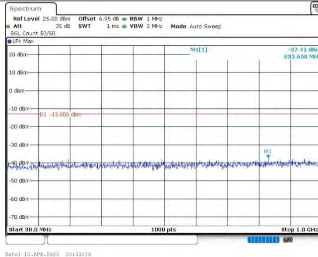
Band25-20MHz-QPSK-26590-1RB#0-Range1:30~1000MHz
