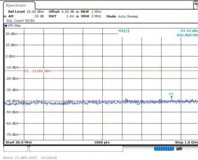
Band25-5MHz-16QAM-26365-1RB#0-Range1:30~1000MHz
