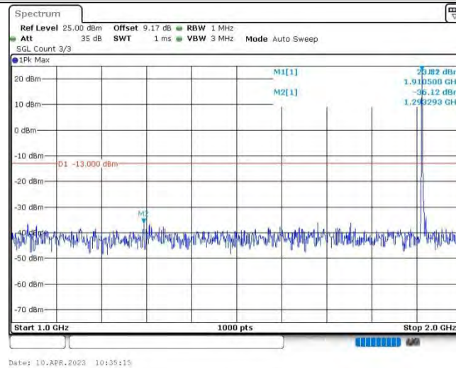
Band25-5MHz-QPSK-26665-1RB#0-Range2:1000~2000MHz
