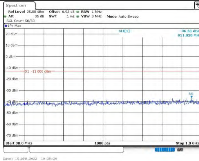
Band25-5MHz-16QAM-26665-1RB#0-Range1:30~1000MHz
