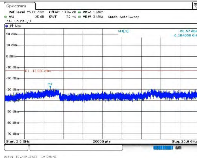
Band25-10MHz-16QAM-26090-1RB#0-Range3:2000~20000MHz
