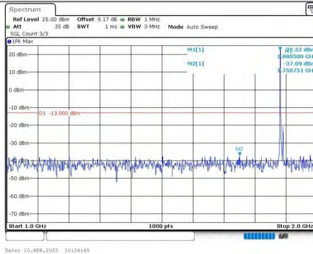
Band25-5MHz-16QAM-26365-1RB#0-Range2:1000~2000MHz
