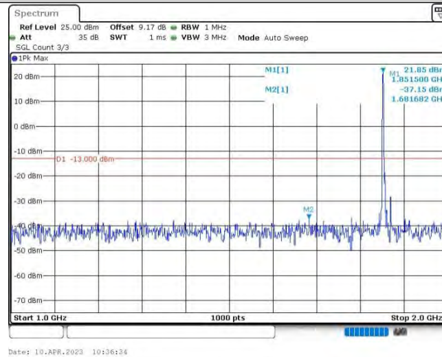
Band25-10MHz-16QAM-26090-1RB#0-Range2:1000~2000MHz
