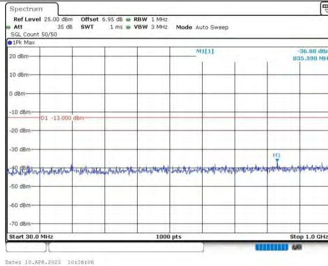
Band25-10MHz-QPSK-26090-1RB#0-Range1:30~1000MHz
