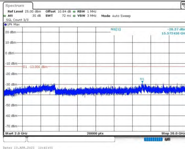
Band25-15MHz-16QAM-26615-1RB#0-Range3:2000~20000MHz
