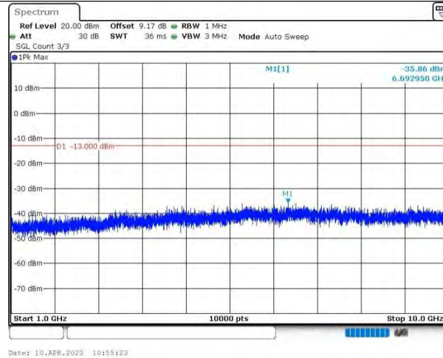
Band26@22-3MHz-QPSK-26740-1RB#0-Range2:1000~10000MHz
