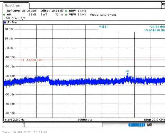
Band25-15MHz-QPSK-26115-1RB#0-Range3:2000~20000MHz
