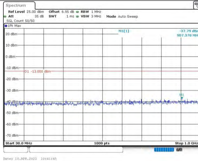
Band25-20MHz-16QAM-26140-1RB#0-Range1:30~1000MHz
