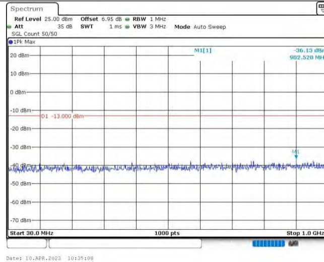
Band25-5MHz-QPSK-26665-1RB#0-Range1:30~1000MHz
