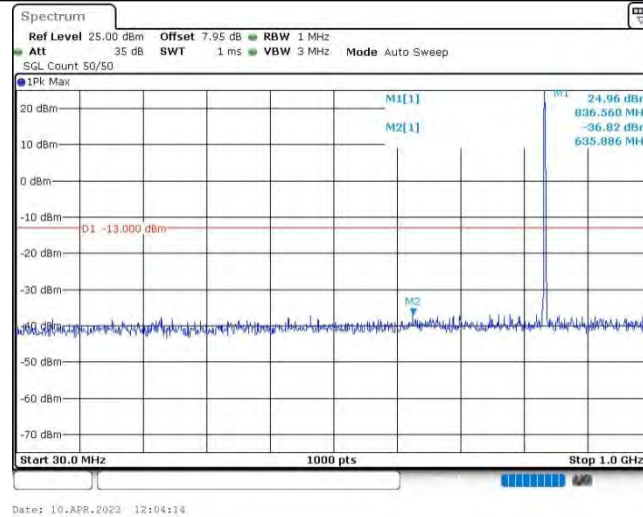
Band26@90-1.4MHz-QPSK-26915-1RB#0-Range1:30~1000MHz
