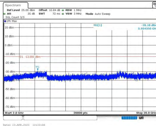
Band25-3MHz-QPSK-26675-1RB#0-Range3:2000~20000MHz
