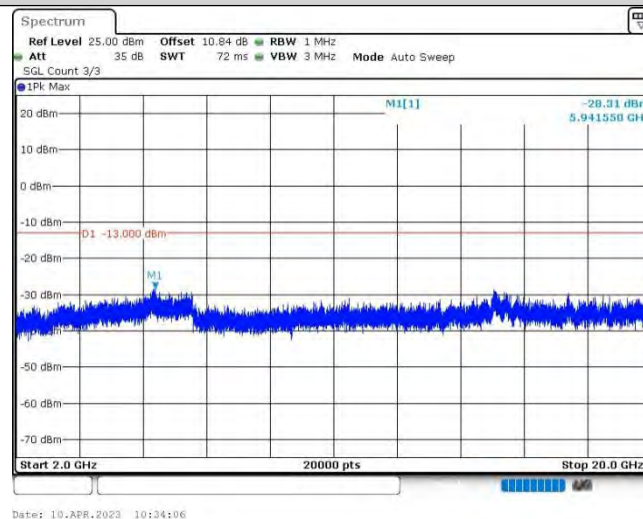
Band25-5MHz-16QAM-26065-1RB#0-Range3:2000~20000MHz
