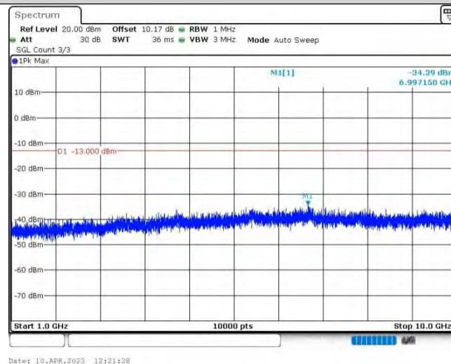
Band26@90-10MHz-QPSK-26915-1RB#0-Range2:1000~10000MHz
