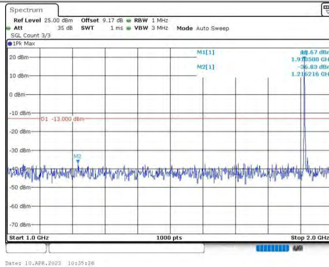
Band25-5MHz-16QAM-26665-1RB#0-Range2:1000~2000MHz
