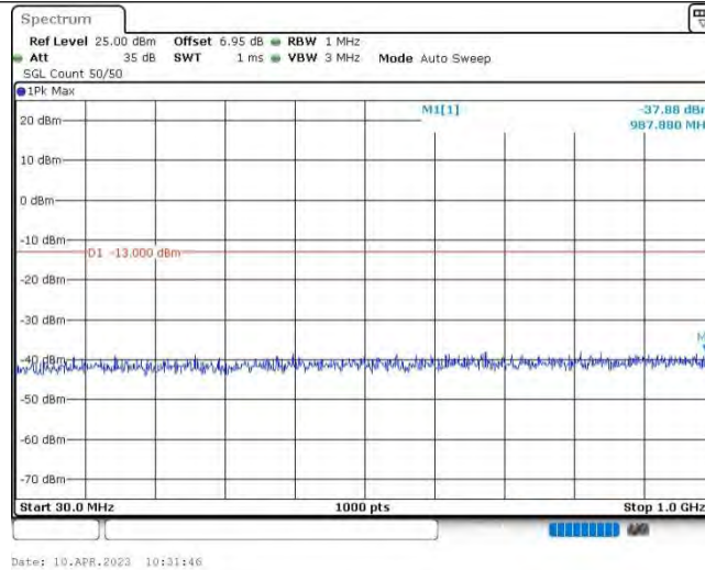
Band25-3MHz-QPSK-26365-1RB#0-Range1:30~1000MHz
