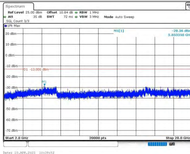
Band25-15MHz-QPSK-26365-1RB#0-Range3:2000~20000MHz
