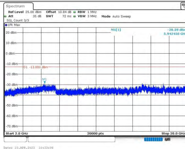
Band25-3MHz-16QAM-26675-1RB#0-Range3:2000~20000MHz
