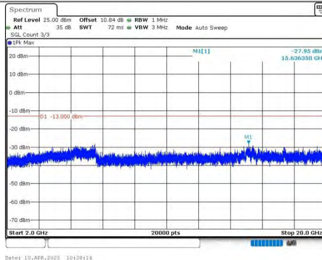
Band25-10MHz-16QAM-26640-1RB#0-Range3:2000~20000MHz
