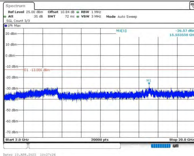
Band25-10MHz-16QAM-26365-1RB#0-Range3:2000~20000MHz
