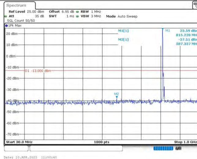
Band26@22-5MHz-16QAM-26715-1RB#0-Range1:30~1000MHz
