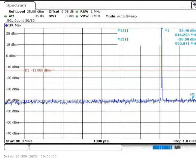
Band26@22-3MHz-16QAM-26705-1RB#0-Range1:30~1000MHz
