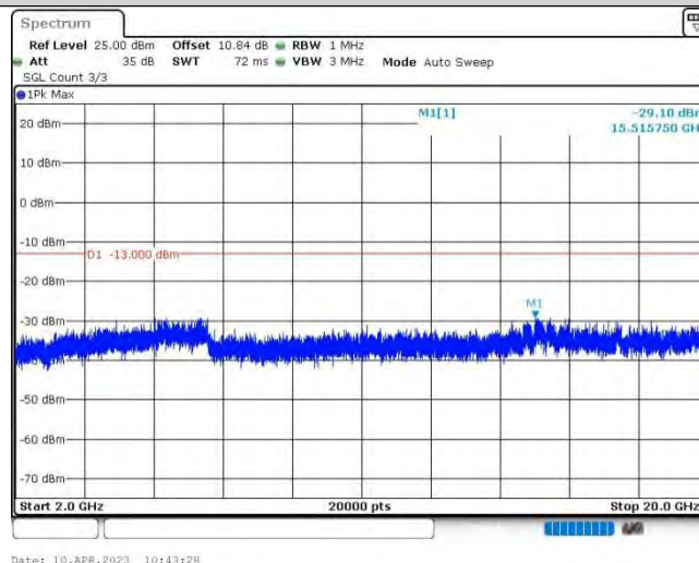
Band25-20MHz-QPSK-26590-1RB#0-Range3:2000~20000MHz
