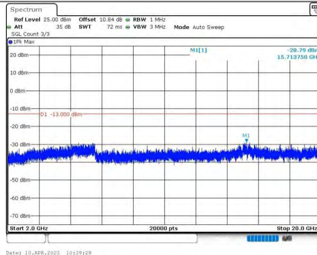
Band25-15MHz-16QAM-26115-1RB#0-Range3:2000~20000MHz
