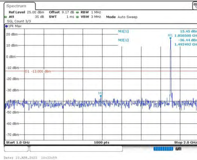
Band25-5MHz-16QAM-26065-1RB#0-Range2:1000~2000MHz
