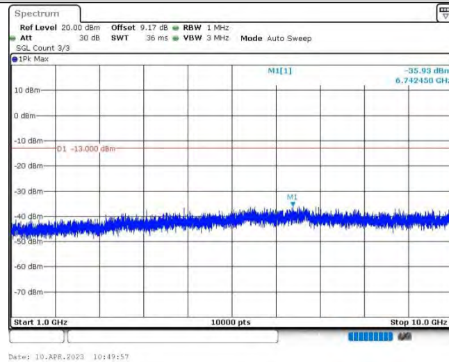
Band26@22-1.4MHz-QPSK-26697-1RB#0-Range2:1000~10000MHz
