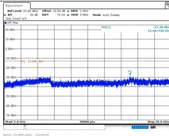
Band25-20MHz-16QAM-26365-1RB#0-Range3:2000~20000MHz
