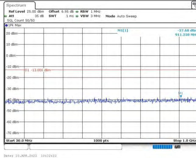
Band25-3MHz-QPSK-26675-1RB#0-Range1:30~1000MHz
