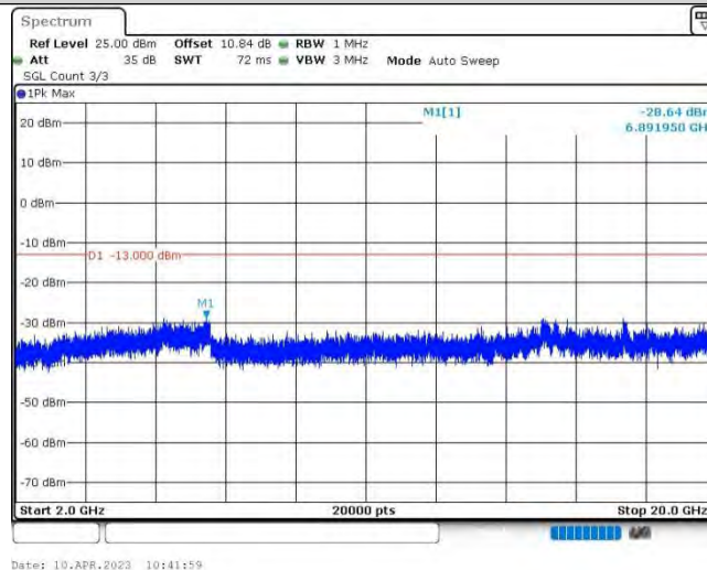
Band25-20MHz-16QAM-26140-1RB#0-Range3:2000~20000MHz
