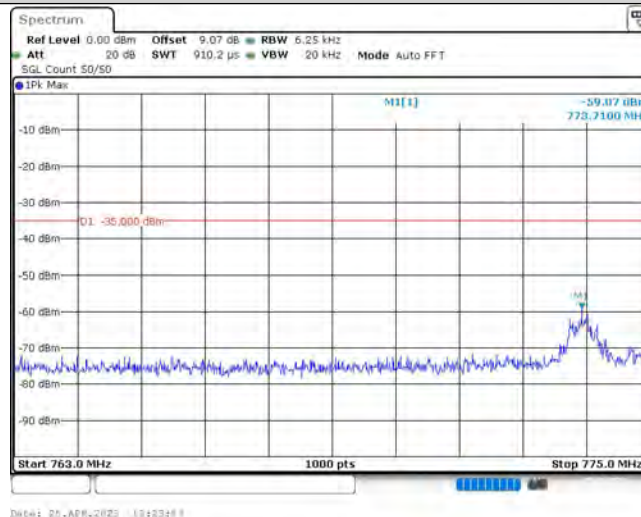
Band13-5MHz-QPSK-23255-1RB#0-Range1:763~775MHz
