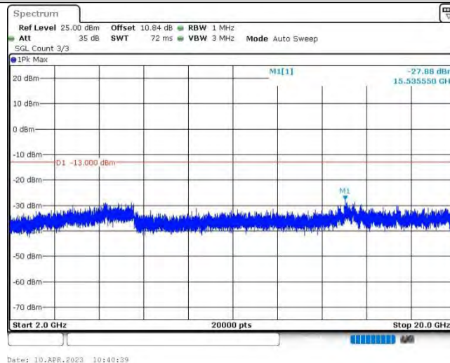
Band25-15MHz-QPSK-26615-1RB#0-Range3:2000~20000MHz
