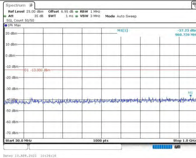
Band25-5MHz-QPSK-26365-1RB#0-Range1:30~1000MHz
