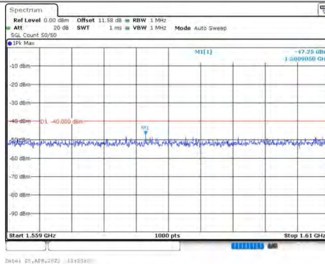
Band13-5MHz-QPSK-23230-1RB#0-Range3:1559~1610MHz
