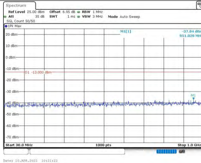
Band25-3MHz-16QAM-26055-1RB#0-Range1:30~1000MHz
