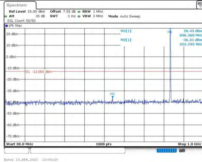
Band26@90-1.4MHz-16QAM-26915-1RB#0-Range1:30~1000MHz
