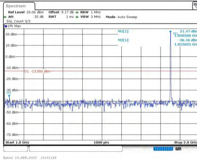
Band25-3MHz-16QAM-26055-1RB#0-Range2:1000~2000MHz
