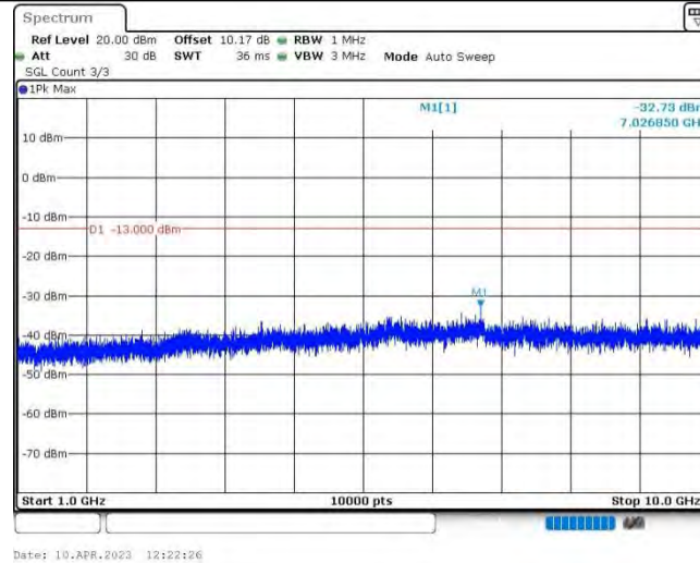
Band26@90-10MHz-16QAM-26990-1RB#0-Range2:1000~10000MHz
