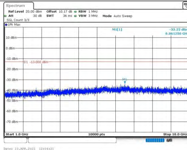
Band26@90-1.4MHz-QPSK-26915-1RB#0-Range2:1000~10000MHz
