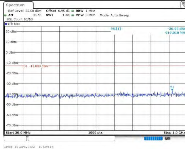
Band25-15MHz-16QAM-26115-1RB#0-Range1:30~1000MHz
