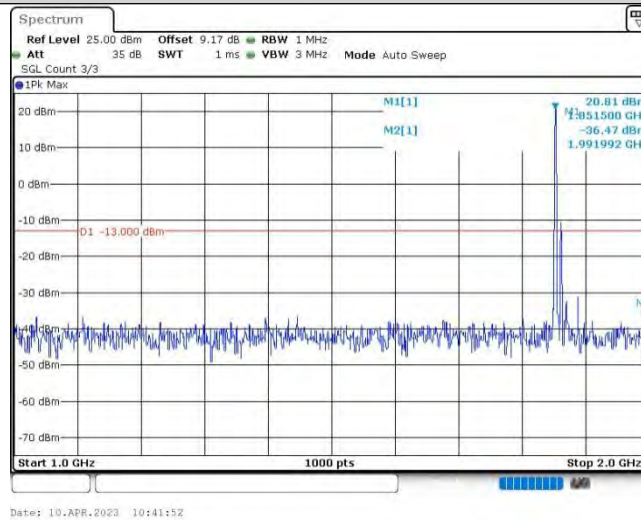
Band25-20MHz-16QAM-26140-1RB#0-Range2:1000~2000MHz
