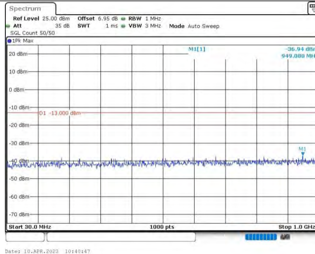
Band25-15MHz-16QAM-26615-1RB#0-Range1:30~1000MHz
