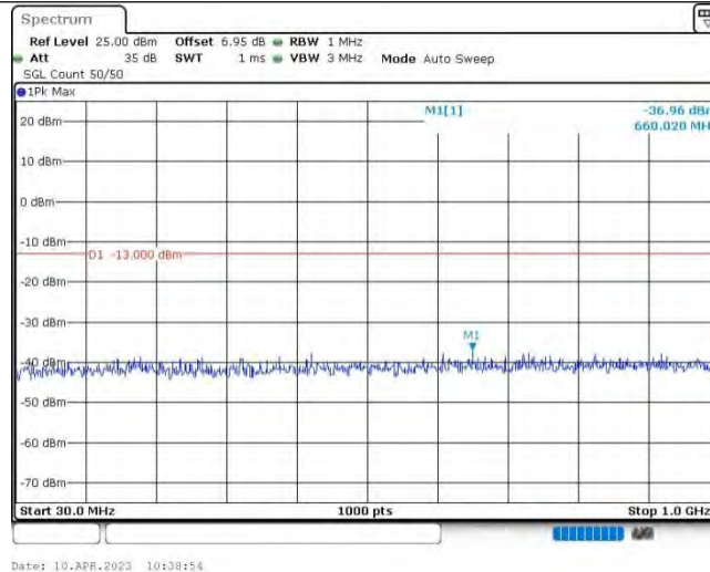
Band25-15MHz-QPSK-26115-1RB#0-Range1:30~1000MHz
