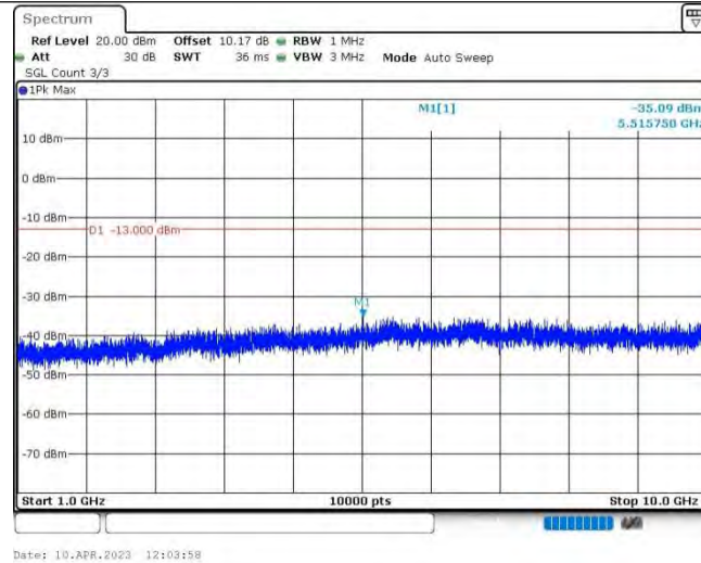
Band26@90-1.4MHz-16QAM-26797-1RB#0-Range2:1000~10000MHz
