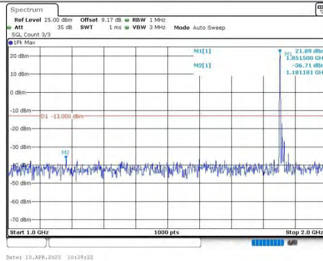
Band25-15MHz-16QAM-26115-1RB#0-Range2:1000~2000MHz
