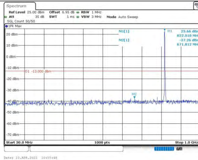
Band26@22-3MHz-QPSK-26775-1RB#0-Range1:30~1000MHz
