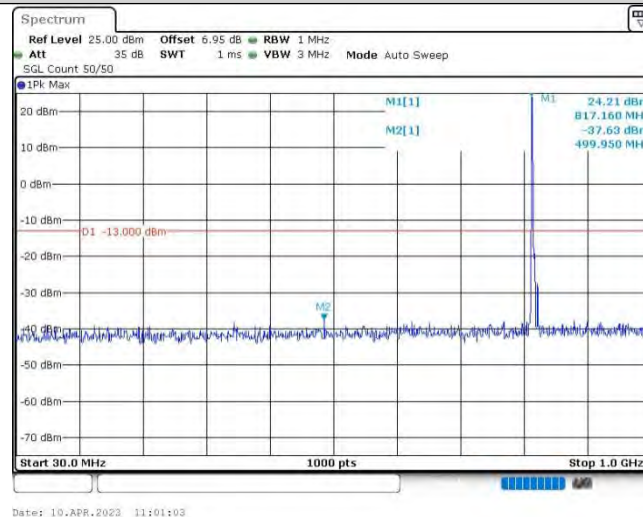
Band26@22-5MHz-QPSK-26740-1RB#0-Range1:30~1000MHz
