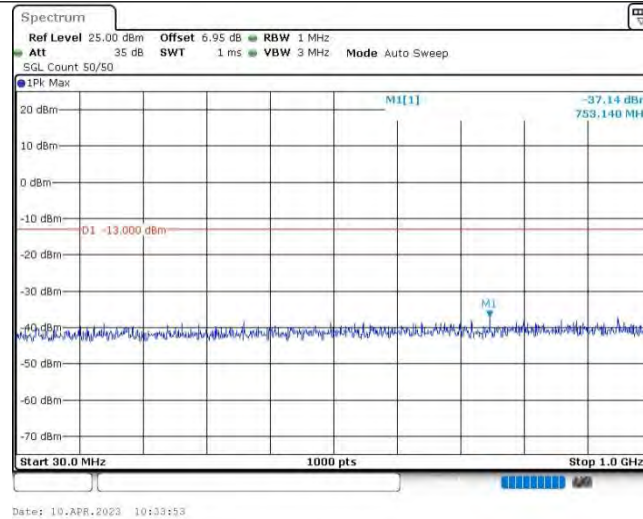
Band25-5MHz-16QAM-26065-1RB#0-Range1:30~1000MHz
