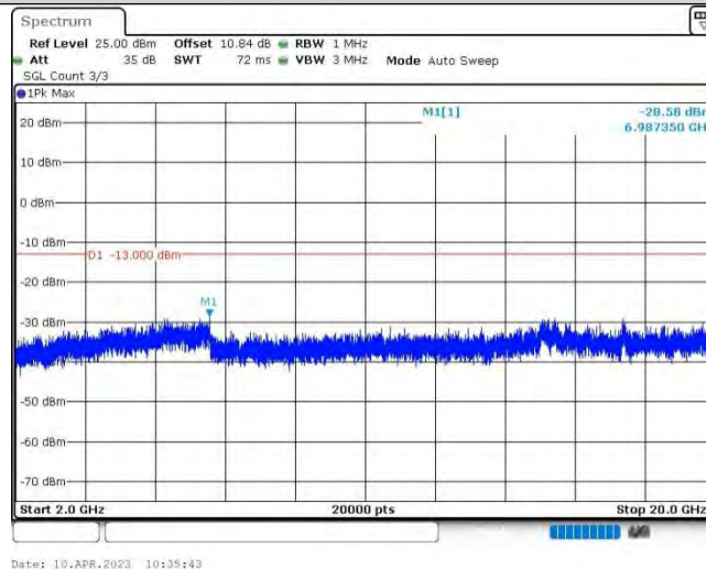
Band25-5MHz-16QAM-26665-1RB#0-Range3:2000~20000MHz
