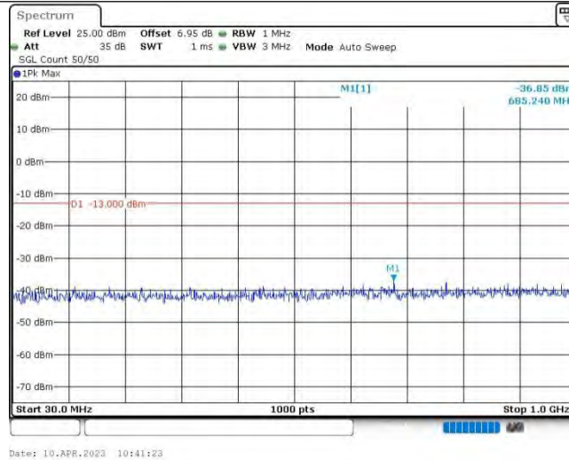
Band25-20MHz-QPSK-26140-1RB#0-Range1:30~1000MHz
