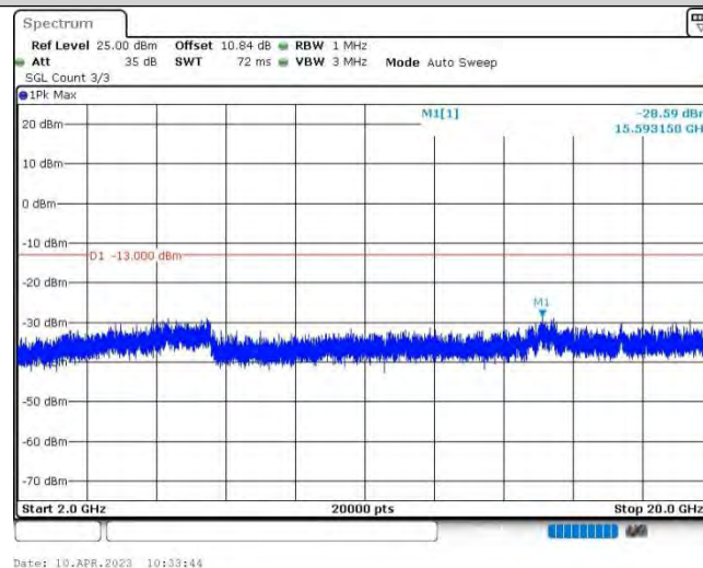
Band25-5MHz-QPSK-26065-1RB#0-Range3:2000~20000MHz
