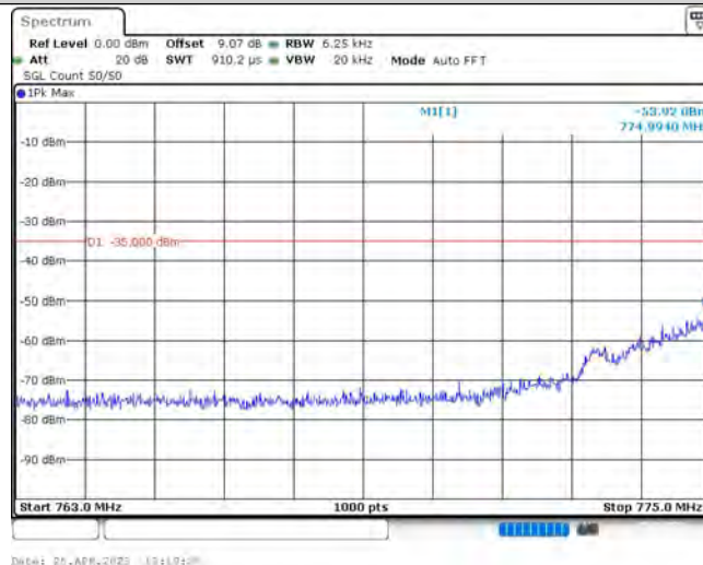
Band13-5MHz-QPSK-23205-1RB#0-Range1:763~775MHz
