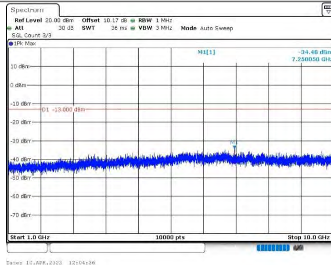
Band26@90-1.4MHz-16QAM-26915-1RB#0-Range2:1000~10000MHz
