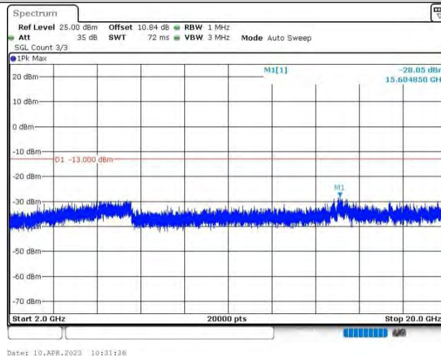
Band25-3MHz-16QAM-26055-1RB#0-Range3:2000~20000MHz
