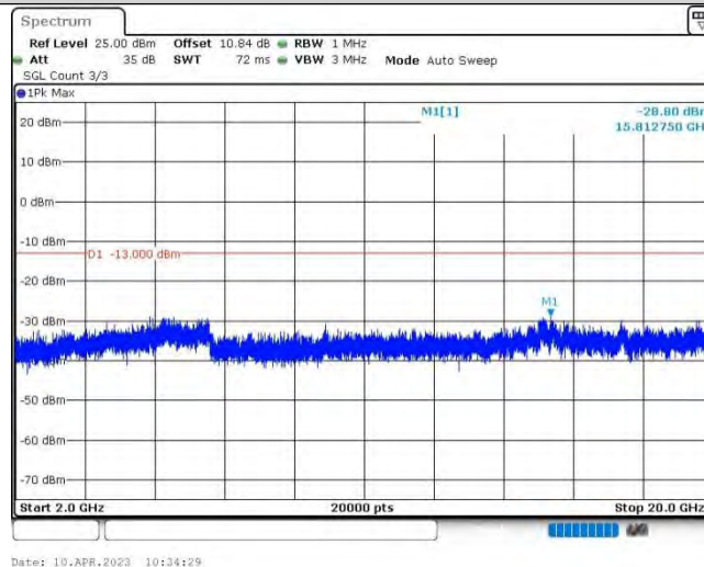
Band25-5MHz-QPSK-26365-1RB#0-Range3:2000~20000MHz
