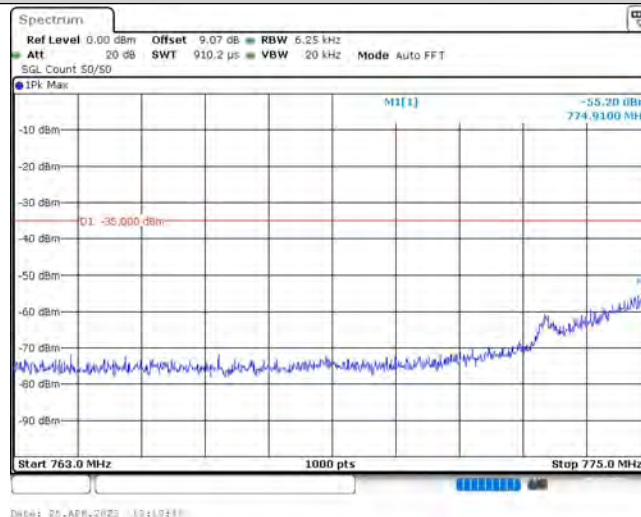
Band13-5MHz-16QAM-23205-1RB#0-Range1:763~775MHz
