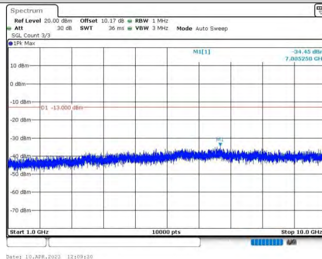
Band26@90-3MHz-16QAM-26915-1RB#0-Range2:1000~10000MHz
