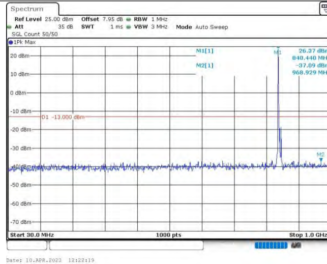
Band26@90-10MHz-16QAM-26990-1RB#0-Range1:30~1000MHz
