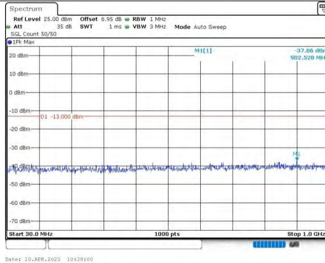
Band25-10MHz-16QAM-26640-1RB#0-Range1:30~1000MHz
