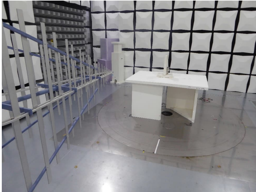
EUT Position 2 – standing Test setup semi-anechoic chamber M276 Preliminary and final measurment
