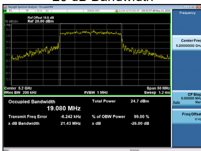
99 % Occupied Bandwidth
