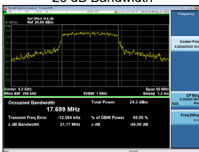
CH40 26 dB Bandwidth
