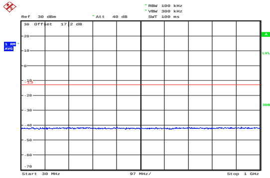
NB-IOT Band 2 CH-Low 30MHz-1GHz
