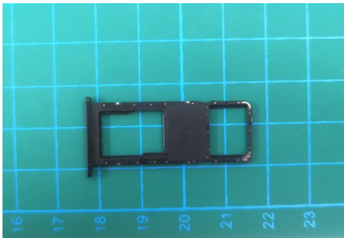
Single SIM tray for SM-A042F:
