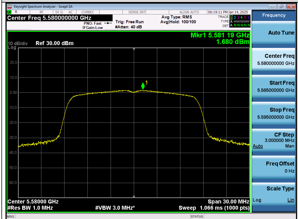
Test_Graph_802.11a_Chain A_5580_6Mbps_PSD
