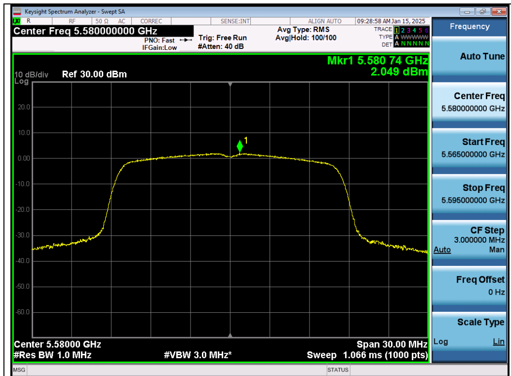
Test_Graph_802.11a_Chain B_5580_6Mbps_PSD
