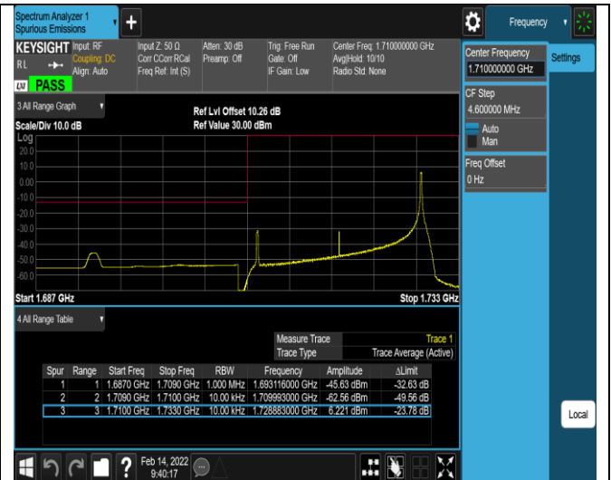
Band4-20MHz-16QAM-20300-1RB#0
