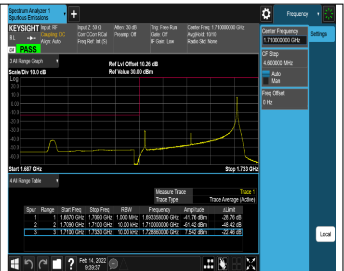
Band4-20MHz-QPSK-20300-1RB#0
