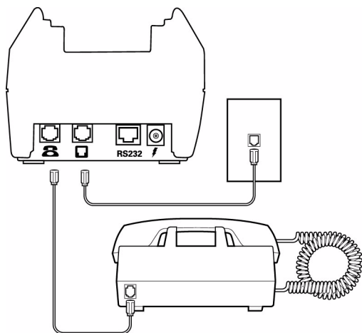
Figure 27 Pass-through Connection
