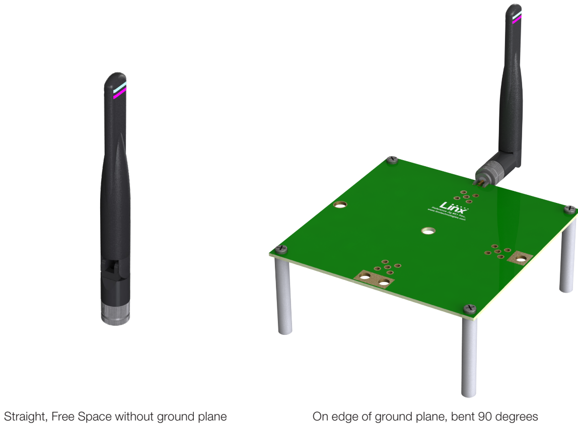
Figure 2. ANT-DB1-RAF Antenna Evaluation Orientations
